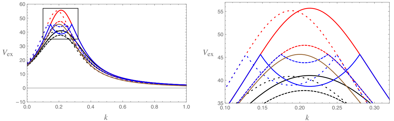
FIG. 7. Left panel: lines for z = -1 , p = 0.2 showing the exchange kernel V_{\text{ex}}^{\text{D}} with \lambda = 0.7 , as a function of k for W = 1.978 (black), W = 2.01 (long-dashed black) and W = 2.1 (short-dashed black), the singular kernel V_{\text{ex}}^{\text{B}} as a function of k for W = 1.978 (red), W = 2.01 (long-dashed red) and W = 2.1 (short-dashed red), and the regularized kernel V_{\text{ex}}^{\text{C}} as a function of k for W = 1.978 (blue), W = 2.01 (long-dashed blue) and W = 2.1 (short-dashed blue). The nonrelativistic limit, independent of energy, is shown for comparison (brown). The dimensionless units are defined in the text. Right panel: the same cases on the expanded scale shown in the box in the left panel.
