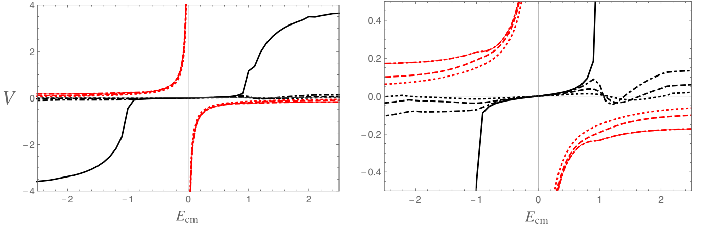
FIG. 15. The integrated kernels V = -16V_D^4/g^4 (black lines) and V = -16V_D^{2\times 2}/g^4 (red lines) for \lambda = 1 (dotted), 0.7 (dashed), 0.5 (dot-dashed) and 0.1 (solid) as a function of E_{\text{cm}} for the special case when p = p' = 0 and \mu = 1 . Left panel: large vertical scale. Right panel: small vertical scale. Note that, for -16V_D^{2\times 2}/g^4 , the cases \lambda = 0.1 and 0.5 overlap, appearing as a single line. Units for E_{\text{cm}} are the boson mass \mu .
