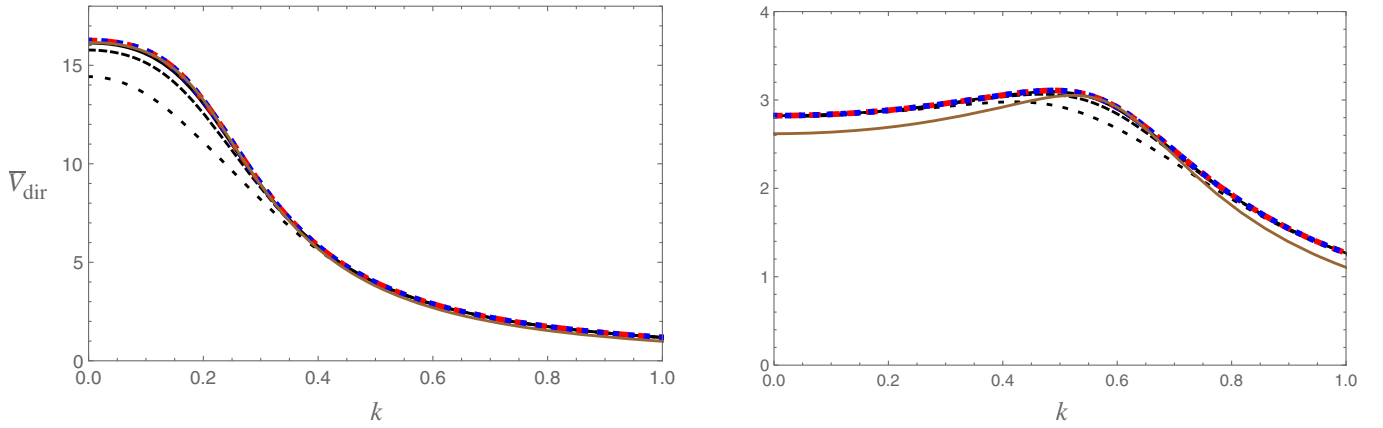
FIG. 9. Left panel: lines for integrated kernels at p = 0.2 showing the direct kernel \bar{V}_{\text{dir}}^{\text{D}} as a function of k for \lambda = 0.5 (black), 0.7 (long-dashed black) and \lambda = 1 (short-dashed black). The other cases, also for p = 0.2 , are the nonrelativistic limit (brown), \bar{V}_{\text{dir}}^{\text{B}} (red dashed), and \bar{V}_{\text{dir}}^{\text{C}} (blue dashed). The dimensionless units are defined in the text. Right panel: the same cases but for p = 0.6 .
