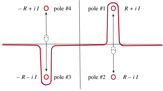
FIG. 13. Figure showing the migration of the four poles identified in Eq. (4.9) in the complex q_0 plane. Two double poles for I = 0 are shown as overlapping dashed circles; as I increases they migrate to the small red circles, and the contour (red line) is deformed to avoid them.
