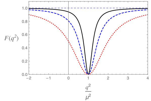
FIG. 5. Form factor (2.12) for \lambda = 0.5 (black), 0.7 (blue dashed), and 1 (red dotted).
