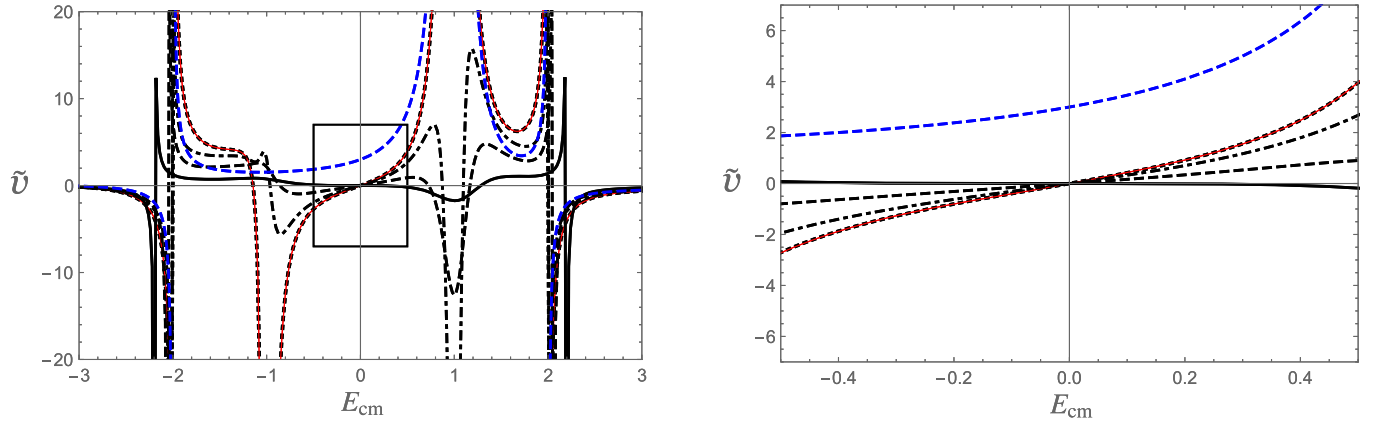
FIG. 14. Lines showing the integrands \tilde{v}_{\text{BS}}^4 (blue dashed), \tilde{v}_{\text{B}}^4 (thin red) and \tilde{v}_D^4 for \lambda = 0.1 (black dotted line overlapping the thin red line), 0.5 (black dot-dashed), 0.7 (black dashed), and 1 (black solid), all as a function of E_{\text{cm}} for the special case when \mu = 1 and p = p' = k = 0 . Left panel: expanded scale. Right panel: enlarged picture of the region in the square box in the left panel. Units for E_{\text{cm}} are the boson mass \mu .
