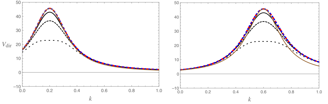
FIG. 6. Left panel: lines for z = 1 , p = 0.2 showing the direct kernel V_{\text{dir}}^{\text{D}} as a function of k for \lambda = 0.5 (black), \lambda = 0.7 (long-dashed black) and \lambda = 1 (short-dashed black). The other cases, also for z = 1 and p = 0.2 , are the nonrelativistic limit (brown), V_{\text{dir}}^{\text{B}} (red dashed), and V_{\text{dir}}^{\text{C}} (blue dashed). The dimensionless units are defined in the text. Right panel: the same cases but for p = 0.6 .
