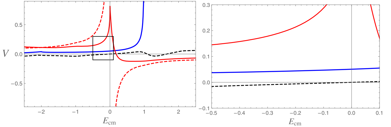
FIG. 16. Lines showing the integrated kernel V = -16V_{\text{BS}}^4/g^4 (blue), and for \lambda_\mu = 0.7 , the kernels V = -16V_D^4/g^4 (black dashed), V = -16(\Re V_D^{2\times 2})/g^4 (red), V = -16V_{D0}^{2\times 2}/g^4 (red, dashed). Left panel shows these on a large scale; right panel gives the details inside the box shown in the left panel. Units for E_{\text{cm}} are the boson mass \mu .
