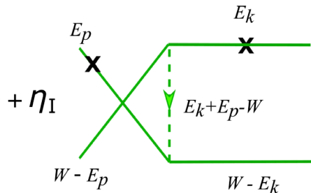
FIG. 3. OBE exchange diagram with particle 1 on shell in both the initial state and final states, and in this paper \eta_I = \eta = 1 .
