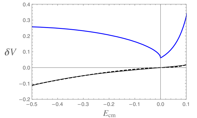
FIG. 17. Lines showing, for \lambda_\mu = 0.7 the ratio \delta V_{\text{BS}}^4 = V_{\text{BS}}^4/V_D^{2\times 2} (blue), and \delta V_D^4 = V_D^4/V_D^{2\times 2} (black dashed). The thin black line which fits \delta V_D^4 is discussed in the text. Units for E_{\text{cm}} are the boson mass \mu .
