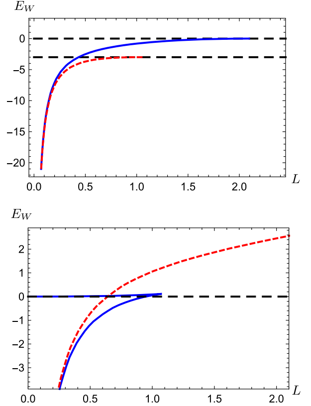
FIG. 9. Energy E_W as a function of the separation L , for supersymmetric solutions n = 2 , (\phi_2, \mathcal{A}_2) (top) and n = 4 , (\phi_4, \mathcal{A}_4) (bottom), and chosen to have \mathcal{A}_I = 0 . Continuous (blue) lines correspond to configurations with \theta = 0 , short-dashed (red) lines depict configurations with \theta = \pi/2 , and long-dashed (black) lines represent configurations reaching exactly the end of space.
