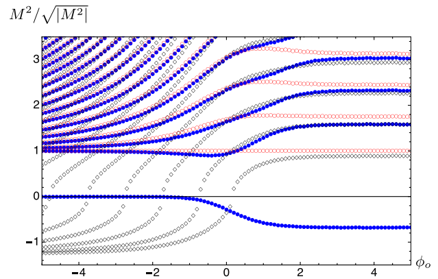
FIG. 5. Mass spectrum of the fluctuations of the negative DW solutions. The (red) circles are spin-two states, the (blue) disks are spin-zero states, and the (black) diamonds represent the probe approximation calculation of the same spin-zero masses. The masses M are normalized to the lightest spin-two state, and plotted as a function of \phi_o , defined in Eqs. (43) and (44). For \phi_o \rightarrow -\infty the backgrounds approach the supersymmetric solution in Eqs. (A3) and (A4)—or Eqs. (A7) and (A8). The numerical calculations are performed with finite cutoffs \rho_1 = 10^{-6} and \rho_2 = 8 . We checked explicitly that these choices are close enough to the physical limits \rho_1 \rightarrow \rho_o = 0 and \rho_2 \rightarrow +\infty that the numerical results do not display important residual spurious dependence on the cutoffs.
