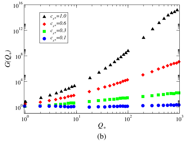
FIG. 1. The growing function G(Q_*) as defined by Eq. (4.1). (a) Linear in T dissipation coefficient (b) Cubic in T dissipation coefficient.
