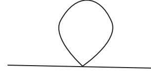
FIG. 1. Tadpole one-loop contribution to the propagator in \phi^4 theory.
