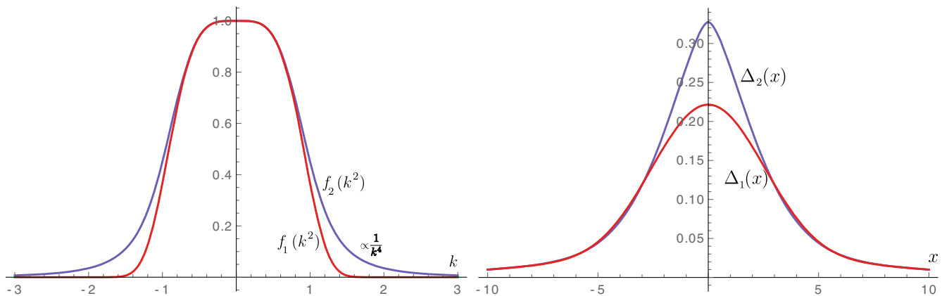
FIG. 6. The left plot represents the functions f_1(k), f_2(k) and the right plot shows their Fourier images \Delta_{1,2}(x) .
