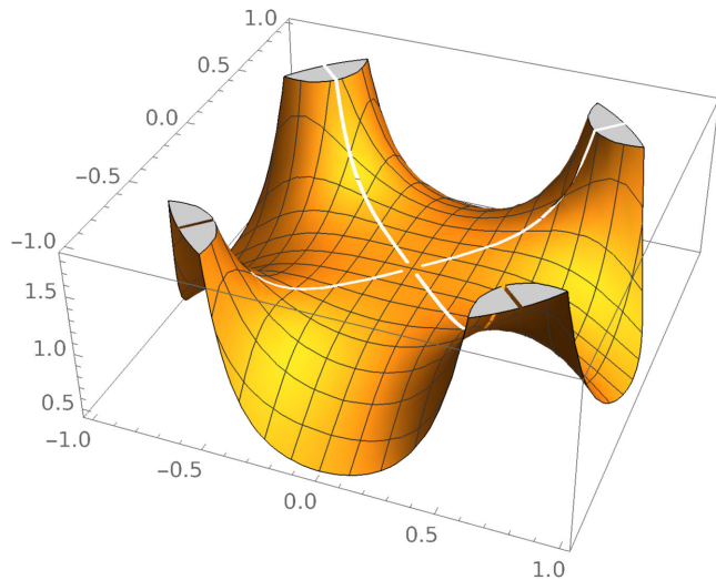
FIG. 5. Absolute value of the function f_2(\text{Re } k, \text{Im } k) .
