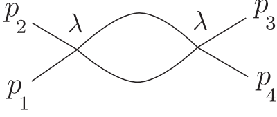
FIG. 2. One-loop contribution to 2 \rightarrow 2 scattering in \phi^4 theory. Here only the s -channel contribution is shown, p = p_1 + p_2 .
