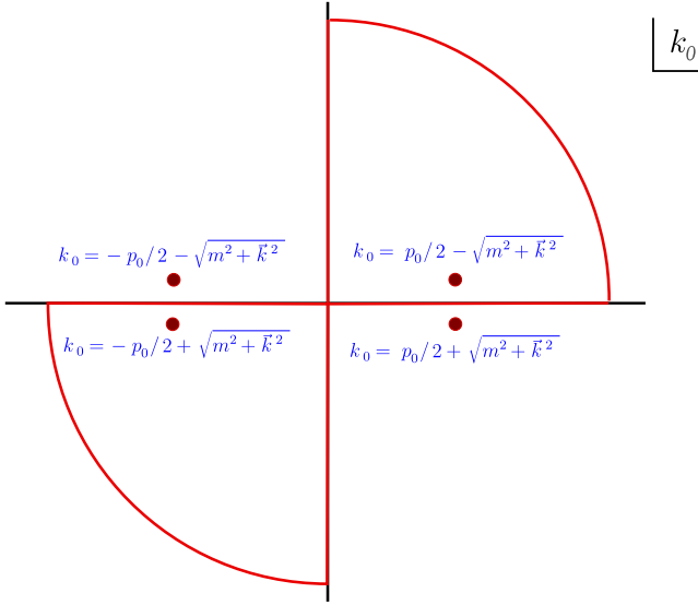
FIG. 3. Poles of the amplitude (20).
