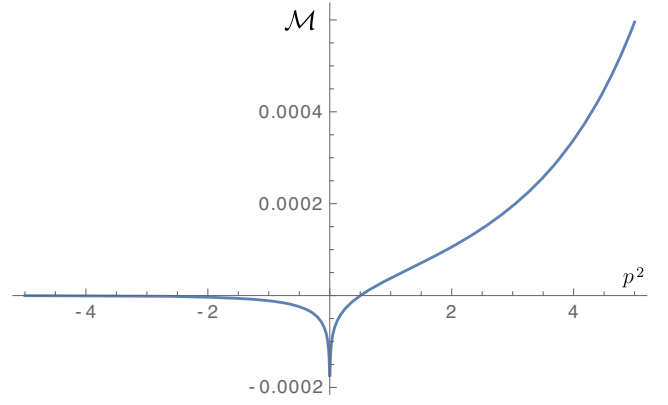
FIG. 4. Amplitude (real part) dependence on the external momentum. Here \alpha = 1 , m = 0 , \lambda = 0.1 .
