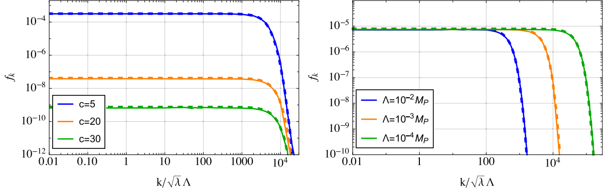
FIG. 2. Particle number spectra for \chi -particles with a mass with a single pole. Solid lines correspond to the full numerical solution, dashed lines to the semiclassical approximation. The initial amplitude is \Phi = 2\sqrt{M_P\Lambda} . Left: \Lambda = 10^{-3}M_P , \tilde{c} = 0.05 and c = 5, 20, 30 , (blue, orange, green, respectively). Right: c = 10 , \tilde{c} = 0.05 and \Lambda = 10^{-2}M_P, 10^{-3}M_P, 10^{-4}M_P , (blue, orange, green, respectively).
