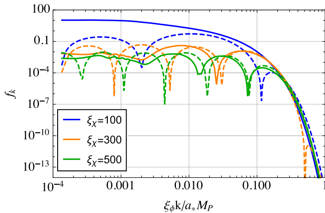
FIG. 6. Particle number and energy density for Higgs inflation. Solid lines show the numerical solution of the mode equation and the dashed lines the results from the semiclassical approximation. Left: particle number density for Higgs inflation with \xi_\phi = 100 and \xi_\chi = 100, 300, 500 (blue, orange, green, respectively). Right: energy density for Higgs inflation with \xi_\phi = 10^2, 10^3, 10^4 (blue, orange, green, respectively) and \xi_\chi = \xi_\phi .
