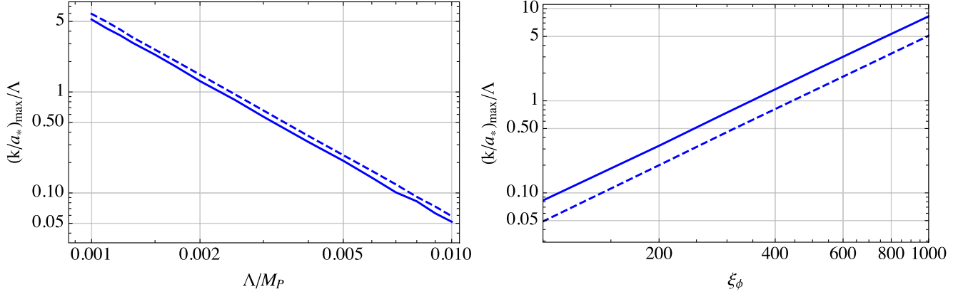
FIG. 5. Ratio of (k/a_*)_{\max} to the unitarity cutoff scale for running kinetic inflation, with c_K = 1 and c_V = 0.1 , (left) and Higgs inflation, with \xi_\phi = \xi_\chi , (right) (with \Lambda = M_P/\xi_\phi ). The solid line shows the numerical result and the dashed line the semiclassical approximation.
