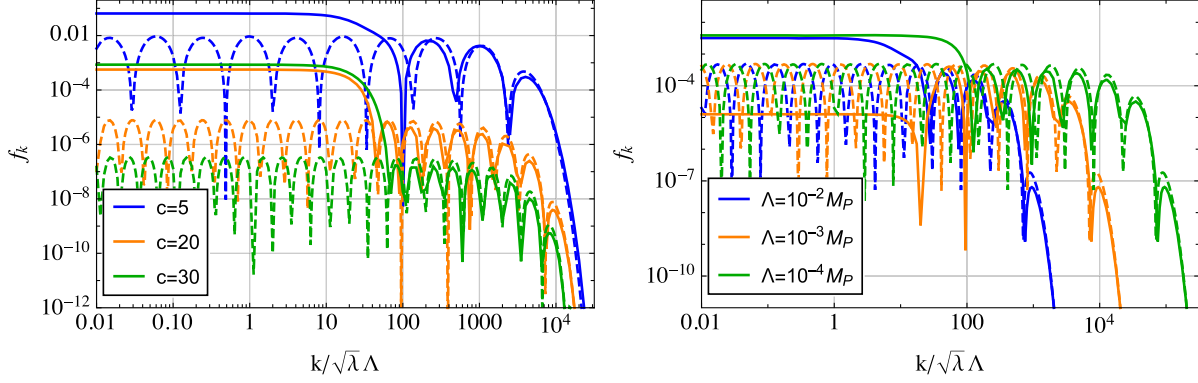
FIG. 3. Particle number spectra for \chi -particles with a mass with a double pole. Solid lines correspond to the full numerical solution, dashed lines to the semiclassical approximation. The initial amplitude is \Phi = 2\sqrt{M_P\Lambda} and the numerical spectra are evaluated at \phi = \phi_* . Left: \Lambda = 10^{-3}M_P , \tilde{c} = 0.05 and c = 5, 20, 30 , (blue, orange, green, respectively). Right: c = 10 , \tilde{c} = 0.05 and \Lambda = 10^{-2}M_P, 10^{-3}M_P, 10^{-4}M_P , (blue, orange, green, respectively).
