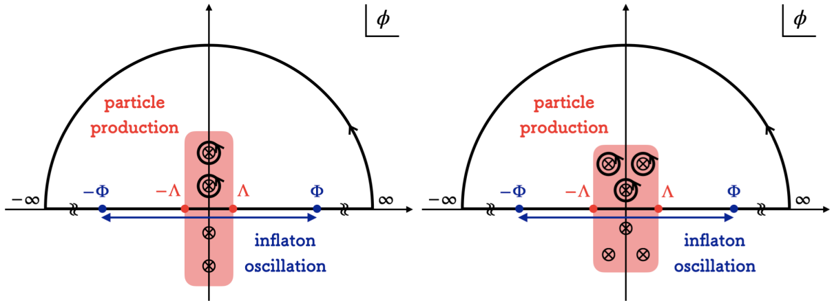
FIG. 1. Integration contours in the complex \phi -plane, for two different types of pole structure, corresponding to the two examples in Sec. II D. The extension of the integration range from [-\Phi, \Phi] to [-\infty, \infty] is justified when the particle production dominantly occurs only around the origin |\phi| \lesssim \Lambda (\ll \Phi) . The extended integration contour can then be closed at complex infinity, reducing the integral to the sum of the residues at the poles.
