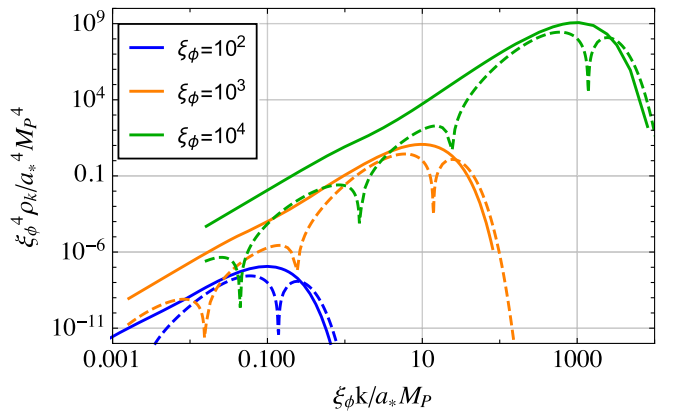
FIG. 6. Particle number and energy density for Higgs inflation. Solid lines show the numerical solution of the mode equation and the dashed lines the results from the semiclassical approximation. Left: particle number density for Higgs inflation with \xi_\phi = 100 and \xi_\chi = 100, 300, 500 (blue, orange, green, respectively). Right: energy density for Higgs inflation with \xi_\phi = 10^2, 10^3, 10^4 (blue, orange, green, respectively) and \xi_\chi = \xi_\phi .
