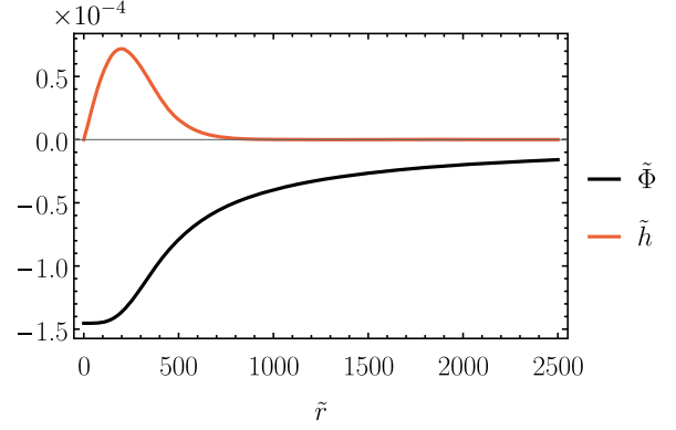
FIG. 1. The spherical hedgehog solution, \mathcal{A}^i = (\mathcal{A}^r, \mathcal{A}^\theta, \mathcal{A}^\varphi) = (h(|\mathbf{x}|)e^{-imE_h t}, 0, 0) , given in terms of the rescaled quantities from Eq. (28). The solution is normalized so that \int \tilde{h}^2(\tilde{r}) 4\pi \tilde{r}^2 d\tilde{r} = 1 .
