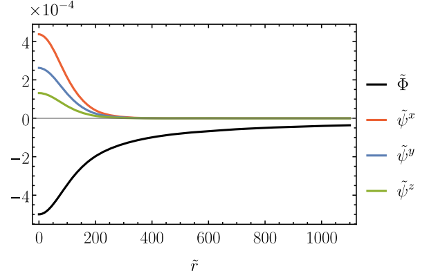
FIG. 5. The ground-state solution for the ansatz in Eq. (A21) with \tilde{M}^{(x)} = 0.690 , \tilde{M}^{(y)} = 0.248 . Note that \sum_j \tilde{M}^{(j)} = 1 . The \tilde{\Phi}(\tilde{r}) and \sqrt{\sum_j \tilde{\psi}^{j2}(\tilde{r})} are identical to the blue and orange curves in Fig. 3, respectively. Since the data in Fig. 3 are equivalent to, e.g., \tilde{M}^{(x)} = 1 , one concludes that the gravitational properties of the ground-state VDM halos, i.e., the gravitational potential, \tilde{\Phi}(\tilde{r}) , and energy density, \sum_j \tilde{\psi}^{j2}(\tilde{r}) , are independent of the \tilde{M}^{(j)} values.
