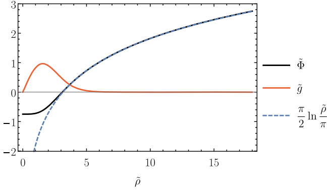
FIG. 2. The hedgehog cylindrical solution, \mathcal{A}^j = (\mathcal{A}^\rho, \mathcal{A}^\theta, \mathcal{A}^z) = (g(\rho)e^{-imE_\rho t}, 0, 0) , given in terms of the rescaled quantities from Eq. (28). The solution is normalized so that \tilde{g}'(\tilde{\rho} = 0) = 1 .
