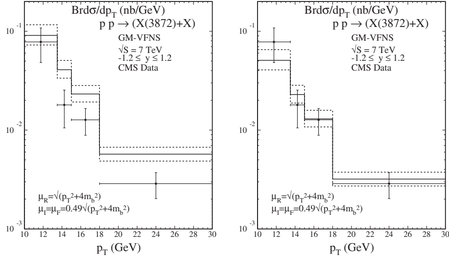
FIG. 3. Differential cross sections times branching fractions for X(3872) nonprompt hadroproduction at \sqrt{S} = 7 TeV, integrated over y in the region |y| \leq 1.2 , as a function of p_T . The solid points with error bars are extracted from the CMS data [11]. The solid and the upper and lower dashed histograms represent our NLO GM-VFNS predictions for \xi = 1, 0.5, 2 , respectively. The theoretical predictions were evaluated using the R_B values in (a) Eq. (3) (left) and (b) Eq. (5) (right).
