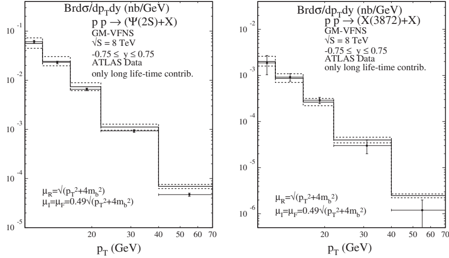
FIG. 1. Double differential cross sections times branching fractions for (a) \psi(2S) (left) and (b) X(3872) (right) nonprompt hadroproduction at \sqrt{S} = 8 TeV, averaged over y in the region |y| \leq 0.75 , as a function of p_T . The solid points with error bars represent the ATLAS data [12]. The solid and the upper and lower dashed histograms represent our NLO GM-VFNS predictions for \xi = 1, 0.5, 2 , respectively.
