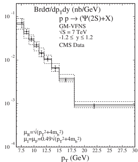
FIG. 2. Double differential cross section times branching fraction for \psi(2S) nonprompt hadroproduction at \sqrt{S} = 7 TeV, averaged over y in the region |y| \leq 1.2 , as a function of p_T . The solid points with error bars represent the CMS data [5]. The solid and the upper and lower dashed histograms represent our NLO GM-VFNS predictions for \xi = 1, 0.5, 2 , respectively.
