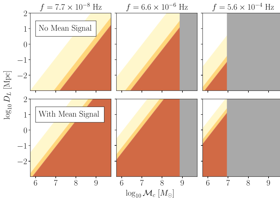
FIG. 4. Detection sensitivity of the Roman EML Survey in \log_{10}\mathcal{M}_c - \log_{10}D_L space at multiple fixed frequency. Colors indicate detection thresholds at different confidence levels. Top row: sensitivity when signals are mean subtracted. Bottom row: Sensitivity when the full signal is observable. For the three columns, the GW frequencies are fixed to be 7.7 \times 10^{-8} Hz, 6.6 \times 10^{-6} Hz, and 5.6 \times 10^{-4} Hz, respectively. In all panels, GW sources that reach the ISCO at the specified frequency or lower are blocked out in gray.
