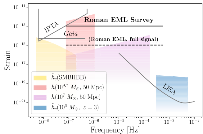
FIG. 3. Strain sensitivity of various GW detectors and corresponding example signals. Note that the sensitivity for different detectors is not represented by the same quantity, in anticipation of the signal source types. The sensitivity for LISA and IPTA is represented by the dimensionless characteristic noise strain from the detector noise power spectral density, given by \tilde{h}_n(f) = \sqrt{fS_n(f)} . In the frequency range of IPTA, the yellow block shows the expected \tilde{h}_c of the SMBHBB. In the frequency range of LISA, the blue block shows the characteristic strain, \tilde{h}_c(f) \equiv 2f\tilde{h}(f) , of a fast-evolving 10^6 M_\odot binary at D_L = 25 Gpc. The sensitivity of Gaia and Roman EML Survey is represented by the detectable instantaneous (time-domain) strain, h , of monochromatic GWs, assuming end-of-survey performance. For Roman EML Survey, the solid line shows the sensitivity under signal mean subtraction, and the dashed line shows the sensitivity if full astrometric deflections are detectable. The red and violet block show the time-domain wave amplitude of monochromatic GWs with chirp masses 10^{9.7} M_\odot and 10^7 M_\odot . The shown frequency range of these GWs are limited by the mission lifetime of Roman EML survey and f_{\text{ISCO}} at this chirp mass. Note that the example signals of Roman EML and LISA are illustrative; they do not reflect the GW source population expected from binary black hole formation theory. As is shown, the frequency band from roughly 5 \times 10^{-7} Hz to 1 \times 10^{-5} Hz is uniquely accessed by Roman EML survey.
