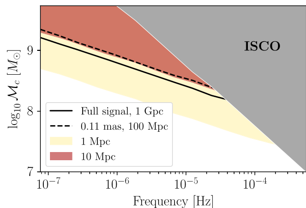
FIG. 5. Sensitivity of the Roman EML Survey to \log_{10}\mathcal{M}_c . The upper right corner (shaded gray) excludes massive systems that reach the ISCO at each frequency or lower. Detection sensitivity threshold is represented by the detectable chirp mass at a 2\sigma confidence level at various luminosity distances. Yellow and red blocks show detectable mass ranges at 1 Mpc and 10 Mpc, respectively, assuming the mean astrometric deflection is subtracted from the signal. The dashed line shows the detection threshold at 100 Mpc if the astrometric accuracy were to improve to 0.11 mas, equivalent to a factor of 10 improvement in the sensitivity. The solid line shows the sensitivity at 1 Gpc if the mean signal were observable, roughly comparable to a factor of 100 sensitivity improvement. See Sec. IV for further discussions.
