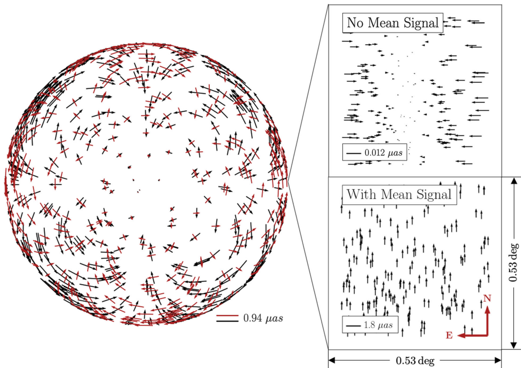
FIG. 1. The expected stellar astrometric deflections. Left: Orthographically projected dn for a subset of stars observed by Gaia in the Northern Hemisphere onto the galactic plane (inspired by a very similar plot in [24]). The North Galactic pole is at the center, which is also the position of the GW source. Black arrows correspond to the real part of the waveform at GW phase \phi = 0 (plus polarization), and the red arrows correspond to that at \phi = \pi/4 (cross polarization). The source is a 10^9 M_\odot equal-mass binary black hole at 1 Mpc at (l = 90 \text{ deg}, b = 90 \text{ deg}) in galactic coordinates, emitting GWs at 10^{-6} Hz. This inclination angle is set to i = 0 (i.e., face-on) and the polarization angle is \psi = 0 . Right: Deflections within the Roman Space Telescope's FoV during the EML survey. The lower panel shows the total deflection, and the upper panel shows the deflection after subtracting the mean, since the mean is expected to be absorbed in the pointing reconstruction; for further discussion see Sec. IV. Star coordinates are selected from the Gaia Data Release 2 catalog, with brightness 0 < G < 9 [32,33]. Density of stars reflects only a subset of the true stellar density in the catalog.
