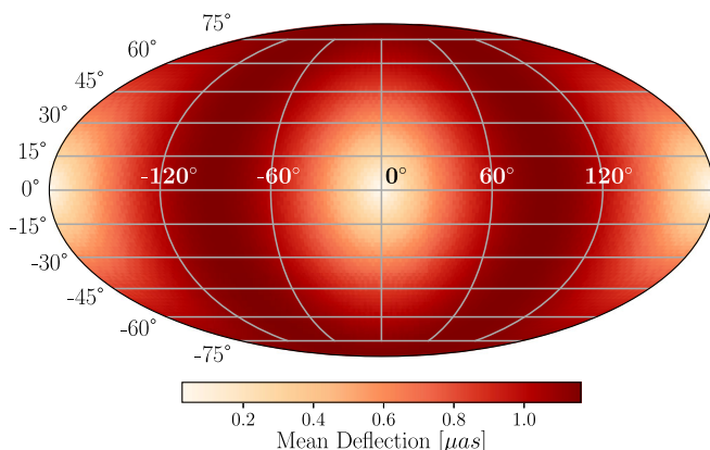
FIG. 2. Mean maximal deflection due to GW sources at different Galactic coordinates. The FoV is fixed to point toward the Galactic center, i.e., l = 0 deg, b = 0 deg. The magnitude is calculated as that of the orthographic projection of dn in the FoV, averaged over all observed stars. The maximum occurs when the source position vector is perpendicular to the star position vectors, which is consistent with Eq. (5). Aside from its coordinates, the GW source at each position has the same properties as that in Fig. 1. In combination with Fig. 1, we observe that the quadrupolar deflection pattern does not show up when we consider signal magnitude only.
