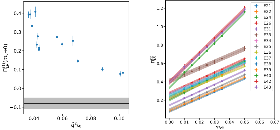
FIG. 4. Left: \Pi^{(1)} in the chiral-valence limit am_v \rightarrow 0 plotted against \hat{q}^2 t_0 for all 15 ensembles. The horizontal grey band shows the contribution 8L_{10} to \Pi^{(1)}(q) , where for simplicity we combined the statistical and systematic errors of our final result in quadrature [see Eq. (3.2)]. Right: the linear fits of \Pi^{(1)} in each ensemble that give the limits shown on the left. Ensemble numbers are as in Ref. [11].
