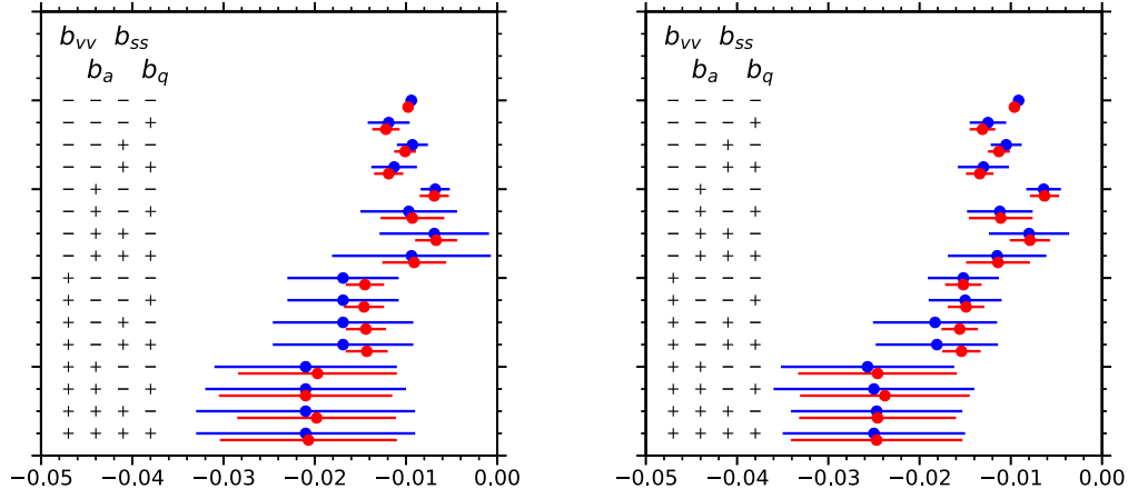
FIG. 3. Results for L_{10} , using only the smallest valence mass am_v = 0.01 , for all combinations of the four NNLO parameters and \Delta_{\text{mix}} (see Appendix C 1). Left panel: fits of \Pi^{(1)} . Right panel: fits of \Pi^{(1-0)} . The columns with +/- signs indicate which NNLO parameters are present/absent in each fit. Fit results with \Delta_{\text{mix}} free are shown in blue, and fits with \Delta_{\text{mix}} = 0 in red. The topmost pair of points in each plot represents the NLO fit.
