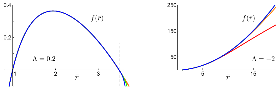
FIG. 4. The function f(\bar{r}) of the standard metric form (8) related to the solution (90), (91) via the transformation (11). The positive \Lambda case (left) indicates the presence of the cosmological horizon at the boundary of the convergence interval (the dashed line). For negative \Lambda (right), the series converges in the whole plotted range, corresponding to a static region everywhere above the black-hole horizon. Here we use the same values of parameters as in Figs. 2, 3.
