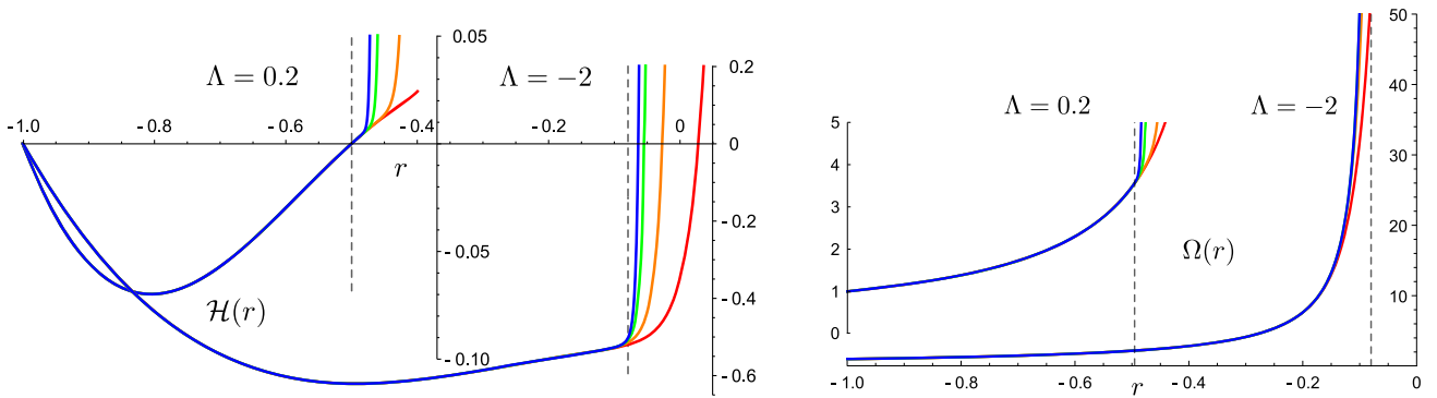
FIG. 3. The functions \mathcal{H}(r) given by (91) (left) and \Omega(r) given by (90) (right) for two values of the cosmological constant \Lambda (with the same parameters as in Fig. 2). The black-hole horizon r_h = -1 is located at the center of the radius of convergence. Here we plot the functions \mathcal{H}(r) in the regions outside the black-hole horizon up to the outer radii of convergence indicated by dashed vertical lines. For \Lambda > 0 , the function \mathcal{H}(r) seems to have another root corresponding to the cosmological horizon, while for \Lambda < 0 , it remains nonvanishing. First 50 (red), 100 (orange), 200 (green), 300 (blue) terms in the expansions are used. The results fully agree with the numerical solutions up to the dashed lines, where such simulations also fail. The function \Omega(r) grows monotonously.
