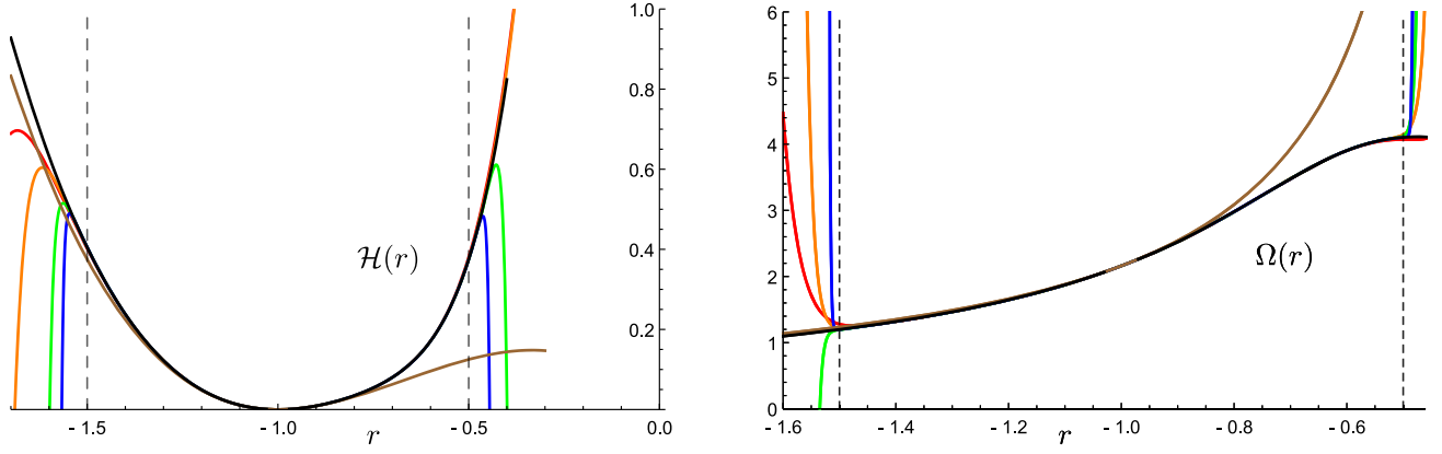
FIG. 7. The metric functions \mathcal{H}(r) (left) and \Omega(r) (right) for the extreme higher-order (discrete) Schwarzschild-Bach-de Sitter solution [0, 2] with L = 2 , k = -1/2 , \Lambda = 3/14 , c_1 = -1 , \tilde{b}_2 = 1 , r_0 = -1 and a_0 = 1/\sqrt{\Lambda} . First 10 (red), 20 (orange), 50 (green), and 100 (blue) terms in the expansions are used. Furthermore, the corresponding Schwarzschild-de Sitter solution obtained by setting \tilde{b}_2 = 0 is shown (brown). A numerical solution with initial values taken from the first 100 terms of the metric functions at r = -1.15 and r = -0.85 is also given (black). The numerics breaks down on the extreme horizon. Vertical dashed lines indicate the radius of the convergence obtained using the same method as in Fig. 3.
