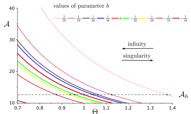
FIG. 6. Relation between the sphere area \mathcal{A} (of constant r ) and the corresponding value of the expansion \Theta of the privileged null vector field \mathbf{k} = \partial_r , for different values of the Bach parameter b . The dashed line indicates the horizon area \mathcal{A}_h which is b independent. Here r_h = -1, k = 0.5, \Lambda = 0.2 .
