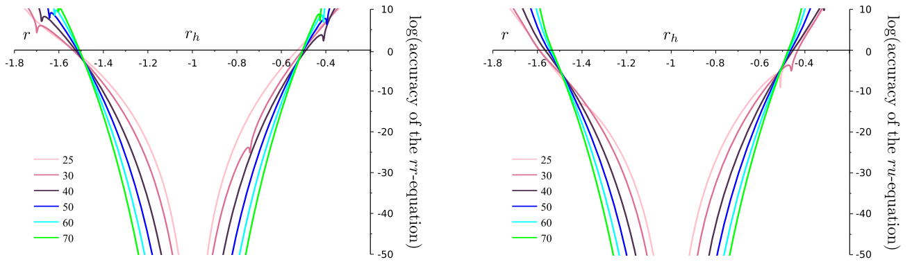
FIG. 1. The difference between the left- and right-hand side of the field equation (25) (left) and (26) (right) for the metric functions \Omega and \mathcal{H} given by (90), (91). The plotted values approach zero in a certain range of the radial coordinate r around the horizon r_h with the growing order n . This indicates that the equations are satisfied with a reasonable precision, depending on the finite order of the polynomial approximation in some convergence radius. Here we set r_h = -1, k = 0.5, b = 0.3 , and \Lambda = 0.2 .
