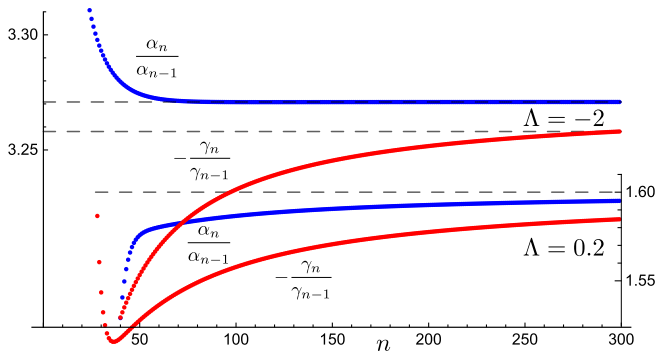
FIG. 2. The convergence radius for the power series (90) and (91) representing the metric functions \Omega and \mathcal{H} can be estimated using the d’Alembert ratio test demonstrating the asymptotic behavior similar to the geometric series. Here we assume r_h = -1, k = 0.5 with b = 0.3, \Lambda = 0.2 (bottom) and b = 0.2, \Lambda = -2 (top).
