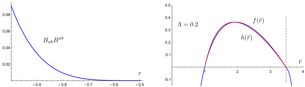
FIG. 5. The Bach invariant (19) as a function of the Kundt coordinate r (left), and the metric functions f(\bar{r}) and h(\bar{r}) of standard line element (8) corresponding to the solution (90), (91) via (11) (right), with the same parameters as in Figs. 2, 3 for \Lambda = 0.2 .
