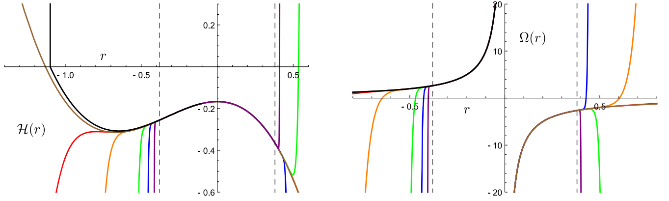
FIG. 8. The metric functions \mathcal{H}(r) (left) and \Omega(r) (right) for the non-Schwarzschild (Bachian) solution [-1, 0] with the parameters L = 0 , k = 1/2 , \Lambda = -1/2 , r_0 = 0 , a_0 = -1 , c_3 = -1 and b_0 \equiv c_4 = 1/20 . First 10 (red), 20 (orange), 50 (green), 100 (blue), and 300 (purple) terms in the expansions have been used. Furthermore, we plot the corresponding Schwarzschild-AdS solution obtained by setting b_0 \equiv c_4 = 0 (brown). A numerical solution with initial values taken from the first 100 terms of the metric functions at r = -0.2 is also plotted (black). Note that the numerics breaks down on the horizon given by \mathcal{H} = 0 . Vertical dashed lines indicate the radius of the convergence. From the behavior of the metric function \Omega we can read off that, in the standard spherical coordinates \bar{r} , the metric functions converge from \bar{r} \gtrsim 2.63 . (In contrast with the [0, 1] case, the series in the [-1, 0] class do not approach geometric series asymptotically. Thus we have estimated the radius of convergence by searching for which values of r these series can be bounded by appropriately chosen geometric series.) All the plotted functions visually overlap within the radius of convergence, validating the results.
