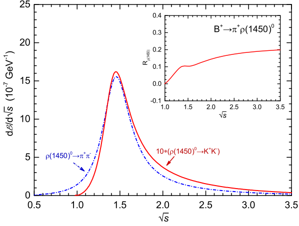
FIG. 3. The differential branching fractions for the decays B^+ \rightarrow \pi^+[\rho(1450)^0 \rightarrow K^+K^-] (solid line), which is magnified by a factor of 10, and B^+ \rightarrow \pi^+[\rho(1450)^0 \rightarrow \pi^+\pi^-] (dash-dot line) in the large diagram and curve for the \sqrt{s} dependent ratio R_{\rho(1450)} in the inset.
