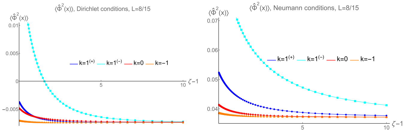
FIG. 6. VP for topological black holes with adS radius of curvature L = 8/15 \approx 0.53 and surface gravity \kappa = 115/32 \approx 3.59 , with Dirichlet (left) and Neumann (right) boundary conditions applied.
