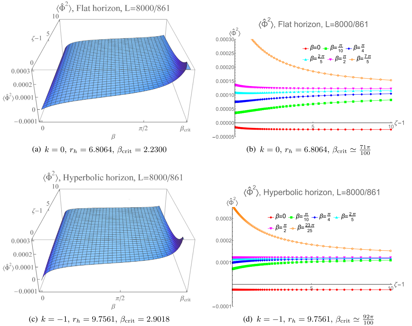
FIG. 5. VP for topological black holes with adS radius of curvature L = 8000/861 \approx 9.29 and surface gravity \kappa = 37843/320000 \approx 0.12 . Left: surface plots of VP as a function of the dimensionless radial coordinate \zeta (2.8), and parameter \beta for \beta \in [0, \beta_{\text{crit}}) . Right: line plots of VP as a function of \zeta for a selection of values of \beta .
