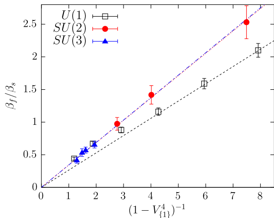
FIG. 5. \beta_f/\beta_s as a function of (1 - V_{\{1\}}^4)^{-1} .
