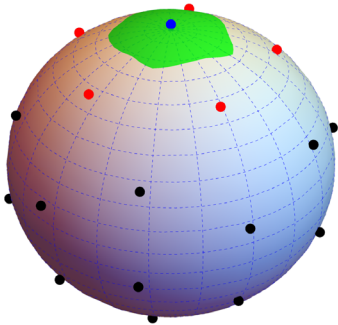
FIG. 1. A schematic demonstration of \Omega (in green) of G (a sphere) around \mathbb{1} (blue point) of the discrete group (shown as points). \mathcal{N} for H are given by red points. We have applied the S^2 metric to obtain the \Omega . In groups representable in two dimensions, this region resembles a polygon while in higher dimensions, it becomes a polytope.
