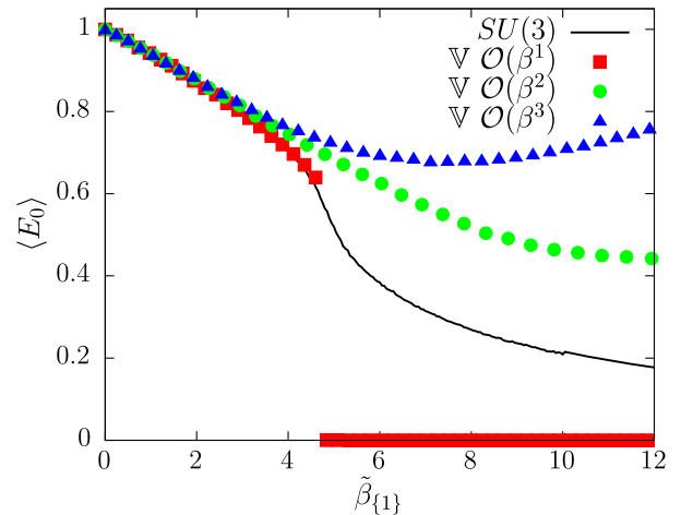
FIG. 3. Average energy per plaquette, \langle E_0 \rangle = 1 - \text{Re}\langle \text{Tr}U_p \rangle / 3 , vs \tilde{\beta}_{\{1\}} on 4^4 lattice for \mathbb{V} action with corrections of: (■) \mathcal{O}(\beta^1) , (●) \mathcal{O}(\beta^2) , and (▲) \mathcal{O}(\beta^3) . The black line is the SU(3) result.
