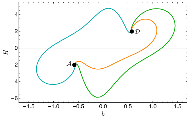
FIG. 2. This plot shows numerically integrated branches of solutions to the autonomous equations (42) for the + sign choice and choosing g_b = 1 , \Gamma = 2 ( \gamma = \frac{1}{4} ) and M_{\text{pl}} = 1 . The initial values of all three branches were chosen in the vicinity of the repeller \{b_c, H_c\} = \{-\frac{1}{\sqrt{3}}, -2\} ( A ). All branches then evolve in distinct trajectories in the phase plane towards the stable de Sitter attractor at \{b_c, H_c\} = \{\frac{1}{\sqrt{3}}, 2\} ( D ). This represents a numerical check of the phase portrait consideration.
