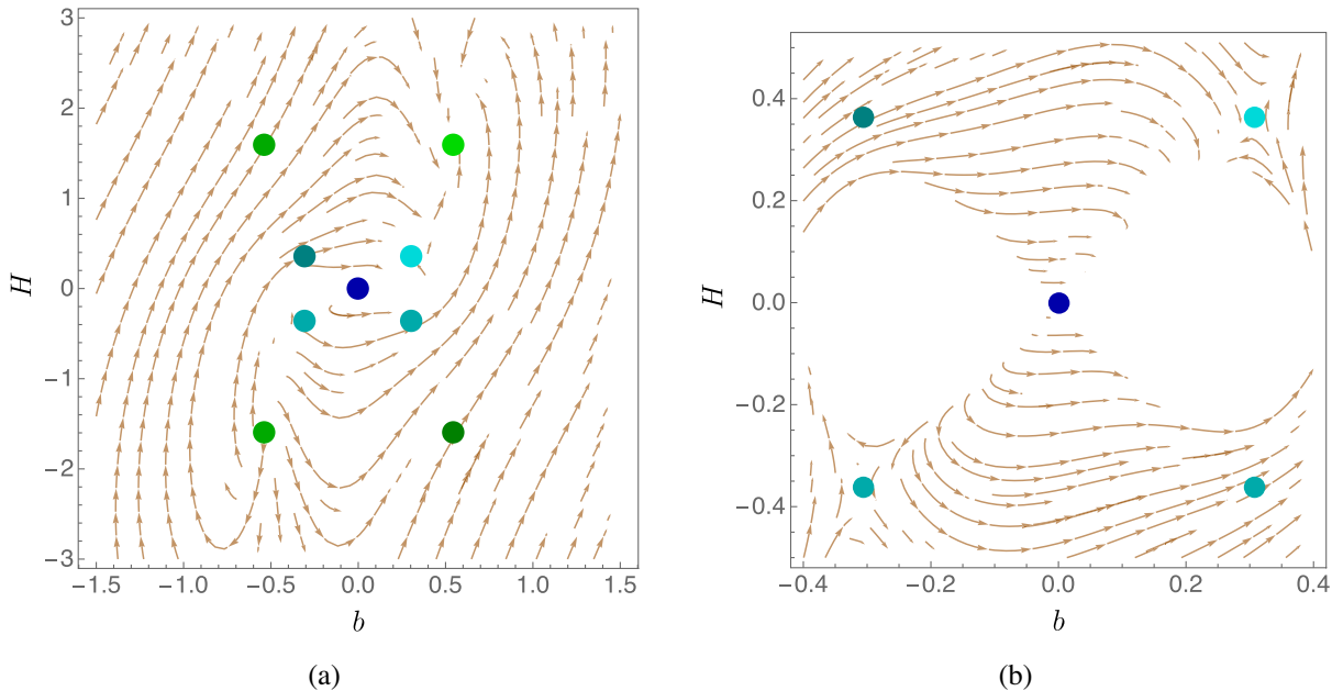
FIG. 3. These plots show the dynamical phase portrait of the autonomous system of equations (42) for the + sign choice in Eq. (43) and an interacting potential with an additional mass term V[x] = \frac{1}{4}m^2x - g_b x^2 , with choices m = 2 , g_b = 1 , \Gamma = 2 ( \gamma = \frac{1}{4} ) and M_{\text{pl}} = 1 in the phase plane \{b, H\} . The colored dots represent the nine critical points. This shows that additional terms in the choice of the potential have direct implications on the numbers of critical points and the shape of the solution space. (a) The overall picture far away from the central trivial critical point essentially remains the same and still admits stable as well as unstable critical de Sitter points. (b) An enlarged section of the phase portrait around the trivial critical point shows the direct effect of the additional mass term.
