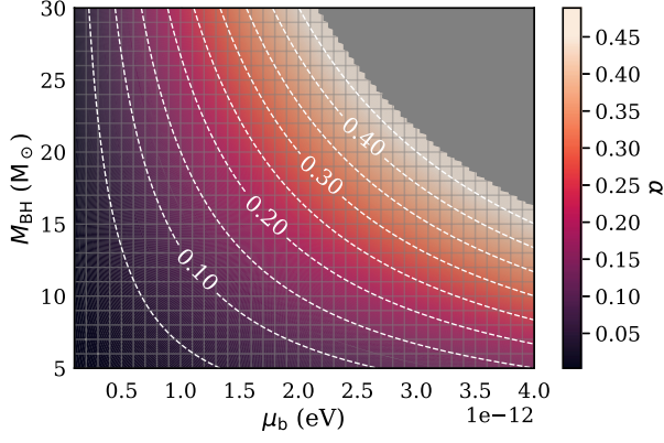
FIG. 1. Gravitational fine structure constant \alpha \equiv GM_{\text{BH}}\mu_b/(\hbar c) . Given the superradiance condition, the (n, \ell, m) = (0, 1, 1) bound state cannot form for \alpha \geq 0.5 , which is shown in gray.
