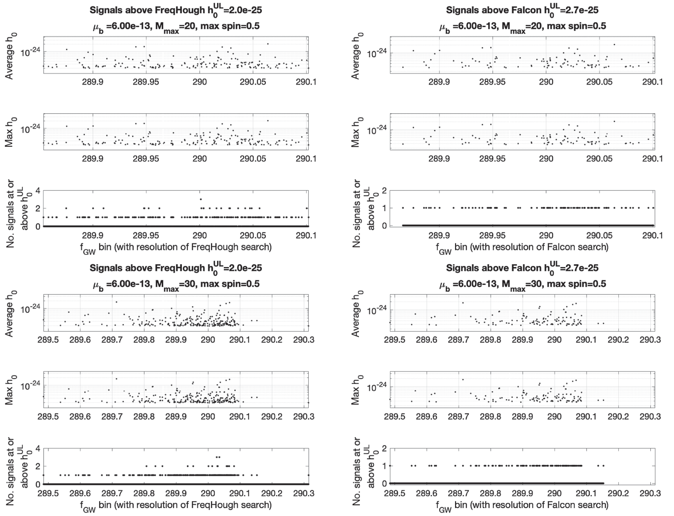
FIG. 39. The x axes show the signal frequency binned with the resolution of the two searches: (left panels) Freq Hough, 2.4 \times 10^{-4} Hz [22] and (right panels) Falcon, 1.7 \times 10^{-5} Hz [20,21]. From the bottom panel up, the y axis shows the number of detectable signals in each bin, their maximum intrinsic amplitude, and their average amplitude.
