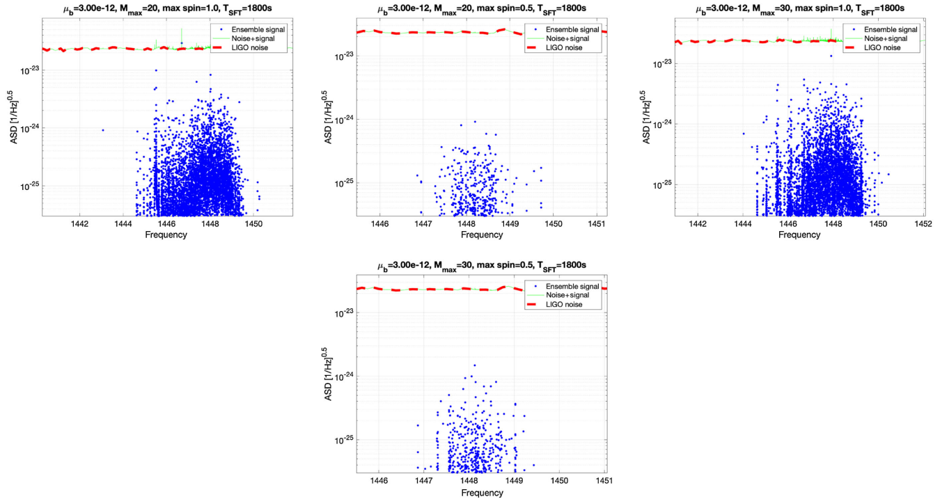
FIG. 47. The amplitude spectral density of the LIGO O2 data alone (dashed red line) and of an ensemble signal (top green points) assuming that \mu_b = 3 \times 10^{-12} eV and a Galactic black hole population with maximum mass 20M_\odot or 30M_\odot and maximum initial spins of 0.5 and 1. The time baseline assumed is 1800 s, close to what is used by the Freq Hough search in this frequency range [22].
