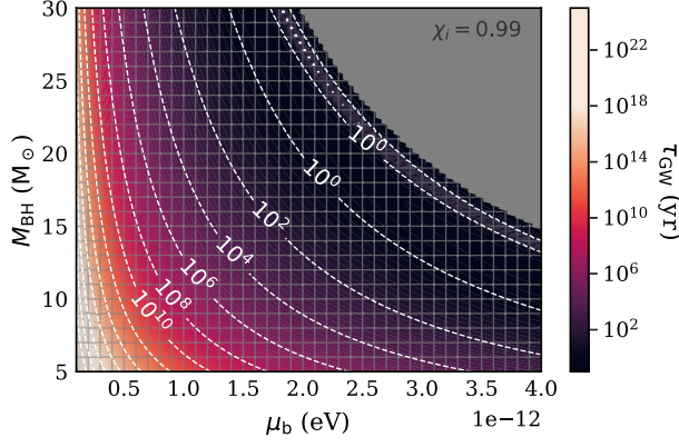
FIG. 4. The gravitational-wave signal amplitude decay half-time \tau_{\text{GW}} [Eq. (14)] ranges from longer than the Hubble time for lighter bosons to less than 100 yr for heavier bosons. The longer signals from lighter bosons are weaker compared to shorter signals from heavier bosons [Eq. (13)]. Like h_0 , \tau_{\text{GW}} is a nonmonotonic function of \alpha above \alpha \gtrsim 0.35 (Sec. A 4).
