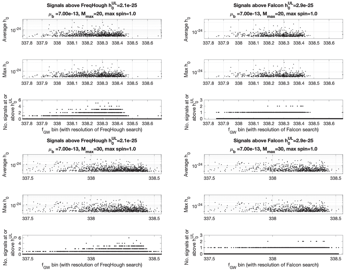
FIG. 40. The x axes show the signal frequency binned with the resolution of the two searches: (left panels) Freq Hough, 2.4 \times 10^{-4} Hz [22] and (right panels) Falcon, 1.7 \times 10^{-5} Hz [20,21]. From the bottom panel up, the y axis shows the number of detectable signals in each bin, their maximum intrinsic amplitude, and their average amplitude.
