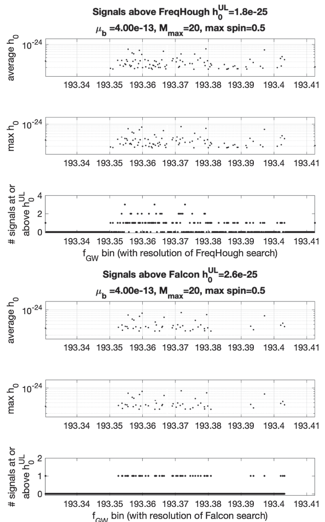
FIG. 20. Same plots as those in Fig. 19 but with the assumption that the maximum initial spin of the black hole population is 0.5.
