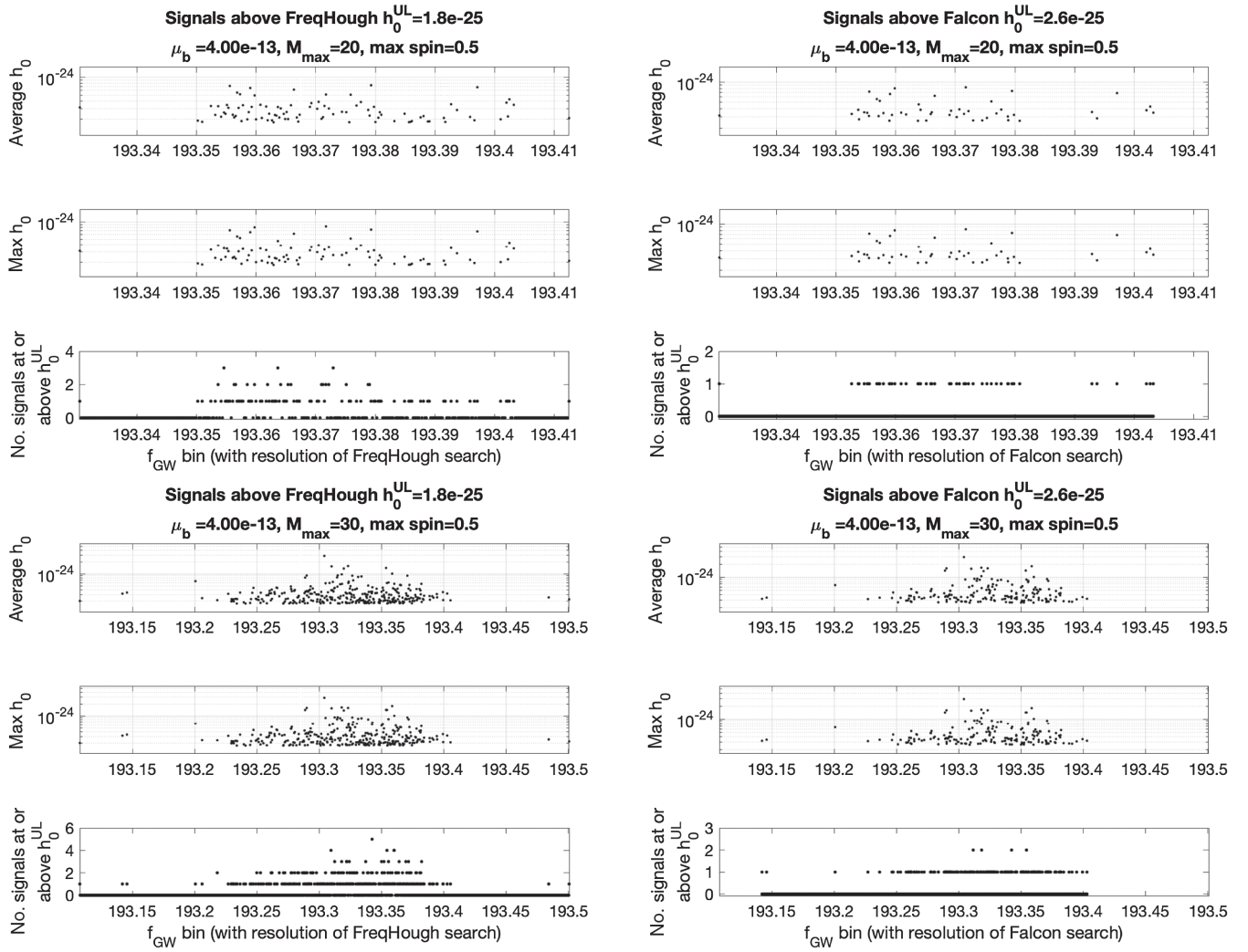
FIG. 37. The x -axis plots show the signal frequency binned with the resolution of the two searches: (left panels) Freq Hough, 2.4 \times 10^{-4} Hz [22] and (right panels) Falcon [20,21], 1.7 \times 10^{-5} Hz. From the bottom panel up, the y axis shows the number of detectable signals in each bin, their maximum intrinsic amplitude, and their average amplitude.
