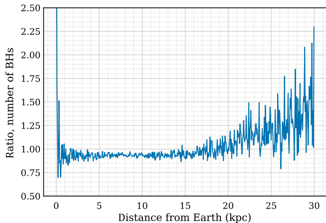
FIG. 24. If black holes are born with faster natal kicks (100 rather than 50 km/s), more of them have sufficiently high speeds to escape the gravitational pull of the Galactic bulge and disk. This causes a slight deficit of black holes at small Galactic radii, which also means there are fewer BHs close to Earth, decreasing on average the number of loud signals.
