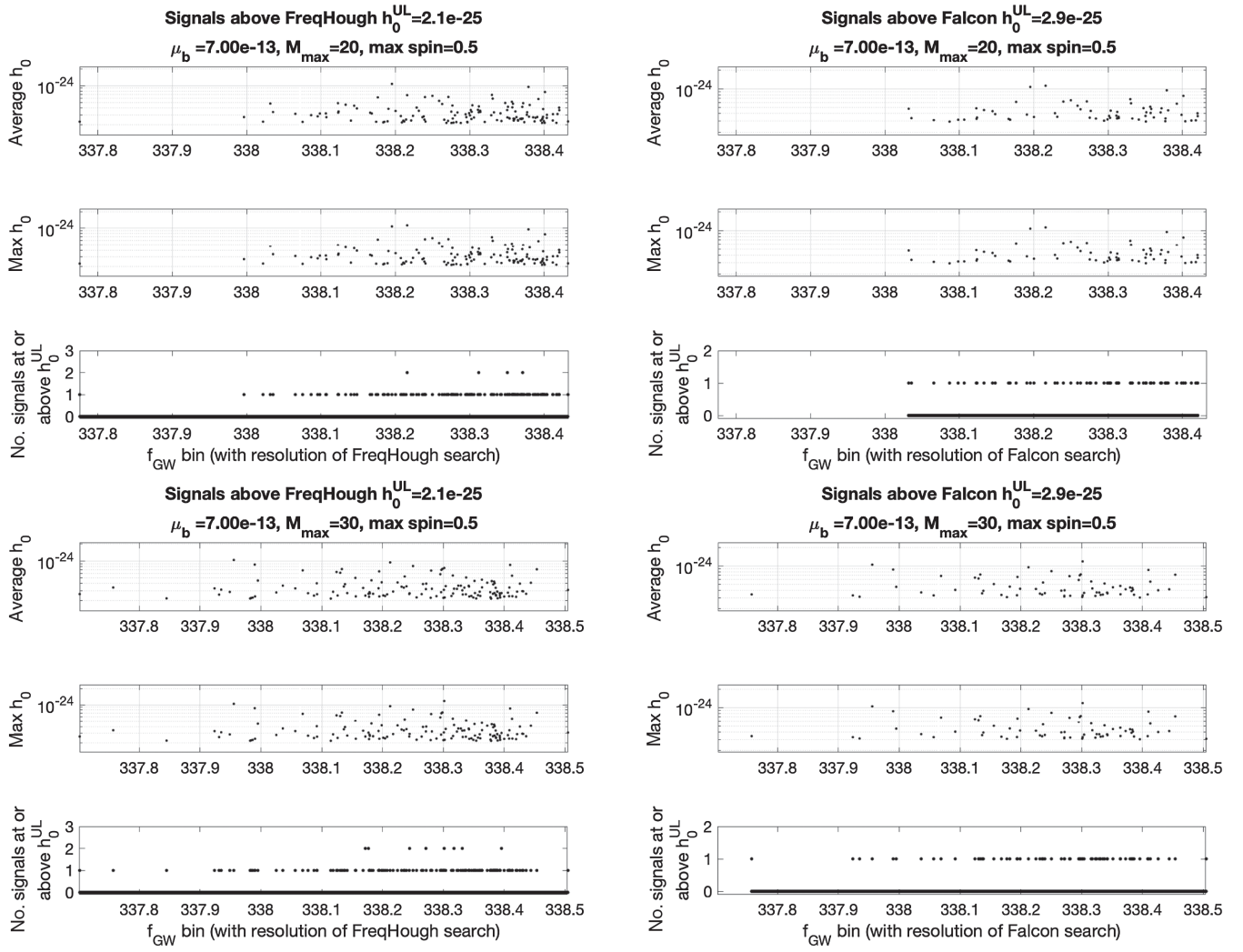
FIG. 41. The x axes show the signal frequency binned with the resolution of the two searches: (left panels) Freq Hough, 2.4 \times 10^{-4} Hz [22] and (right panels) Falcon, 1.7 \times 10^{-5} Hz [20,21]. From the bottom panel up, the y axis shows the number of detectable signals in each bin, their maximum intrinsic amplitude, and their average amplitude.
