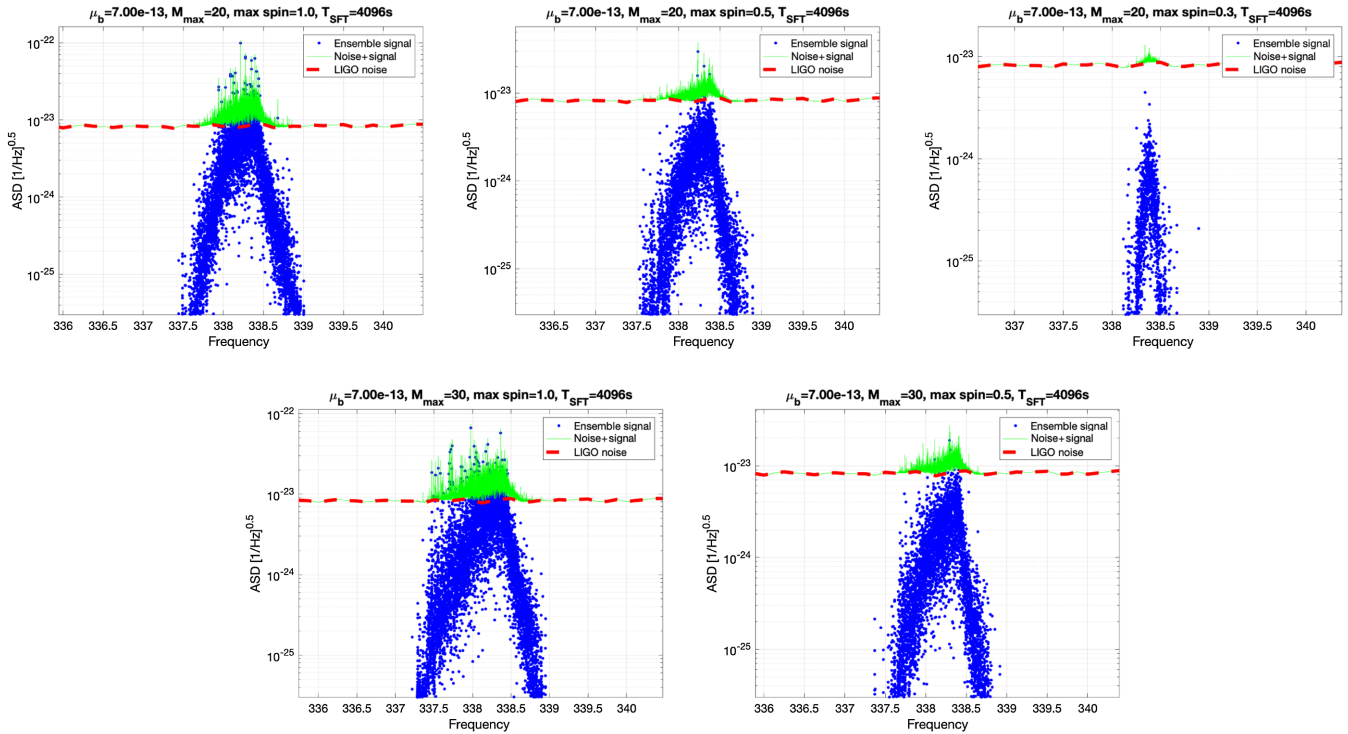
FIG. 45. The amplitude spectral density of the LIGO O2 data alone (dashed red line) and of an ensemble signal (top green points) assuming that \mu_b = 7 \times 10^{-13} eV and a Galactic black hole population with maximum mass 20M_\odot (top plots) and maximum initial spins of 0.3, 0.5, and 1, and maximum mass 30M_\odot (bottom plots) and maximum initial spins of 0.5 and 1. The time baseline assumed is 4096 s, as used by the Freq Hough search in this frequency range [22].
