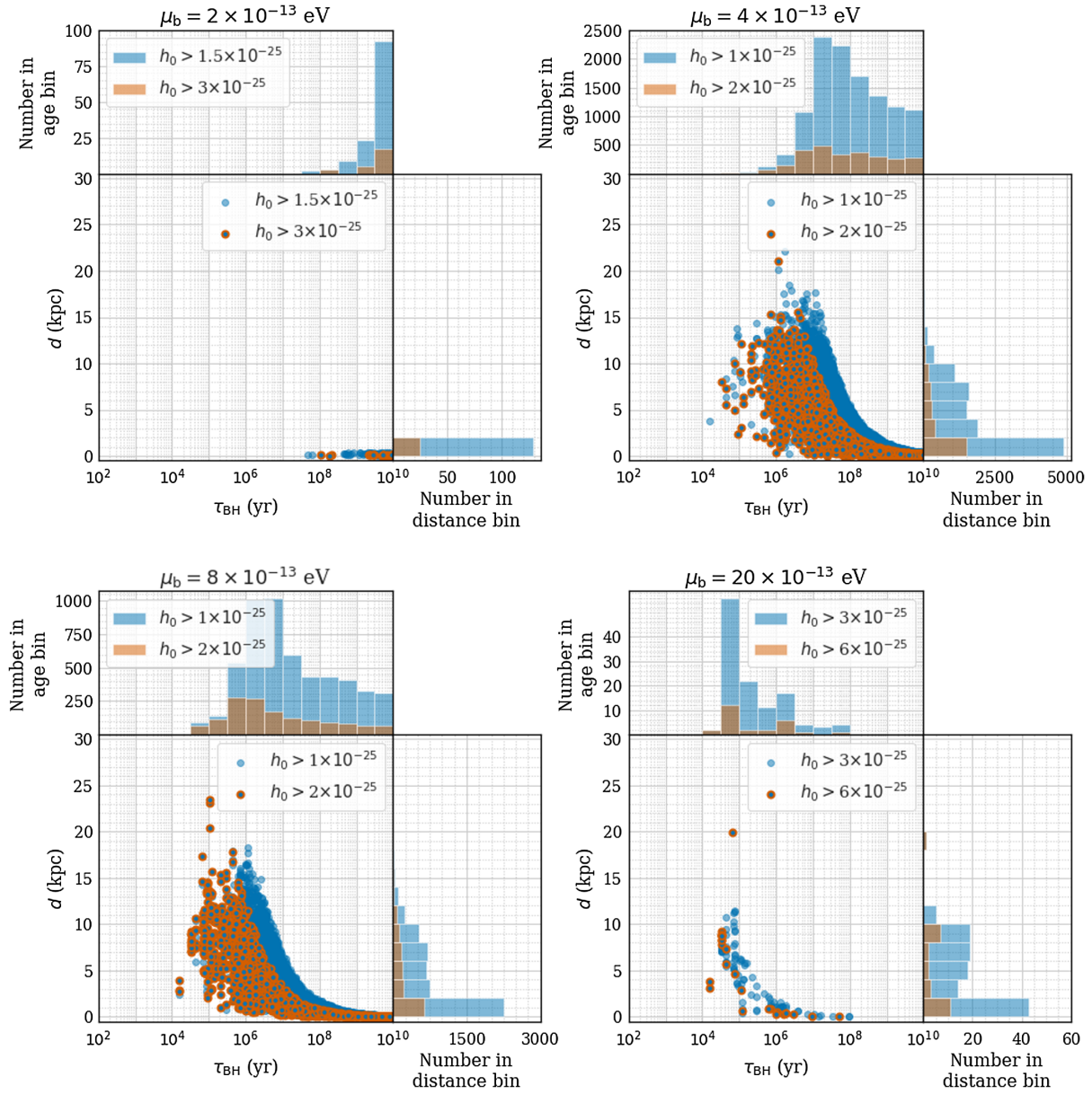
FIG. 34. Ages and distances of the heavy black hole population. As in Fig. 33, the addition of black holes with M_{BH} > 20M_{\odot} increases the number of detectable systems for the lighter bosons ( \mu_b = 2 \times 10^{-13} and 4 \times 10^{-13} eV) but has little to no effect on the heavier bosons.
