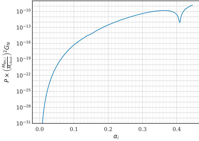
FIG. 22. The power emitted in the \tilde{\ell} = \tilde{m} = 2 spherical harmonics mode of the gravitational radiation, normalized by (M_{\text{BH},i}/M_{\text{cloud}})G_N to be a dimensionless quantity. The initial black hole spin assumed here is \chi_i = 0.99 ; the curves for other values of \chi_i are very similar and primarily differ in their maximum value of \alpha_i . The power for \alpha_i > 0.1 is calculated numerically [Eq. (A16)] and is suppressed for some high spins, resulting in a “dip” near \alpha \sim 0.4 . This directly affects the shape of h_0 and \tau_{\text{gw}} .
