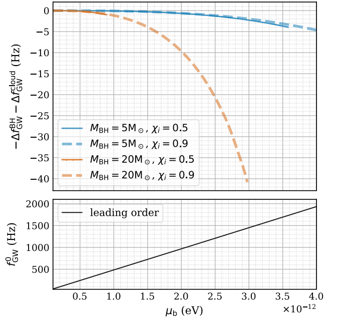
FIG. 5. Bottom panel: The leading-order gravitational-wave frequency f_{\text{GW}}^0 is proportional to the boson rest energy \mu_b [Eq. (9)]. Top panel: Systems with heavier black holes (orange curves) produce GW signals with lower frequencies than do systems with lighter black holes (blue curves) due to the larger gravitational binding energy. Systems with larger spins (dashed curves) result in slightly higher frequencies than systems with smaller spins (solid curves) due to a positive spin-orbit energy. The two solid curves—corresponding to \chi_i = 0.5 —stop at intermediate boson masses; for heavier bosons, \chi_c > 0.5 and the systems never form. The contribution from the cloud self-energy is of the order of 10^{-3} or less of the black hole’s gravitational potential energy.
