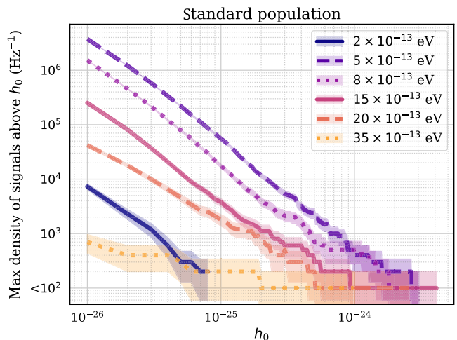
FIG. 17. The maximum density of signals above a given h_0 is up to an order of magnitude larger than the mean density (Fig. 16). Frequency ranges with sufficiently high signal densities can cause complications for standard searches for continuous wave signals (Sec. V). The contours show the uncertainty \sqrt{N}/\Delta f , where N is the number of signals and \Delta f = 0.01 Hz is the size of the frequency bin over which the maximum density is calculated.
