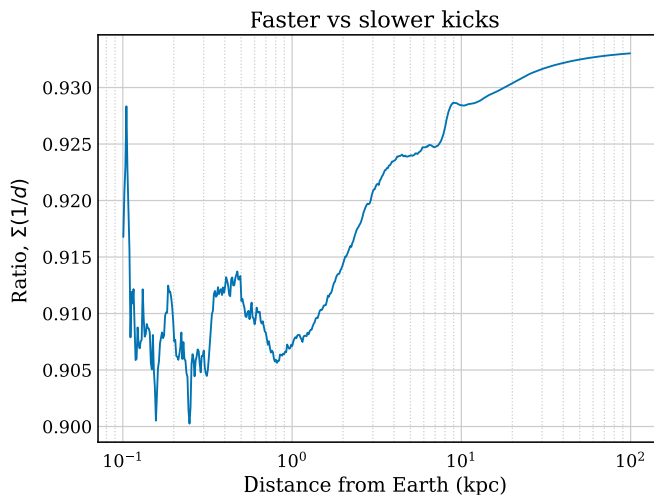
FIG. 25. The ratio of the sum of 1/d for all the black holes within a distance d provides a comparison of the number of signals between the two populations. Here we plot the ratio for the population with faster versus slower kicks. Overall, this ratio is smaller than unity and is decreasing toward shorter distances; the ratio is affected by small number statistics at distances much less than 1 kpc. The lower signal number is consistent with the fact that the population of black holes with faster kicks in general produces fewer signals above a given h_0 (Fig. 25).
