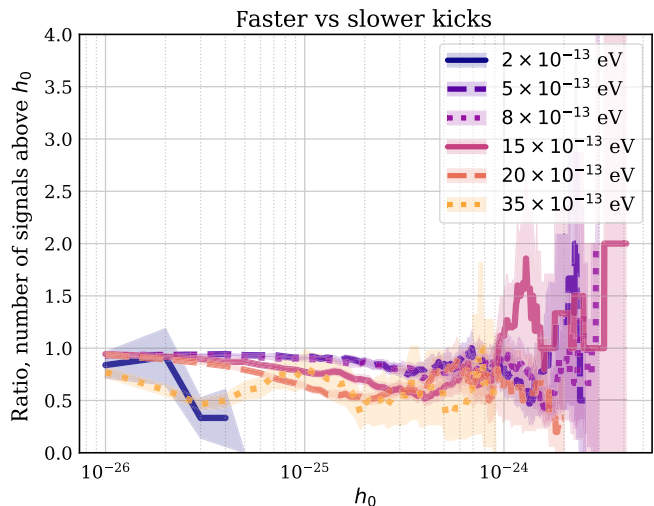
FIG. 26. The loudest signals in an ensemble are in general produced by the closest black holes. A black hole population with slightly faster natal kicks produces a slight deficit of boson clouds close to Earth (Fig. 24), resulting in fewer signals at larger values of h_0 . This effect is greater for heavier bosons, as the louder signals are preferentially produced by closer black holes.
