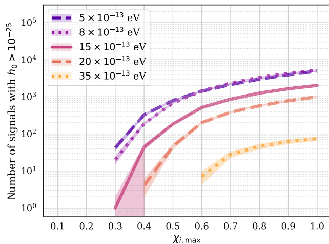
FIG. 13. The number of signals above h_0 > 10^{-25} depends on the maximum of the initial spin distribution, \chi_{i,\max} . For a cloud to form, the initial spin must be larger than the critical spin [Eq. (4)]. Since \chi_c increases with \alpha , this also results in fewer signals above a given strain for heavier bosons. The contours show Gaussian statistical uncertainties. There are no signals with amplitude h_0 > 10^{-25} for \mu_b = 2 \times 10^{-13} eV for any value of \chi_{i,\max} .
