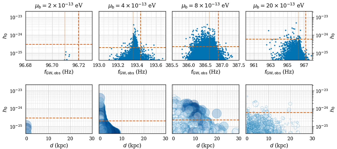
FIG. 10. The ensemble signals for the “standard” black hole population (Table I) and boson mass (left to right) \mu_b = 2 \times 10^{-13}, 4 \times 10^{-13}, 8 \times 10^{-13}, and 20 \times 10^{-13} eV. Top row: Each point represents the annihilation signal from an individual system, illustrating the range of strains and frequencies of the signals. The dashed horizontal red line corresponds to the approximate upper limit at that frequency reported by recent all-sky continuous wave searches [20,21,47,97]. The thick dashed vertical red line marks the values of f_{\text{GW}}^0 , and the dotted red line shows f_{\text{GW}} calculated using the mode of the M_{\text{BH}} distribution (Fig. 11). Bottom row: Distribution of strains as a function of distance and black hole mass. Smaller, whiter circles correspond to lighter black holes (minimum 5M_{\odot} ) and larger bluer circles correspond to heavier black holes (maximum 20M_{\odot} ); the differences in circle sizes are exaggerated for visual effect and do not scale linearly with M_{\text{BH}} . The horizontal dashed red line again represents current search upper limits.
