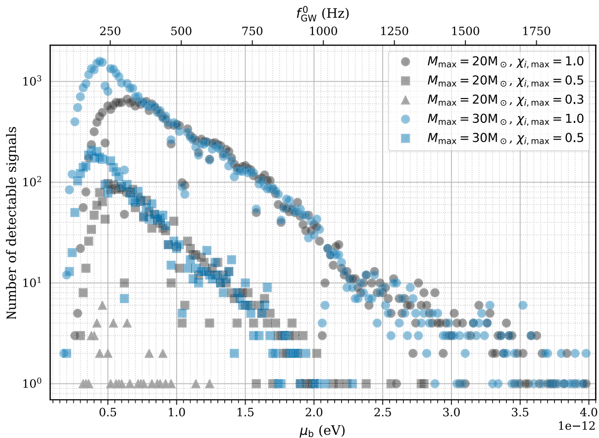
FIG. 18. Number of signals with amplitudes above the detectability level of recent all-sky searches for continuous gravitational waves [20–22], for bosons in the mass range 1 \times 10^{-13} to 4 \times 10^{-12} eV. The Falcon search [20,21] provides 95% confidence strict upper limits on continuous wave emission with near-zero frequency derivative between 20 and 600 Hz. These upper limits are valid for any sky position and polarization of the source, even the ones with the most unfavorable coupling to the detectors. In contrast, the upper limits from the Freq Hough search [22] hold for 95% of the entire population. For this reason, even at the same sensitivity, the Freq Hough upper limits are lower than the Falcon upper limits. We use the Falcon upper limits for bosons with \mu_b < 1.2 \times 10^{-12} eV and the Freq Hough upper limits for bosons with \mu_b \geq 1.2 \times 10^{-12} eV. We consider the standard (black circles) and heavy (blue circles) black hole populations, as well as the moderate (gray squares), heavy moderate (blue squares), and pessimistic (gray triangles) spin populations. The fluctuations are due to stationary lines and other artifacts in the detectors, which decrease the continuous wave search sensitivity in nearby frequency bins.
