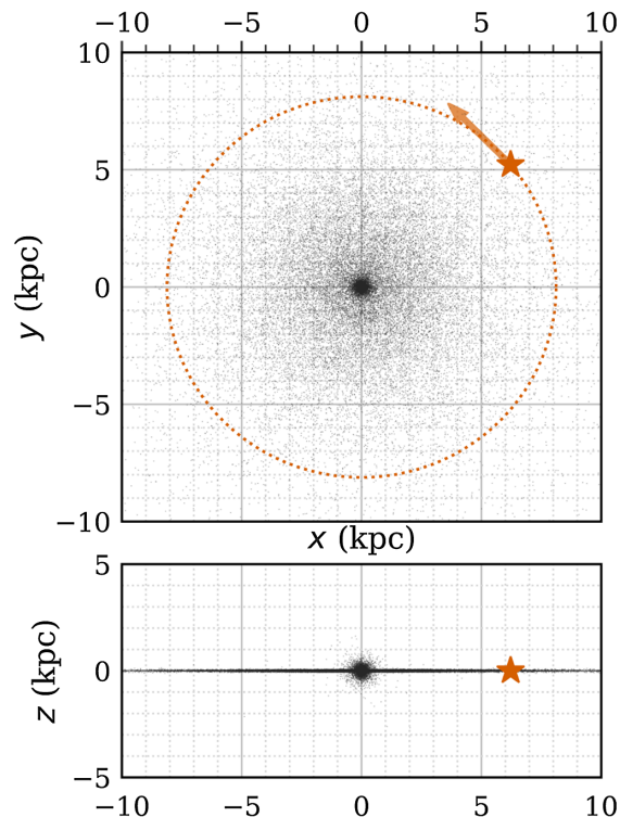
FIG. 6. Top-down (top panel) and edge-on (bottom panel) view of the Galaxy, showing a random sample of 30,000 black holes from our simulated population. The disk and bulge components are visually distinct. Our simulations assume axial symmetry, so the results do not change if the position of the Sun is chosen arbitrarily on the circle of distance \sim 8 kpc from the Galactic Center (orange circle). As explained in the text, we exploit this freedom to simulate 10^8 black holes starting from a set of 10^6 . The orange star marks one sample position and the arrow shows its velocity in the disk, tangential to the circle.
