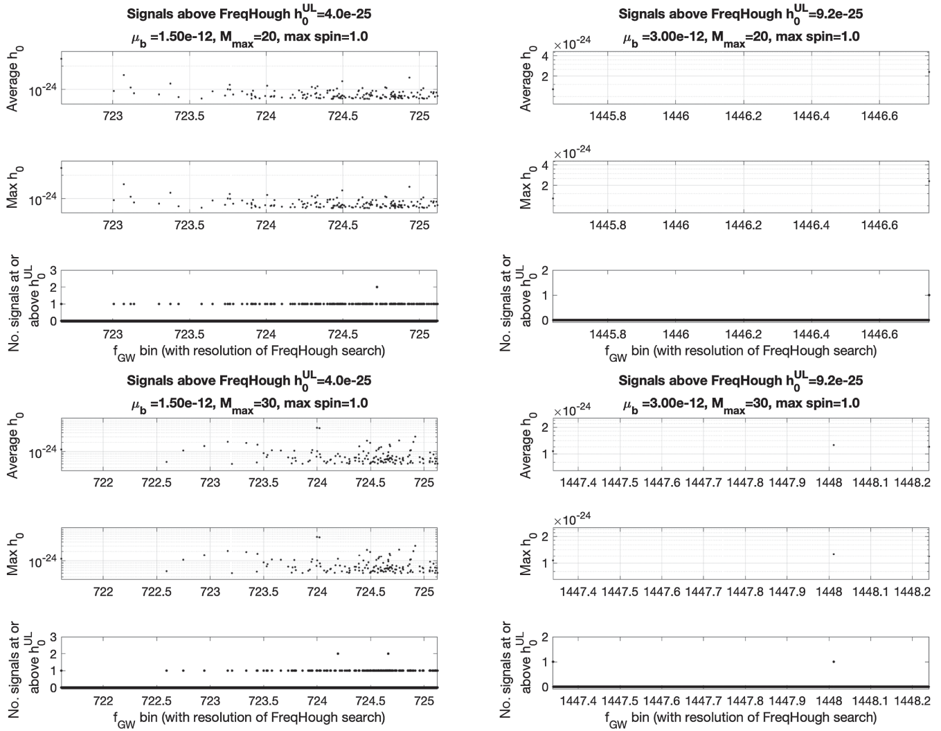
FIG. 42. The x axes show the signal frequency binned with the resolution of the two searches: (left panels) Freq Hough, 2.4 \times 10^{-4} Hz [22] and (right panels) Falcon, 1.7 \times 10^{-5} Hz [20,21]. From the bottom panel up, the y axis shows the number of detectable signals in each bin, their maximum intrinsic amplitude, and their average amplitude.
