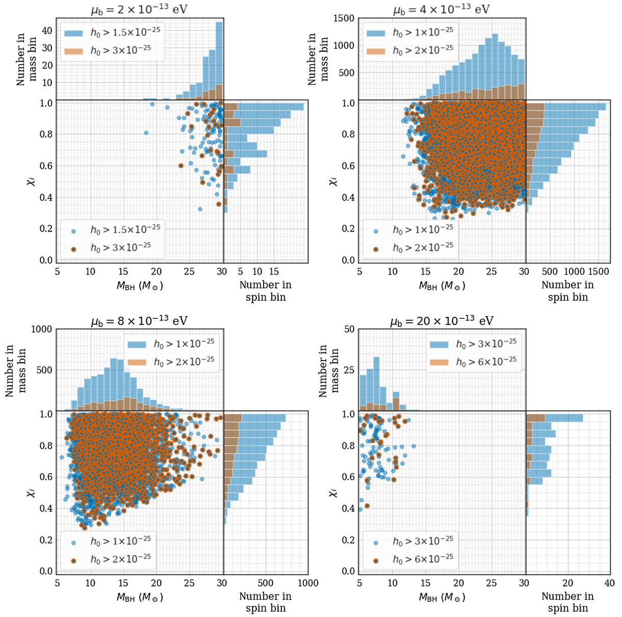
FIG. 33. Mass and spin properties of the heavy black hole population. For the two heavier boson masses ( \mu_b = 8 \times 10^{-13} and 2 \times 10^{-12} eV), the black holes that produce the potentially detectable ensemble signals have similar properties to the black holes that produce the signals in Fig. 10 (the standard population) due to the fact that systems with large values of \alpha have dramatically shortened lifetimes. For the two lighter boson masses ( \mu_b = 2 \times 10^{-13} and 4 \times 10^{-13} eV), the addition of black holes with M_{\text{BH}} > 20M_\odot greatly increases the number of detectable signals.
