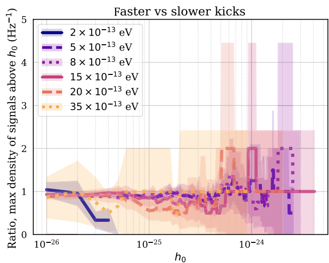
FIG. 27. The ratio of maximum signal density above a given h_0 between the faster and slower kick populations is consistent with unity.
