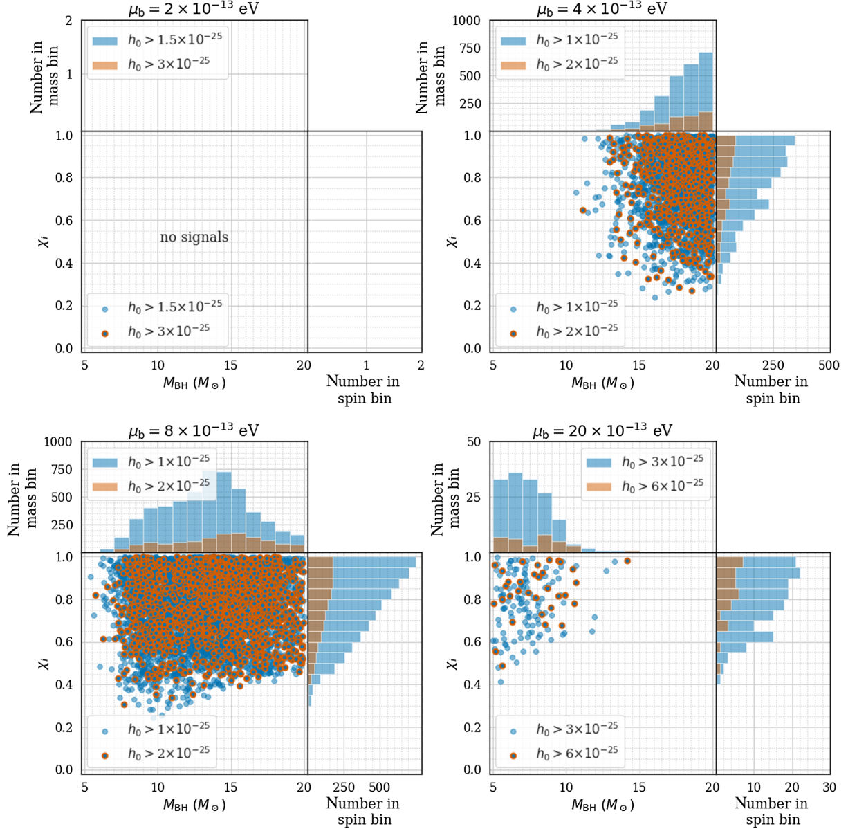
FIG. 11. Each of the four panels shows the mass M_{\text{BH}} and initial spin \chi_i of the black holes that produce the ensemble signals for the four boson masses from Fig. 10, assuming the standard black hole population (Table I). In each panel, the scatterplot shows M_{\text{BH}} and \chi_i for the systems that are detectable with the current search sensitivities (blue circles with orange outlines) and a factor of 2 improvement in sensitivity (blue circles). The histograms show the distributions of M_{\text{BH}} (top panels) and \chi_i (right panels) for these sets of systems. The black holes are assigned spins uniformly distributed in [0, 1] , and only systems satisfying Eq. (4) will form clouds. The upper-left set of plots ( \mu_b = 2 \times 10^{-13} eV) contains no signals at these values of h_0 , suggesting that a larger increase in sensitivity is necessary to detect the annihilation signals produced by the lightest bosons.
