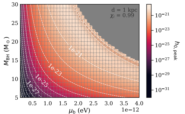
FIG. 3. Maximum characteristic strain h_{0,\text{peak}} for a rapidly rotating black hole as a function of black hole mass M_{\text{BH}} and boson mass \mu_b at a distance of d = 1 kpc. The peak strain scales as 1/d . The value of h_0 increases with \alpha until \alpha \sim 0.35 ; the quadrupolar gravitational-wave power—and thus the observed strain—changes nonmonotonically at large \alpha (Sec. A 4).
