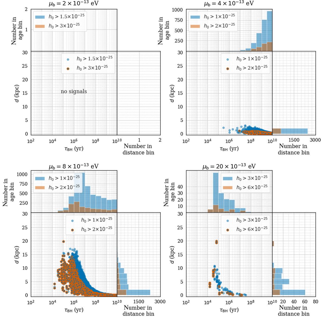
FIG. 12. Each of the four panels shows the age \tau_{\text{BH}} and distance d of the black holes that produce the ensemble signals for the four boson masses in Fig. 10, assuming the standard black hole population (Table I). In each panel, the scatterplot shows \tau_{\text{BH}} and d for the systems that are detectable with the current search sensitivities (blue circles with orange outlines) and a factor of 2 improvement in sensitivity (blue circles). The histograms show the distributions of \tau_{\text{BH}} (top panels) and d (right panels) for these sets of systems. As in Fig. 11, the upper-left set of plots ( \mu_b = 2 \times 10^{-13} eV) contains no signals at these values of h_0 .
