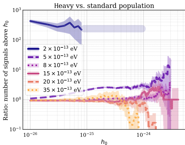
FIG. 30. The ratio of the number of signals above a given h_0 for the heavy ( M_{\text{BH,max}} = 30M_{\odot} ) versus standard ( M_{\text{BH,max}} = 20M_{\odot} ) populations. The number of signals for the lighter bosons ( \mu_b = 2 \times 10^{-13} and 5 \times 10^{-13} eV) increases in going from the standard to the heavy black hole population, while the number of signals for the heavier bosons stays approximately the same (Sec. VA). For \mu_b = 2 \times 10^{-13} eV, the signals from the heavy black hole population extend to strains of h_0 \approx 10^{-24} (indicated by the light, thick bar) while the signals from the standard black hole population only have h_0 \leq 10^{-25} .
