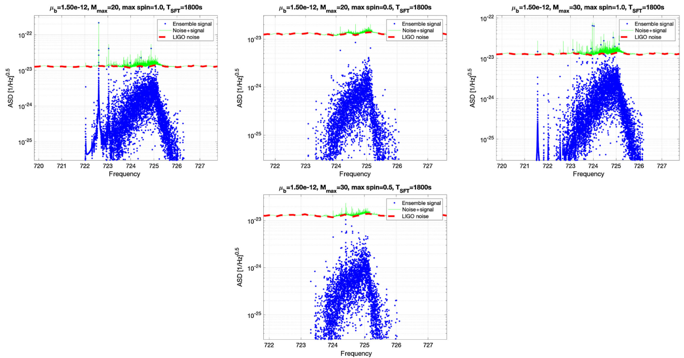
FIG. 46. The amplitude spectral density of the LIGO O2 data alone (dashed red line) and of an ensemble signal (top green points) assuming that \mu_b = 1.5 \times 10^{-12} eV and a Galactic black hole population with maximum mass 20M_\odot or 30M_\odot and maximum initial spins of 0.5 and 1. The time baseline assumed is 1800 s, close to what is used by the Freq Hough search in this frequency range [22]. The distinct excess at low frequencies arises from an exceptionally young and nearby black hole.
