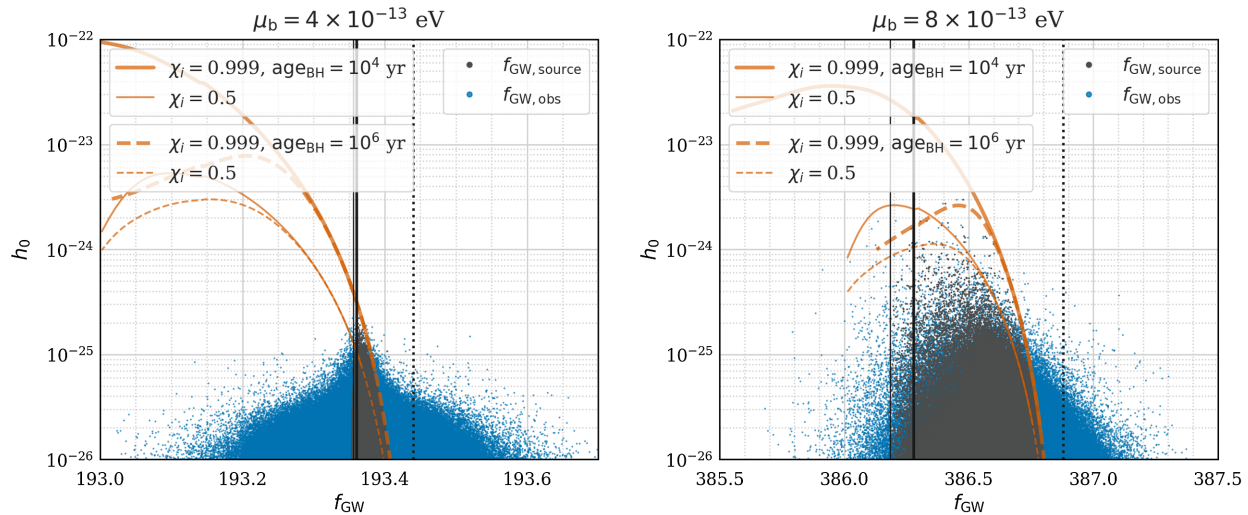
FIG. 9. The distribution of signal strains as a function of source frequency (gray dots) and observed frequency with Doppler shift (blue dots). The strains are selected for signals with d \geq 1 kpc to facilitate comparison to the strain as a function of source frequency for a system at a distance d = 1 kpc: the upper envelope for two sets of black hole spin and age parameters is shown in orange. The black vertical lines show the boundaries of the source frequency distribution: the vertical dotted line shows the rest mass frequency f_{\text{GW}}^0 , and the thick and thin vertical lines correspond to f_{\text{GW,source}} for (20M_{\odot}, \chi_i = 0.999) and (20M_{\odot}, \chi_i = 0.5) , yielding successively more negative potential energy corrections. (In the left panel, the two solid vertical lines lie close to each other.)
