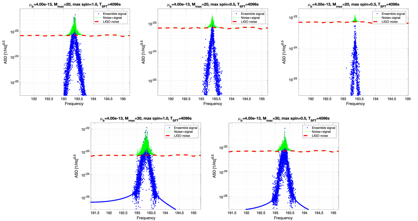
FIG. 44. The amplitude spectral density of the LIGO O2 data alone (dashed red line) and of an ensemble signal (top green points) assuming that \mu_b = 4 \times 10^{-13} eV and a Galactic black hole population with maximum mass 20M_\odot (top plots) and maximum initial spins of 0.3, 0.5, and 1, and maximum mass 30M_\odot (bottom plots) and maximum initial spins of 0.5 and 1. The time baseline assumed is 4096 s, as used by the Freq Hough search in this frequency range [22].
