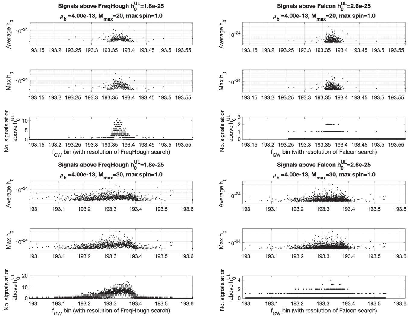
FIG. 36. The x axes show the signal frequency binned with the resolution of the two searches: (left panels) Freq Hough, 2.4 \times 10^{-4} Hz [22] and (right panels) Falcon [20,21], 1.7 \times 10^{-5} Hz. From the bottom panel up, the y axis shows the number of detectable signals in each bin, their maximum intrinsic amplitude, and their average amplitude.
