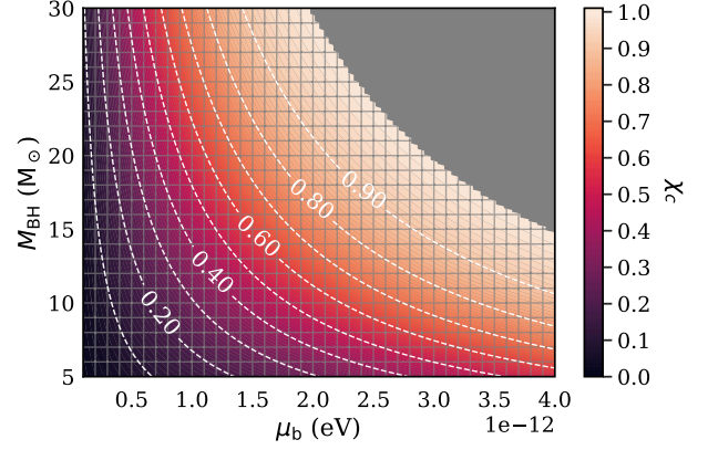
FIG. 2. Critical spin \chi_c for the (n, \ell, m) = (0, 1, 1) bound state. The critical spin is a function of the gravitational fine structure constant \alpha and the bound state quantum numbers. A cloud of bosons with rest energy \mu_b will form around a black hole of mass M_{\text{BH}} and initial spin \chi_i only if \chi_i > \chi_c [Eq. (4)].
