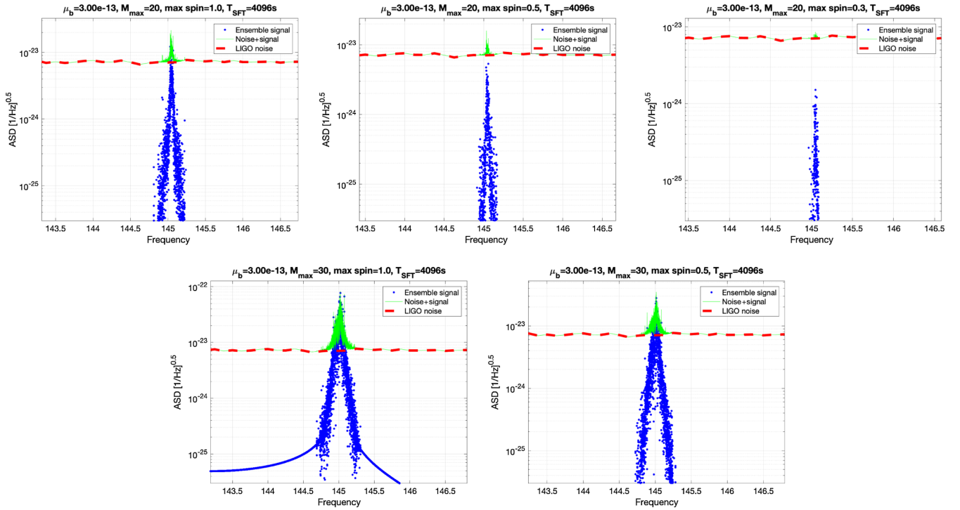
FIG. 43. The amplitude spectral density of the LIGO O2 data alone (dashed red line) and of an ensemble signal (top green points) assuming that \mu_b = 3 \times 10^{-13} eV and a Galactic black hole population with maximum mass 20M_\odot (top plots) and max initial spin of 0.3, 0.5 and 1, and maximum mass 30M_\odot (bottom plots) and maximum initial spins of 0.5 and 1. The time baseline assumed is 4096 s, as used by the Freq Hough search in this frequency range [22].
