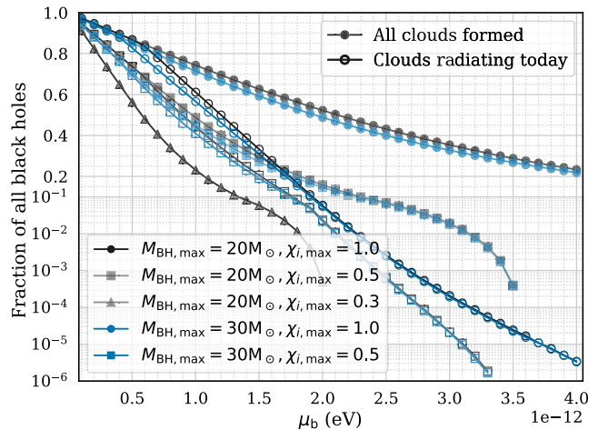
FIG. 14. For a given boson mass, a fraction of black holes is born with spins high enough to support cloud formation (filled markers). Gravitational-wave emission stops when the second level is fully populated, so a subset of the initial clouds are still emitting today (unfilled markers). We consider the five black hole populations of Table I: standard (black circles), heavy (blue circles), moderate spins (gray squares), heavy with moderate spins (blue squares), and pessimistic spin (gray triangles) populations. The percentage of systems still emitting today decreases rapidly with increasing boson mass; at \mu_b = 4 \times 10^{-12} eV, only up to one in every 10^6 black holes in the Galaxy is in a currently emitting system.
