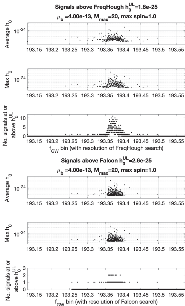
FIG. 19. The x axes show the signal frequency binned with the resolution of the two searches: 2.4 \times 10^{-4} Hz for the Freq Hough search and 1.7 \times 10^{-5} Hz for the Falcon search. From the bottom panel going up, the y axis shows the number of detectable signals in each bin, their maximum intrinsic amplitude, and their average amplitude. The main reason why there are fewer signals per frequency bin in the Falcon searches [20,21] than in the Freq Hough search [22] is that the frequency bin of Freq Hough is significantly larger (by a factor of 14) than the frequency bin of Falcon. The maximum initial spin of the black hole population is taken to be 1.
