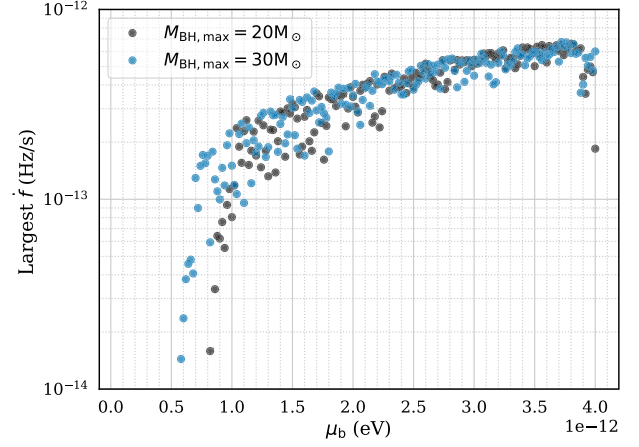
FIG. 23. The spin-up \dot{f} due to the decreasing binding energy of the cloud depends on \mu_b and M_{\text{BH}} [Eq. (16)]. For both the standard and heavy black hole populations, the largest value of \dot{f} is 6 \times 10^{-13} Hz/s.
