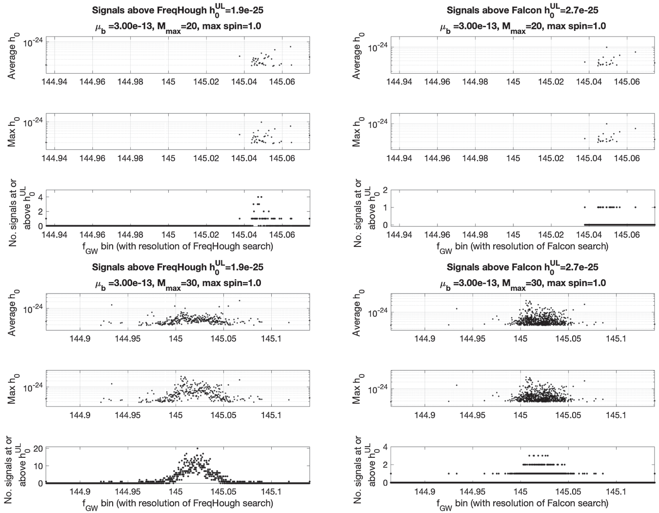
FIG. 35. The x axes show the signal frequency binned with the resolution of the two searches: (left panels) Freq Hough, 2.4 \times 10^{-4} Hz [22] and (right panels) Falcon, 1.7 \times 10^{-5} Hz [20,21]. From the bottom panel up, the y axis shows the number of detectable signals in each bin, their maximum intrinsic amplitude, and their average amplitude.
