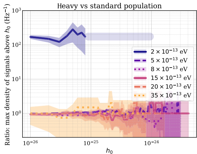
FIG. 32. For the six boson masses plotted here, the ratio of the maximum signal density above a given h_0 for the heavy versus standard black hole populations is similar to the ratio of the mean signal density. The maximum signal density for the lightest boson ( \mu_b = 2 \times 10^{-13} eV) is over 100 times larger for the heavier black hole population.
