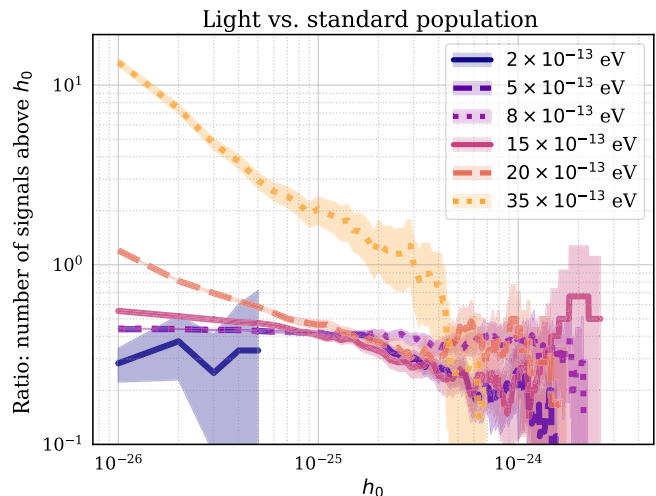
FIG. 29. Increasing the number of light black holes ( M_{\text{BH}} < 5M_{\odot} ) while maintaining the same number of black holes effectively reduces the number of black holes at all other masses. Therefore, the number of signals above a given h_0 decreases by a factor of 2 for most of the boson masses. The exception is the heaviest boson ( \mu_b = 3.5 \times 10^{-12} eV), for which the number of signals is larger with the light black hole population for signals with h_0 < 3 \times 10^{-25} .
