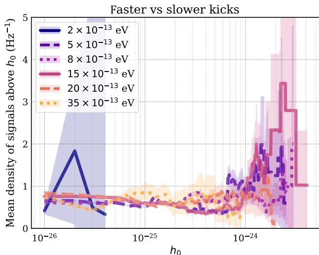
FIG. 28. The ratio of mean signal density above a given h_0 between the faster and slower kick populations reflects the number of signals above a given h_0 (Fig. 26). In general, black holes with faster natal kicks produce signals with larger Doppler shifts, thereby increasing the frequency range spanned by the ensemble and decreasing the mean signal density further.
