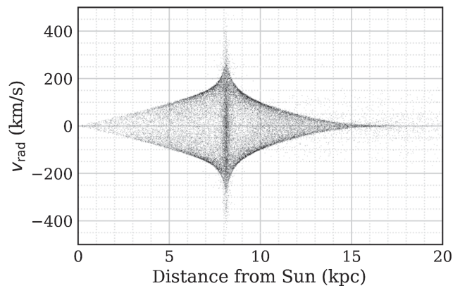
FIG. 7. Radial velocities of the black holes of Fig. 6 as a function of their distance from the Sun. The distribution is symmetric around zero km/s and is widest at 8 kpc, corresponding to the distance of the Galactic Center, as the bulk velocity in the bulge is uniformly distributed in direction. In contrast, since the bulk velocity in the disk is in the \phi direction within the Galactic plane, the radial velocity of black holes in the disk (i.e., not near 8 kpc) has smaller magnitude. The scatter in velocities at large distances from the Sun is due to the black holes that have wandered into the halo and no longer follow the bulk motion of the disk.
