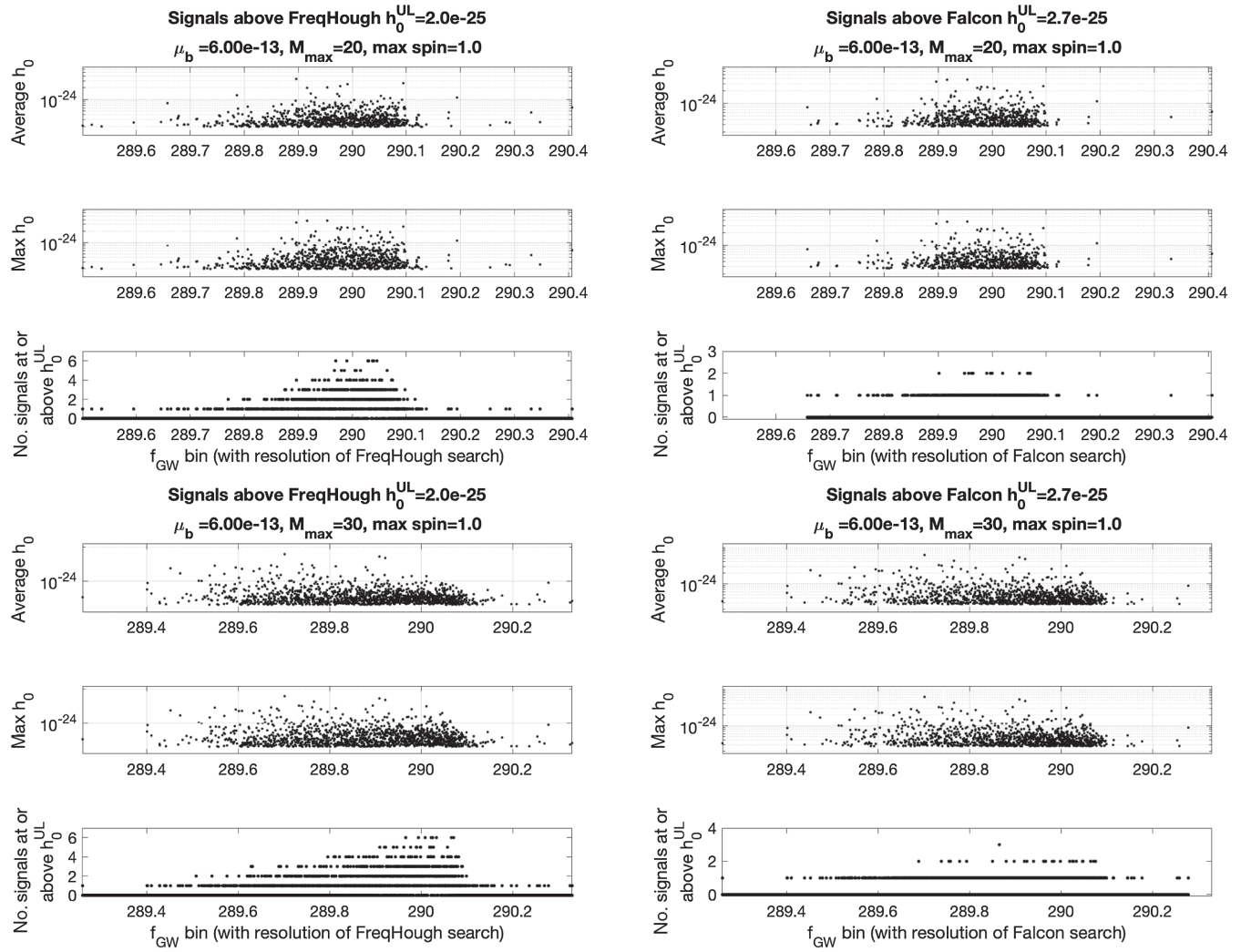
FIG. 38. The x axes show the signal frequency binned with the resolution of the two searches: (left panels) Freq Hough, 2.4 \times 10^{-4} Hz [22] and (right panels) Falcon [20,21], 1.7 \times 10^{-5} Hz. From the bottom panel up, the y axis shows the number of detectable signals in each bin, their maximum intrinsic amplitude, and their average amplitude.
