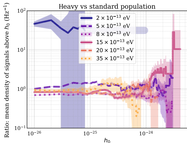
FIG. 31. The ratio of the mean signal density above a given h_0 for the heavy versus standard black hole populations is approximately unity for the five heavier boson masses. For the lightest mass ( \mu_b = 2 \times 10^{-13} eV), the mean density is over 10 times larger for the heavier black hole population.
