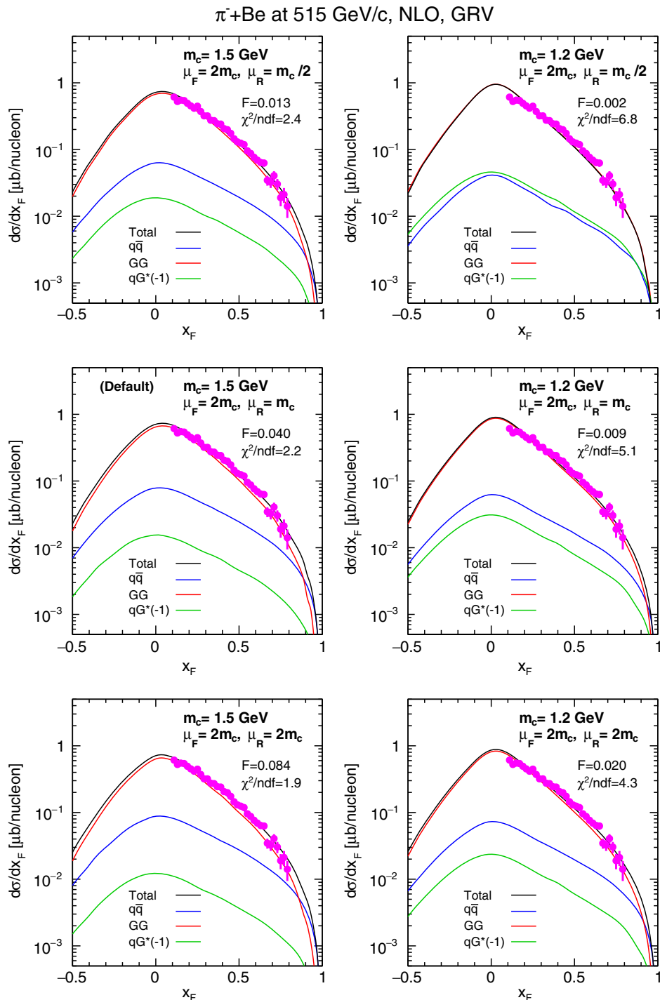
FIG. 11. The NLO CEM results with variation of charm quark mass m_c and renormalization scale \mu_R , compared with the d\sigma/dx_F data of J/\psi production off the beryllium target with a 515-GeV \pi/c^- beam from the E672/E706 experiment [68]. The pion PDFs used for the calculation is GRV. The total cross sections and q\bar{q} , GG , and qG \times (-1) contributions are denoted as black, blue, red, and green lines, respectively. The charm quark mass m_c , factorization scale \mu_F , and renormalization scale \mu_R used for the CEM calculation as well as the fit \chi^2/\text{ndf} and F factors are displayed in each plot.
