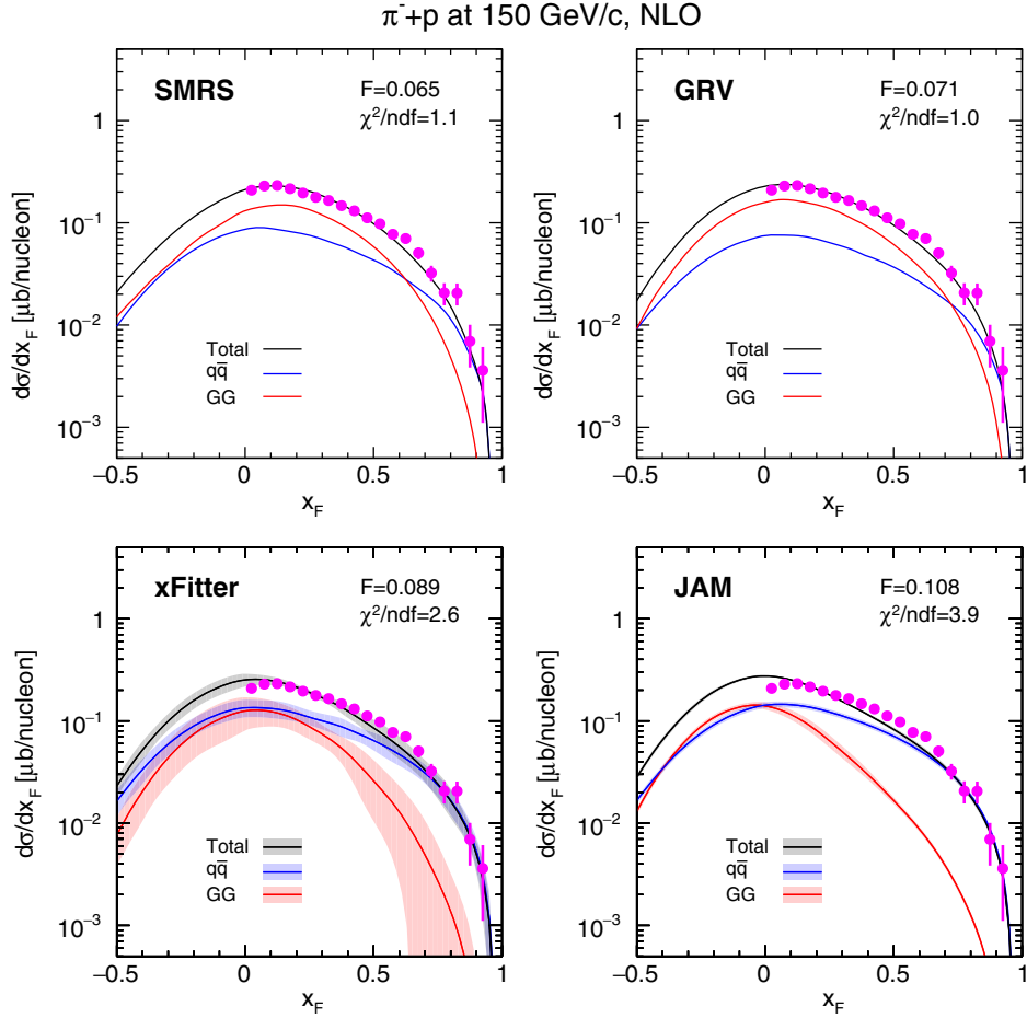
FIG. 8. Comparison of the NLO CEM results for the SMRS, GRV, xFitter, and JAM PDFs, with the d\sigma/dx_F data of J/\psi production off the hydrogen target with a 150-GeV/c \pi^- beam from the NA3 experiment [70]. The total cross sections and q\bar{q} and GG contributions are denoted as black, blue, and red lines, respectively.
