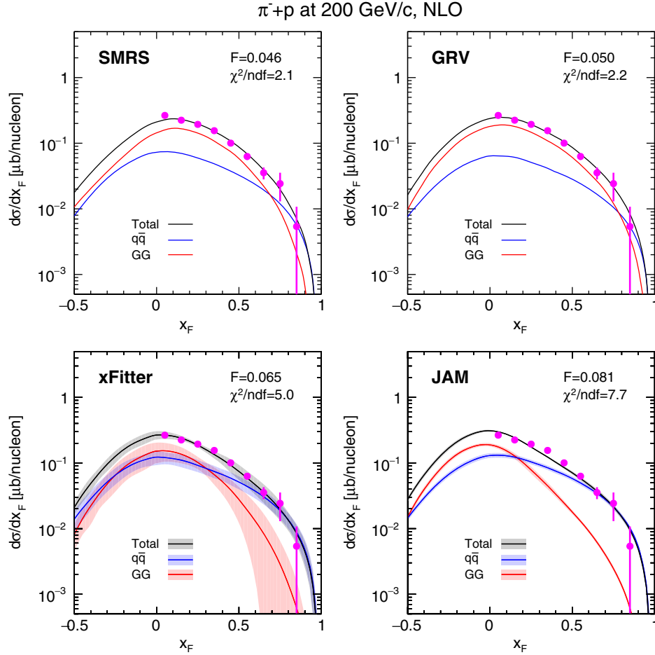
FIG. 6. Comparison of the NLO CEM results for the SMRS, GRV, xFitter, and JAM PDFs, with the d\sigma/dx_F data of J/\psi production off the hydrogen target with a 200-GeV/ c \pi^- beam from the NA3 experiment [70]. The total cross sections and q\bar{q} and GG contributions are denoted as black, blue, and red lines, respectively.
