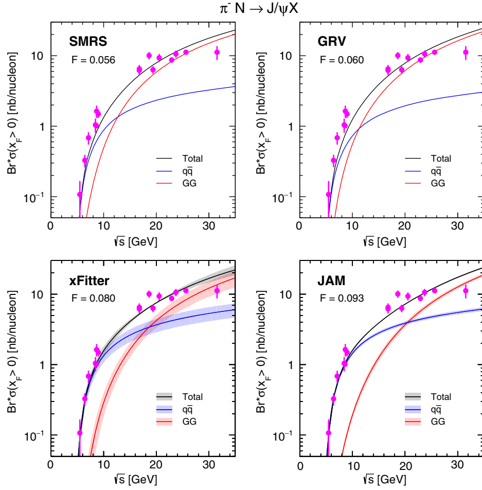
FIG. 2. The product of J/\psi dimuon decay branching ratio ( \text{Br} ) and J/\psi production cross sections at x_F > 0 for the \pi^- N reaction, calculated with four pion PDFs (SMRS, GRV, xFitter, and JAM) is compared with data (solid circles) [46,67]. The black, blue, and red curves represent the calculated total cross section and the q\bar{q} and GG contributions, respectively. The shaded bands on the xFitter and JAM calculations come from the uncertainties of the corresponding PDF sets. The SMRS and GRV PDFs contain no information on uncertainties.
