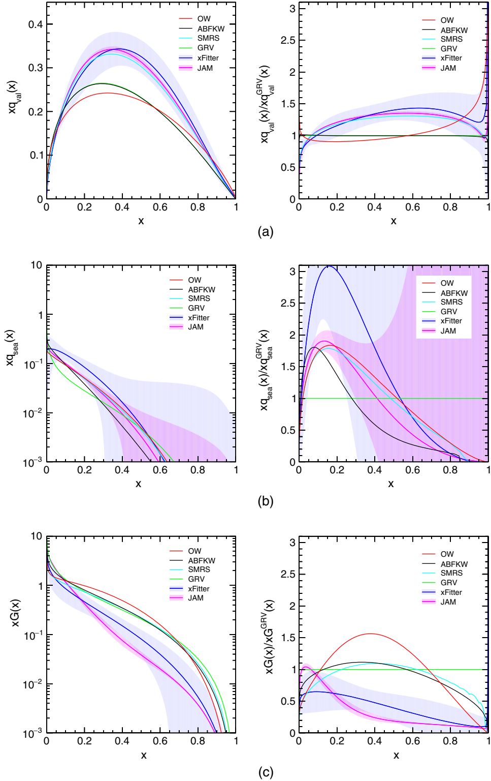
FIG. 1. Momentum density distributions [ xf(x) ] of (a) valence quarks, (b) sea quarks, and (c) gluons of various pion PDFs and their ratios to GRV, at the scale of J/\psi mass ( Q^2 = 9.6 \text{ GeV}^2 ).
