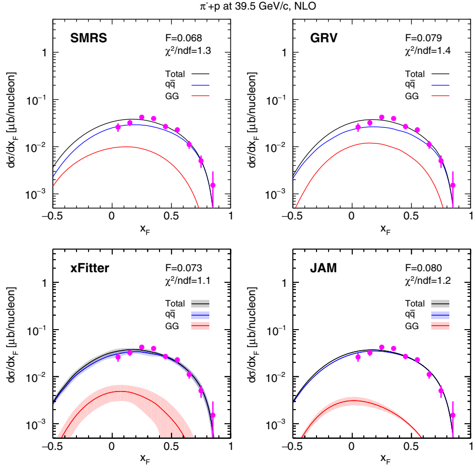
FIG. 10. Comparison of the NLO CEM results for the SMRS, GRV, xFitter, and JAM PDFs, with the d\sigma/dx_F data of J/\psi production off the hydrogen target with a 39.5-GeV/c \pi^- beam from the WA39 experiment [74]. The total cross sections and q\bar{q} and GG contributions are denoted as black, blue, and red lines, respectively.
