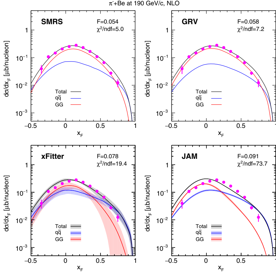
FIG. 7. Comparison of the NLO CEM results for the SMRS, GRV, xFitter, and JAM PDFs, with the d\sigma/dx_F data of J/\psi production off the beryllium target with a 190-GeV/ c \pi^- beam from the WA11 experiment [72]. The total cross sections and q\bar{q} and GG contributions are denoted as black, blue, and red lines, respectively.
