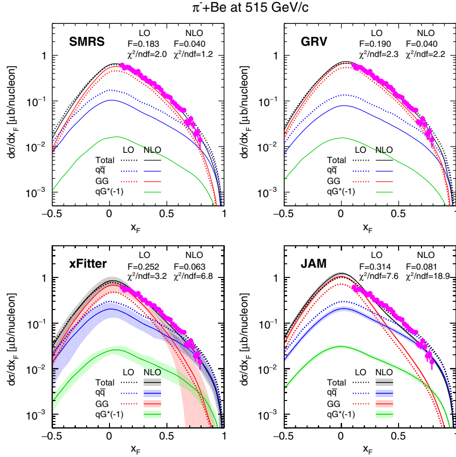
FIG. 3. Comparison of the LO and NLO CEM results for the SMRS, GRV, xFitter, and JAM PDFs, with the d\sigma/dx_F data of J/\psi production off the beryllium target with a 515-GeV/c \pi^- beam from the E672/E706 experiment [68]. The total cross sections and q\bar{q} , GG , and qG \times (-1) contributions are denoted as black, blue, red, and green lines, respectively. Solid and dotted lines are for the NLO and LO calculations, respectively. The shaded bands on the xFitter and JAM calculations come from the uncertainties of the corresponding PDF sets. For clarity, the resulting \chi^2/\text{ndf} and F factors are also displayed.
