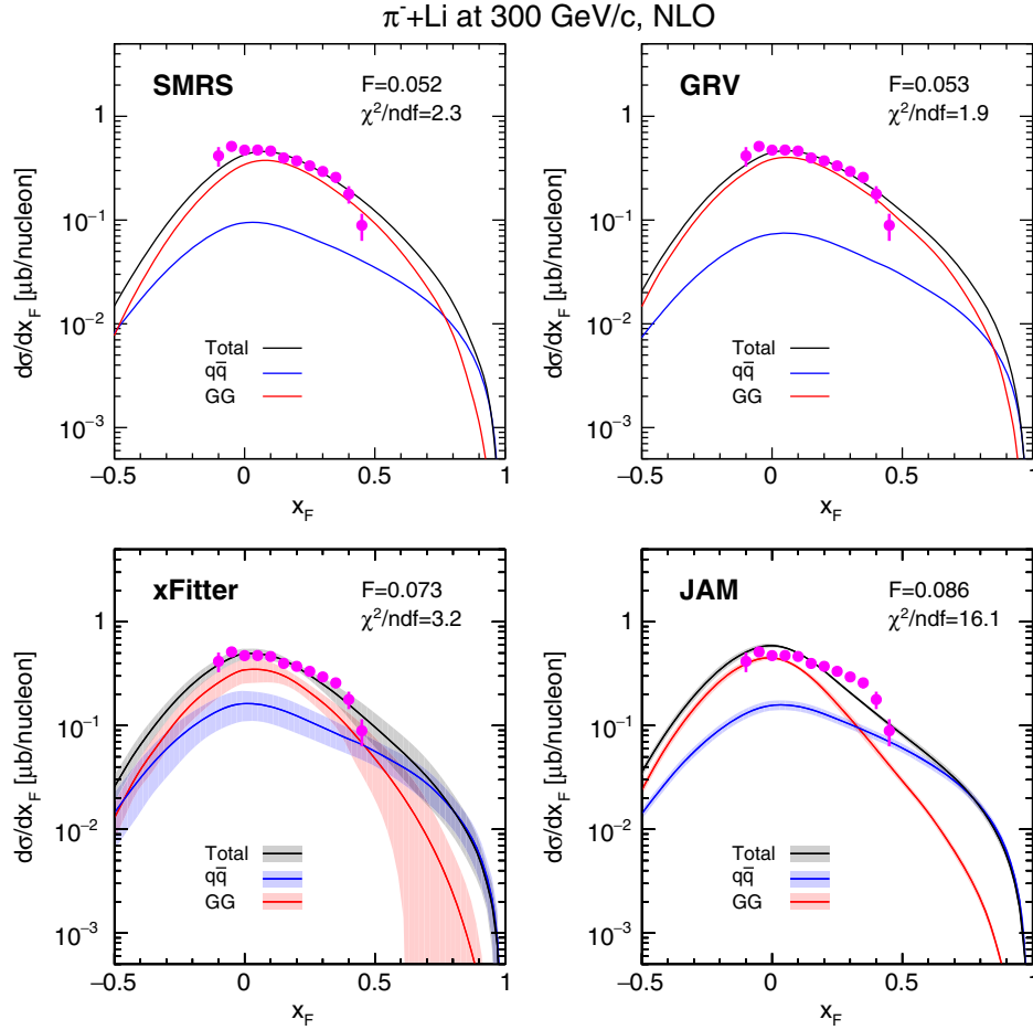
FIG. 4. Comparison of the NLO CEM results for the SMRS, GRV, xFitter, and JAM PDFs with d\sigma/dx_F data of J/\psi production off the lithium target with a 300-GeV/c \pi^- beam from the E705 experiment [69]. The total cross sections and q\bar{q} and GG contributions are denoted as black, blue, and red lines, respectively.
