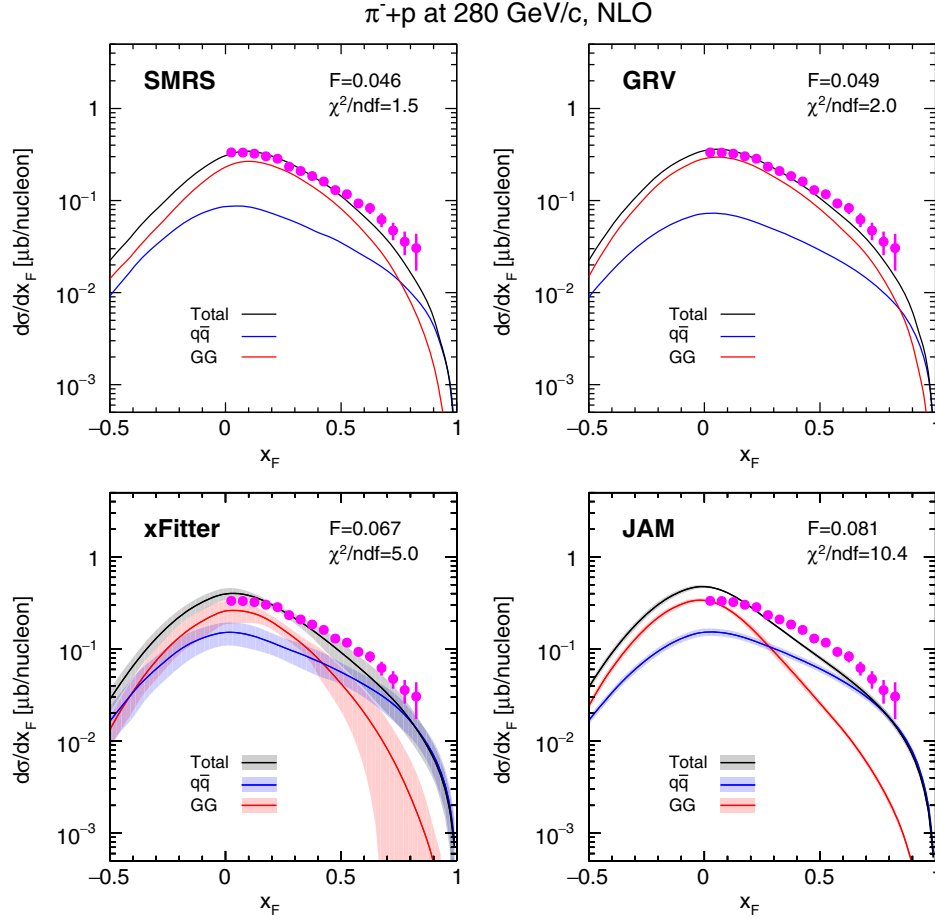
FIG. 5. Comparison of the NLO CEM results for the SMRS, GRV, xFitter, and JAM PDFs, with the d\sigma/dx_F data of J/\psi production off the hydrogen target with a 280-GeV/c \pi^- beam from the NA3 experiment [70]. The total cross sections and q\bar{q} and GG contributions are denoted as black, blue, and red lines, respectively.
