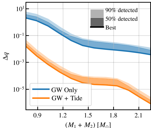
FIG. 7. Uncertainties in inferring the mass ratio, \Delta q , for WD binaries with different total masses.
