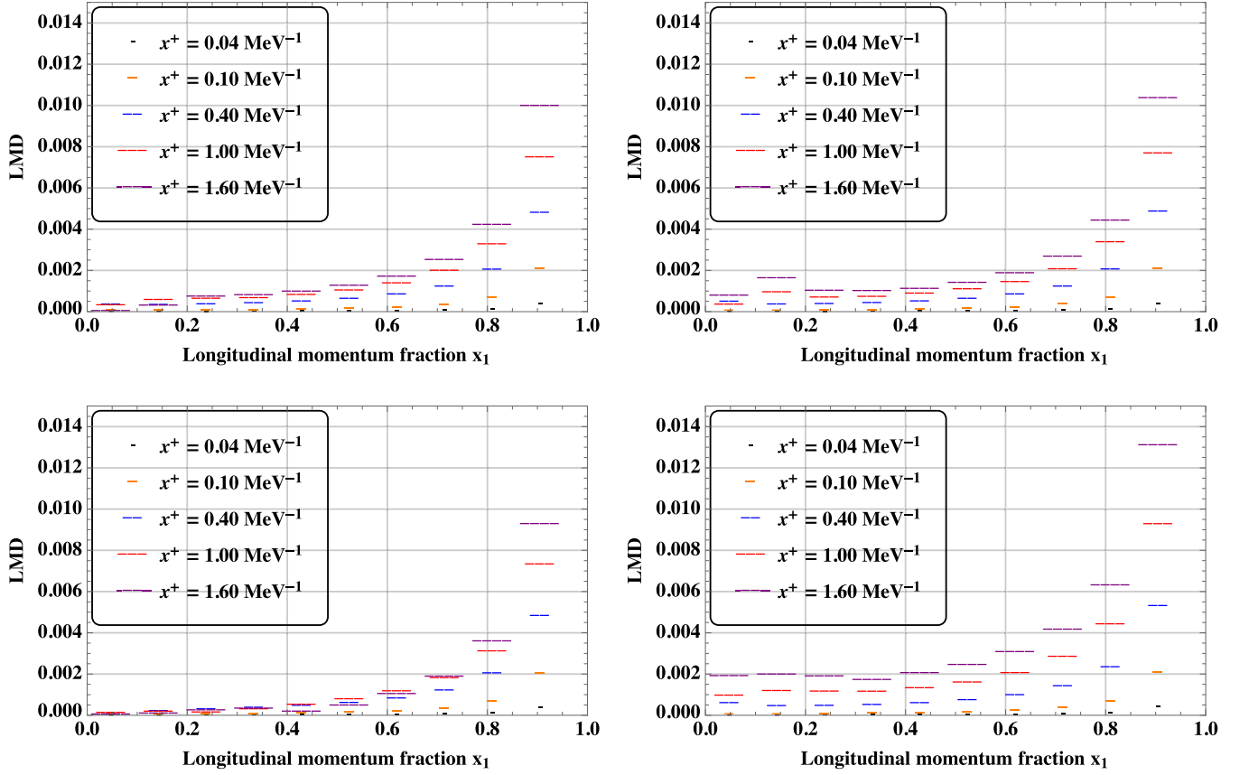
FIG. 10. Time-evolution of the LMD. In all plots, N_{\max} = 100 , K_{\text{total}} = 10.5 , b_l = m_e . In the left-hand column, a_0 = -200 ; in the right-hand column a_0 = 200 . Longitudinal momentum P^+ decreases from P^+ = 10.5 MeV to P^+ = 1.05 MeV as we move from the upper to the lower row. In all the panels the distributions continue to increase with time at almost every electron longitudinal momentum fraction x_1 . In the left column (attractive field), as P^+ decreases, the smaller x_1 excitations decrease. Contrastingly, in the right column (repulsive field), the smaller x_1 excitations increase as P^+ decreases.
