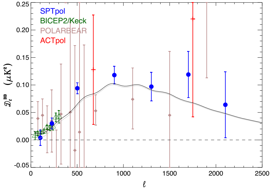
FIG. 2. The B -mode bandpowers from the minimum variance combination of the 95 \times 95 , 95 \times 150 , and 150 \times 150 GHz bandpowers in this work (blue circles) along with the B -mode measurements from other experiments. The 150 GHz results for BICEP2/Keck [6] are shown by the green triangles. ACTpol results at 150 GHz [2] are marked by the red crosses, and POLARBEAR measurements at 150 GHz [13,14] by the rosy brown diamonds. The grey line shows the prediction for lensed B -mode power for the PLANCK best-fit model, while the black line adds on the best-fit Galactic dust power from BICEP2 Collaboration et al. [6]. The B -mode bandpowers from this work are the most precise measurements at \ell > 320 .
