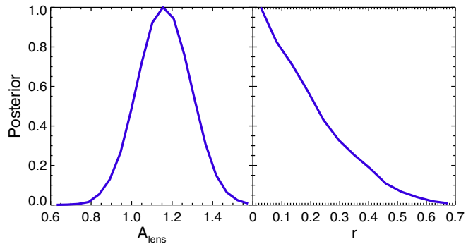
FIG. 3. The measured B -mode power spectrum is consistent with the Planck best-fit \Lambda\text{CDM} model. On the left, we show the posterior probability for A_{\text{lens}} ( A_{\text{lens}} rescales the predicted B -modes due to lensing), finding it consistent with unity. In the right panel, we show that the posterior probability for the tensor-to-scalar ratio r peaks at zero.
