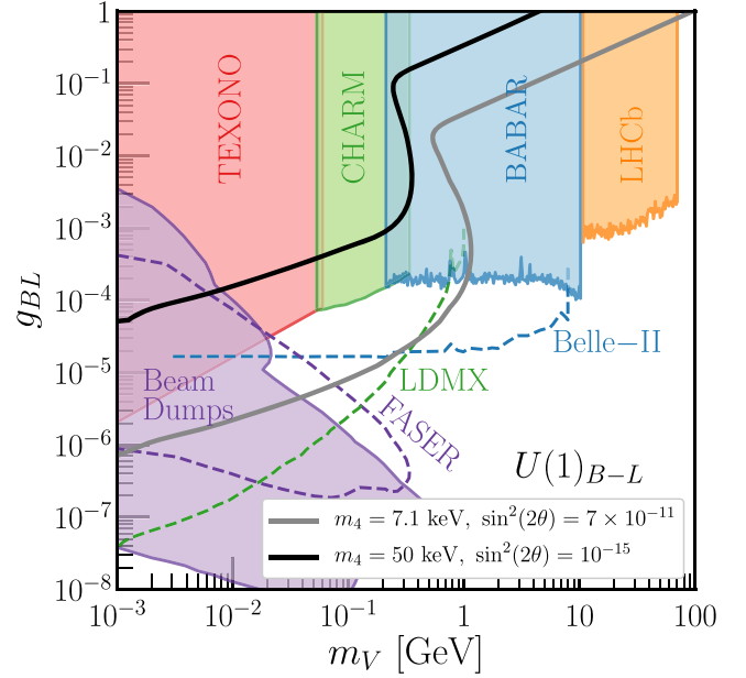
FIG. 8. Curves on the parameter space that yield the observed relic density of dark matter today for the B-L vector boson model and m_4 = 7.1 \text{ keV} , \sin^2(2\theta) = 7 \times 10^{-11} (gray) and m_4 = 50 \text{ keV} , \sin^2(2\theta) = 10^{-15} (black). Existing limits from a variety of probes are shown as filled colored regions: TEXONO (red), CHARM (green), BABAR (blue), LHCb (orange), and a set of beam dump experiments (purple). Future constraints from Belle-II (blue), LDMX (green), and FASER (purple) are shown as dashed lines.
