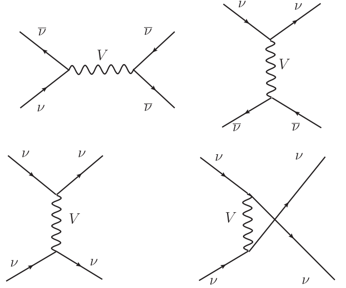
FIG. 3. Scattering diagrams contributing to \Gamma_V . The top panel represents the contribution to the \nu \bar{\nu} \rightarrow \nu \bar{\nu} channel, whereas the bottom panel shows the contribution to the \nu \nu \rightarrow \nu \nu . For m_V \lesssim T , the leading diagram is that of \nu_\mu \bar{\nu}_\mu \rightarrow \nu_\mu \bar{\nu}_\mu with an on-shell V exchange.
