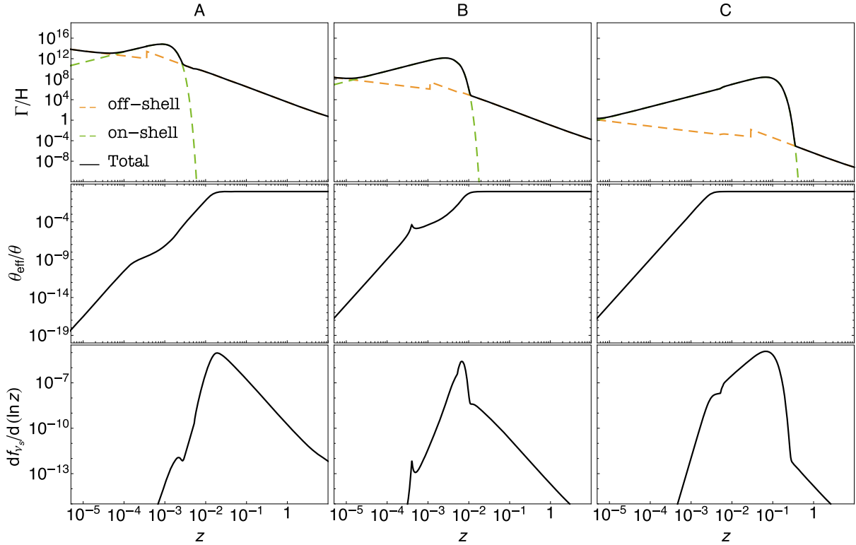
FIG. 5. The variation of the new thermal scattering rate as compared to the Hubble parameter (top), the ratio of the effective mixing angle to the vacuum angle (middle), and the differential sterile neutrino production rate (bottom) as a function of z for the three benchmark points A, B, and C, as chosen in Fig. 4.
