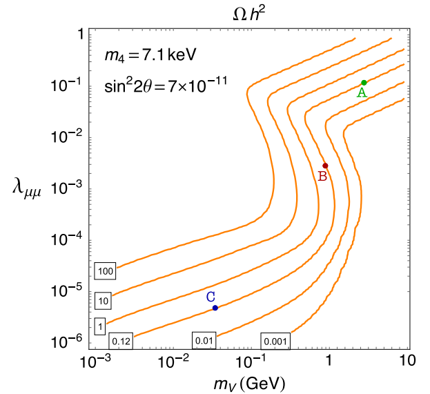
FIG. 4. Contours of \Omega h^2 for m_4 = 7.1 keV, \sin^2 2\theta = 7 \times 10^{-11} , showing regions of over- and underabundance. The values of the relic density are labeled on the contours. Three benchmark points on the contour corresponding to the observed relic density are chosen: A ( \lambda_{\mu\mu} = 0.11 , m_V = 2.77 GeV), B ( \lambda_{\mu\mu} = 0.003 , m_V = 0.88 GeV), and C ( \lambda_{\mu\mu} = 4.8 \times 10^{-6} , m_V = 0.03 GeV).
