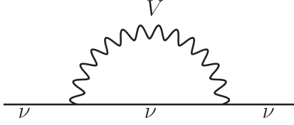
FIG. 2. Loop contribution of the new interaction to the active-neutrino thermal potential V_T .
