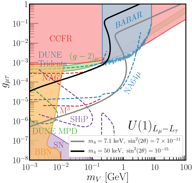
FIG. 7. Curves on the parameter space that yield the observed relic density of dark matter today for the L_\mu - L_\tau vector boson model and m_4 = 7.1 keV, \sin^2(2\theta) = 7 \times 10^{-11} (gray) and m_4 = 50 keV, \sin^2(2\theta) = 10^{-15} (black). Existing limits from a variety of probes are shown as shaded regions: neutrino trident scattering with CCFR (red), BABAR (blue), BBN (orange), and Supernova 1987A (purple). The green filled region corresponds to the preferred region for the (g-2)_\mu anomaly. Future constraints from NA62 (red), NA64 \mu (blue), SHiP (purple), M^3 (red), and DUNE (green for MPD decays and blue for Trident scattering) are shown as dashed lines.
