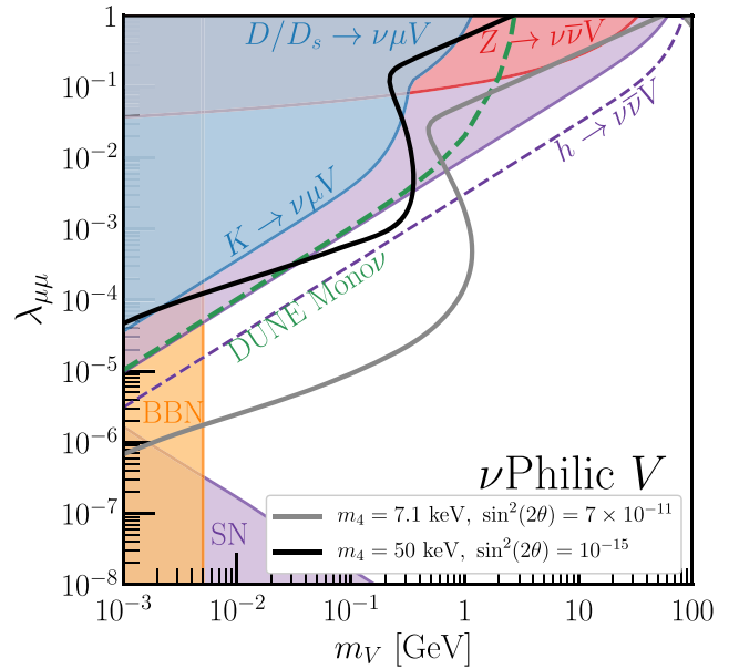
FIG. 6. Curves on the parameter space that yield the observed relic density of dark matter today for the neutrinophilic vector boson model and m_4 = 7.1 keV, \sin^2(2\theta) = 7 \times 10^{-11} (gray), and m_4 = 50 keV, \sin^2(2\theta) = 10^{-15} (black). Existing limits from a variety of probes are shown as filled colored regions: rare meson decays (blue), invisible Z boson decay (red), invisible Higgs boson decay (purple), BBN (orange), and Supernova 1987A (purple). Future constraints from DUNE (green) and the high-luminosity LHC for invisible Higgs boson decay (purple) are shown as dashed lines.
