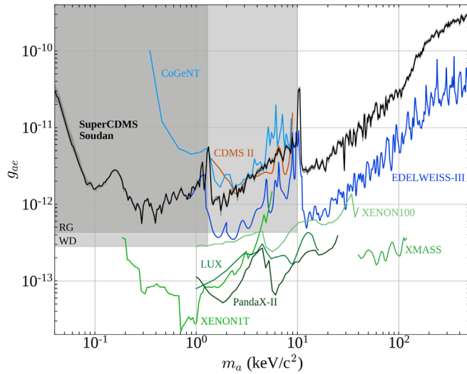
FIG. 9. SuperCDMS Soudan upper limit (solid black) with uncertainty band (shaded grey) on the axioelectric coupling. Also shown are limits set by other direct-detection experiments including: CDMS II [56], CoGeNT [57], EDELWEISS-III [25], LUX [58], PandaX-II [32], XENON100 [59], XENON1T [60], and XMASS [26]. The shaded regions are excluded by the observed cooling of red giant (RG) [61,62] and white dwarf (WD) stars [11,62].
