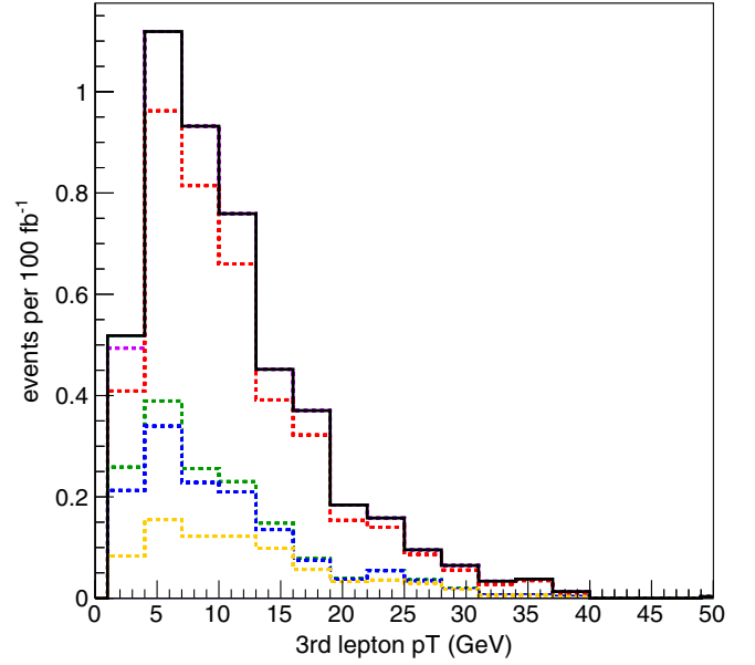
FIG. 5. The p_T of the third hardest lepton in simulated events that pass the ATLAS analysis. The dotted lines indicate the contributions from (starting from the bottom) pp \rightarrow \chi_1^0 \chi_2^0 (yellow), \chi_1^0 \chi_1^+ (blue), \chi_1^0 \chi_1^- (green), \chi_2^0 \chi_1^+ (red), \chi_2^0 \chi_1^- (violet), and \chi_1^- \chi_1^+ (cyan). The black line shows the sum of all contributions.
