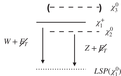
FIG. 1. Schematic spectrum that will have W^\pm Z^0 + \cancel{E}_T as discovery channel. The number of neutralinos depends on the nature (wino or higgsino-like) of \chi_{2,3}^0 .
