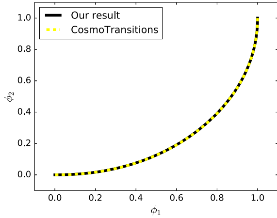
FIG. 6. The same bounce solution as Fig. 5 in the \phi_1 - \phi_2 plane.
