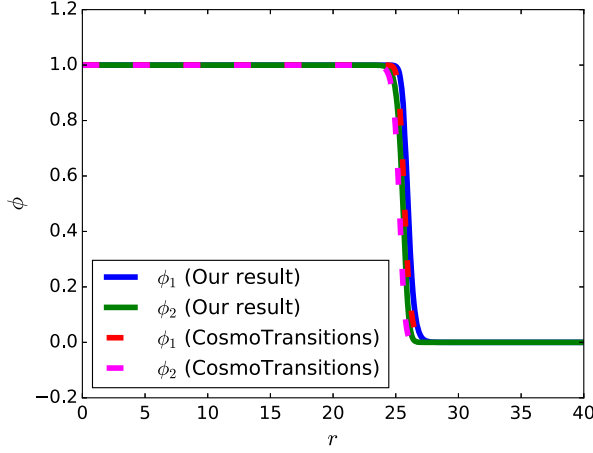
FIG. 5. The bounce solution in the r - \phi plane is shown by solid lines. The dashed lines are results of CosmoTransitions. We take the potential [Eq. (18)] with c = 2 in d = 4 space.
