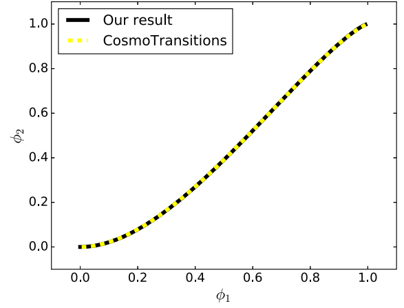
FIG. 8. The same bounce solution as Fig. 7 in the \phi_1 - \phi_2 plane.
