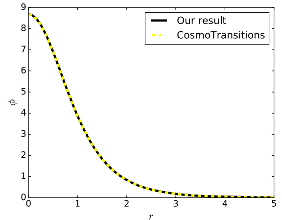
FIG. 4. The black line is obtained from Eq. (15) in the limit of large \tau . The yellow dotted line is calculated by CosmoTransitions.
