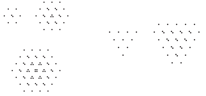
FIG. 2. I_3 , Y plots for some of the SU(3) multiplets which appear in the decomposition of 8 \otimes 8 \otimes 8 . The left-hand plot illustrates the octet, 27-plet and 64-plet representations (clockwise). The right-hand plot shows the 10- and 35-plets (left to right). The number of spots in the central location gives the number of flavor-conserving operators in each multiplet.
