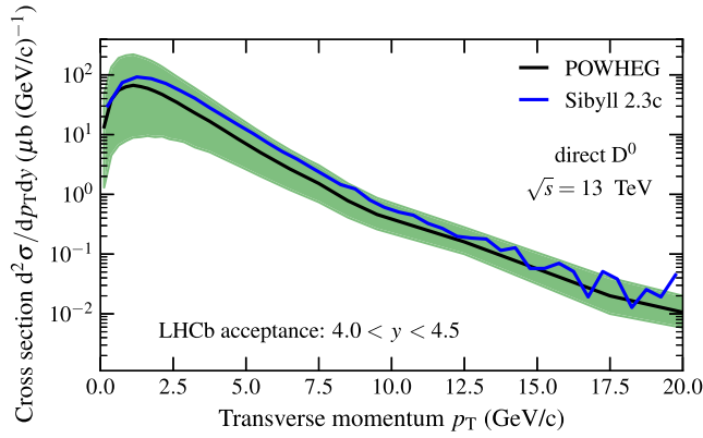
FIG. 25. p_T -spectrum of neutral D-mesons at \sqrt{s} = 13 TeV. Compared are SIBYLL and a NLO QCD calculation (POWHEG) [65]. The band of the theory calculation corresponds to charm quark mass and factorization scale uncertainty. The central phase space covered by the LHCb acceptance is dominated by perturbative processes, such that the full prediction by SIBYLL can be compared to the pQCD calculation.
