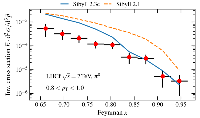
FIG. 15. Longitudinal momentum spectrum of the of neutral pions at 7 TeV. Data are from the LHCf spectrometer, covering 8.9 < \eta < 10.2 in two different p_T bins.
