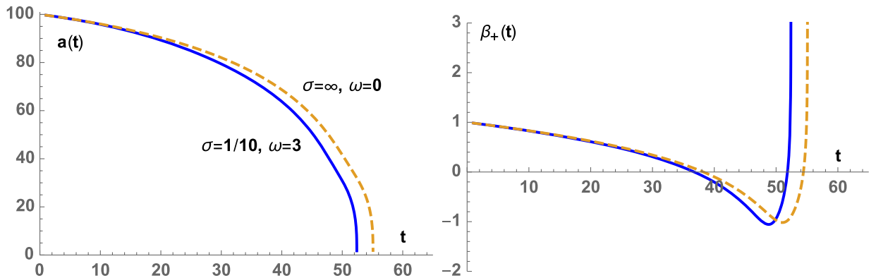
FIG. 1. Plots of the scale factor (left) and the anisotropy (right) as a function of time, for a typical example of the approach to a singularity. The dashed curves show the solution in the absence of quadratic gravity terms, where one can see that after one reflection of the anisotropy parameter, a singularity is reached at a finite time. When quadratic curvature terms are added, the only effect is to accelerate the occurrence of the crunch, as seen in the continuous curves. The initial conditions used here for the two-derivative theory are a(t=0) = 100 , \dot{a}(0) = -1/3 , \beta_+(0) = 1 . For the case with higher-derivative terms added, we fix the additional initial data by using the two-derivative solution, and we check that the constraint remains satisfied to sufficient accuracy.
