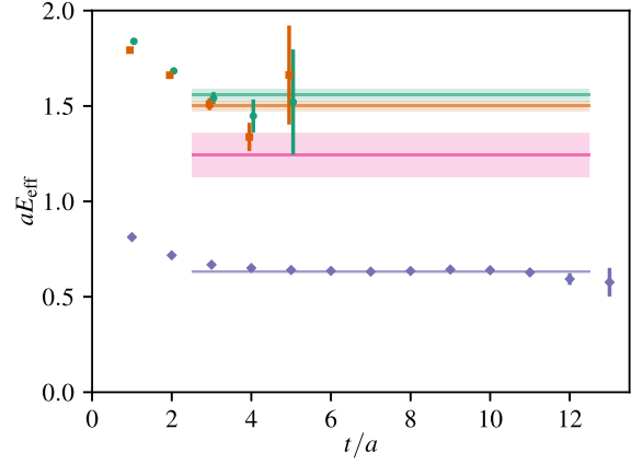
FIG. 3. Effective energies for the three GEVP-projected correlators at zero momentum (in order of increasing energy: blue diamonds, orange squares, and green circles) and energies from the four-state fit (horizontal bands). The colors of the bands correspond to the effective energy with which they are identified in Sec. III A; the additional state has a magenta band. The horizontal range of the bands indicates the time separations in the two-point correlator matrix that are fitted.
