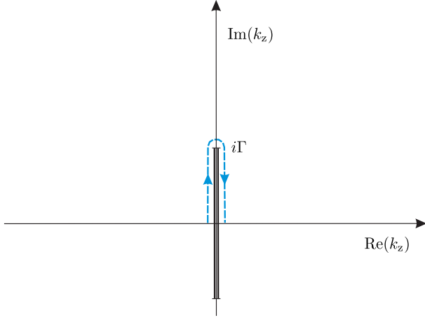
FIG. 1. The dashed line represents the contour \mathcal{C} used to evaluate the k_z -integral in Eq. (39).
