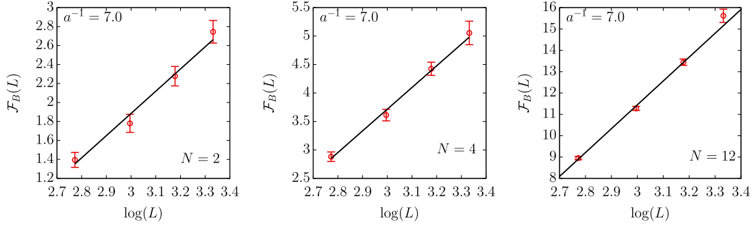
FIG. 3. Determination of monopole naive dimension d(L) as determined in the range of L = 16, 20, 24 and 28 by a linear fit of \mathcal{F}_B at fixed lattice spacing corresponding to a = \frac{1}{7} to an effective \log(L) dependence over the range of L considered. The three panels from left to right correspond to N = 2, 4 and 12 , respectively.
