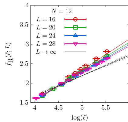
FIG. 6. The large- \ell behavior of f_R for N = 12 is shown. The different colored symbols are for different L . The solid straight lines are from combined fits of the form f_R(\ell) = \alpha_0 + \alpha_1/L + 2(\beta_0 + \beta_1/L) \log(\ell) to the data at L = 16, 20, 24, 28 from \ell = 64 to 250 . The black straight line and band are the estimates for the L \rightarrow \infty continuum limit. The estimate for \beta_0 is 0.26(2) , and can be identified with \Delta(12)/12 .
