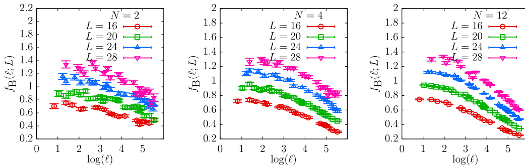
FIG. 2. The bare free energy per fermion degree of freedom, f_{\text{B}} = \mathcal{F}_{\text{B}}/N , of the lattice monopole-antimonopole background field insertion is shown as a function of the physical extent of the box \ell . The three panels from left to right correspond to N = 2, 4 and 12 , respectively. The different colored symbols correspond to different L specified in the key.
