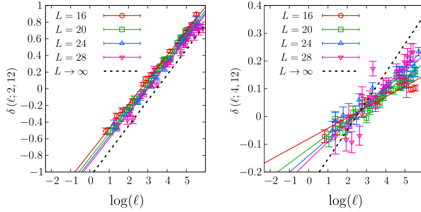
FIG. 5. The difference \delta(\ell; N, N' = 12) = f_R(\ell; N) - f_R(\ell; N' = 12) is shown as a function of \ell for N = 2 and 4 in the left and right panels, respectively. The solid lines are the combined fits to the form \delta(\ell; N, 12) = a_0 + a_1/L + 2(b_0 + b_1/L) \log(\ell) . The dashed line is the central value of the estimated continuum limit, L \rightarrow \infty , of this difference. The positive slope, both in the data and in the estimated continuum limit, clearly indicates that N = 2 and N = 4 have larger infrared scaling dimension than that of N = 12 .
