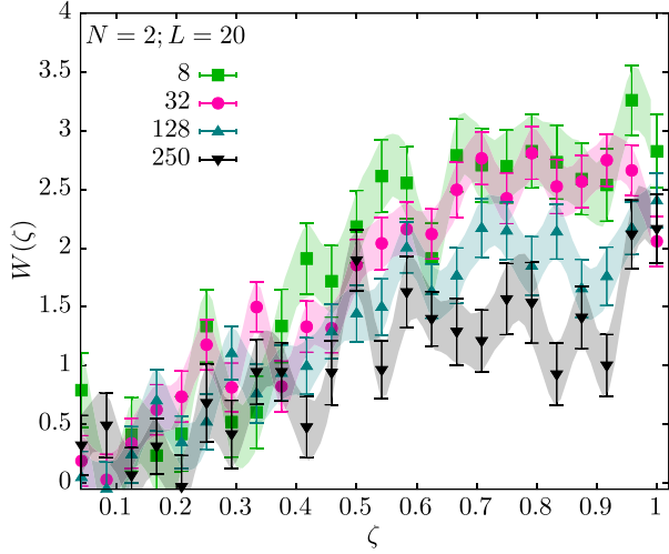
FIG. 1. W(\zeta) is shown as a function of \zeta at different values of \ell at fixed L = 20 for the case of N = 2 flavors. The different colored symbols correspond to different physical extents \ell , and the bands are the cubic spline interpolation of the data points. The free energy for the Q = 1 monopole-antimonopole pair is given by the area under the curves, \int_0^1 W(\zeta) d\zeta .
