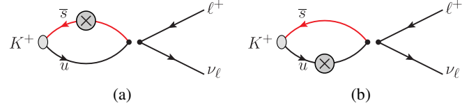
FIG. 4. Connected diagrams contributing at \mathcal{O}(\alpha_{\text{em}}) and \mathcal{O}(m_d - m_u) to the K^+ \rightarrow \ell^+ \nu_\ell decay amplitude related to the insertion of the scalar density (see Ref. [8]).
