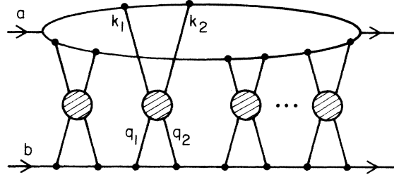
FIG. 4. Same as Fig. 3 except that the ladder only links one fragment of a to particle b .
