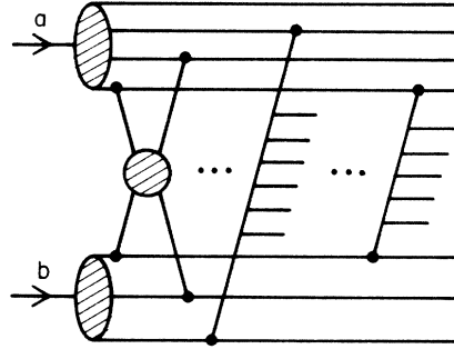
FIG. 2. A typical inelastic amplitude studied in this paper.
