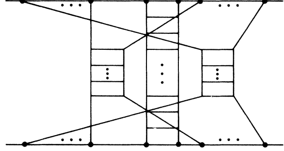
FIG. 9. The generalized Mandelstam diagrams, also known as the "nested diagrams," studied in Ref. 9.
