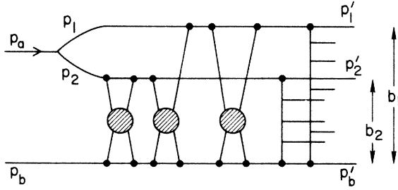
FIG. 8. Production processes associated with Figs. 3 and 4.
