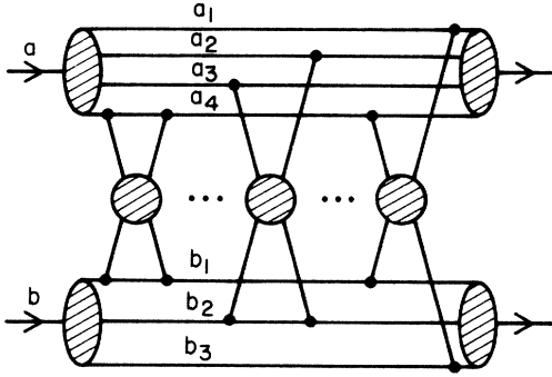
FIG. 1. The elastic amplitude studied in this paper. The lines labeled a_1, \dots, a_n ( b_1, \dots, b_m ) represent the fragments of particle a (particle b ). The blobs exchanged between a and b are t -channel ladders.
