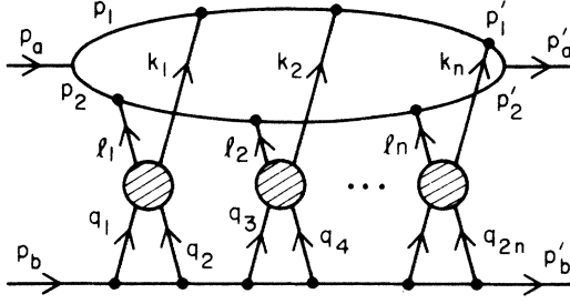
FIG. 3. Example of elastic amplitude with two fragments in particle a and no fragmentation in particle b . The ladders link all 3 lines.
