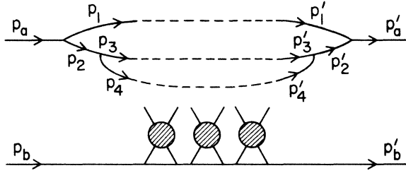
FIG. 5. Elastic amplitude with three fragments in particle a and no fragmentation in particle b .
