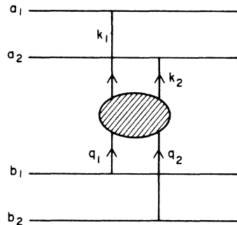
FIG. 7. Ladder-exchange which leads to four-body eikonal function (i.e., four-body potential).
