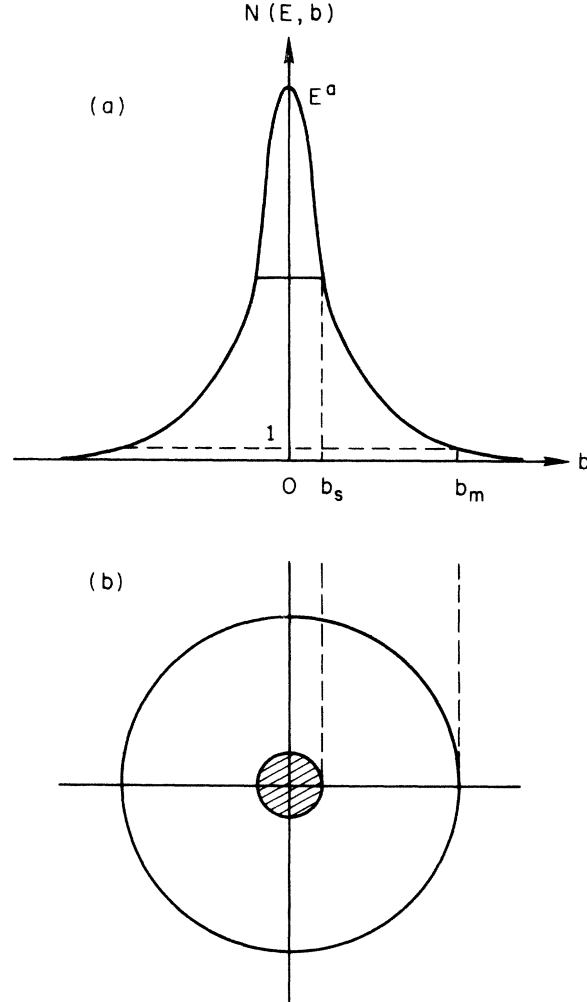
FIG. 10. (a) Multiplicity distribution in b space; (b) two relevant radii b_s (half-width) and b_m (maximal size) obtained from the distribution curve.
