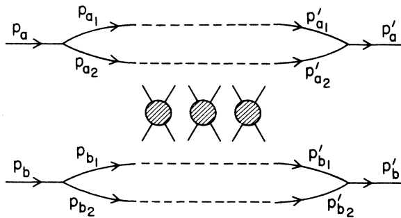
FIG. 6. Elastic amplitude with two fragments each in particle a and b .
