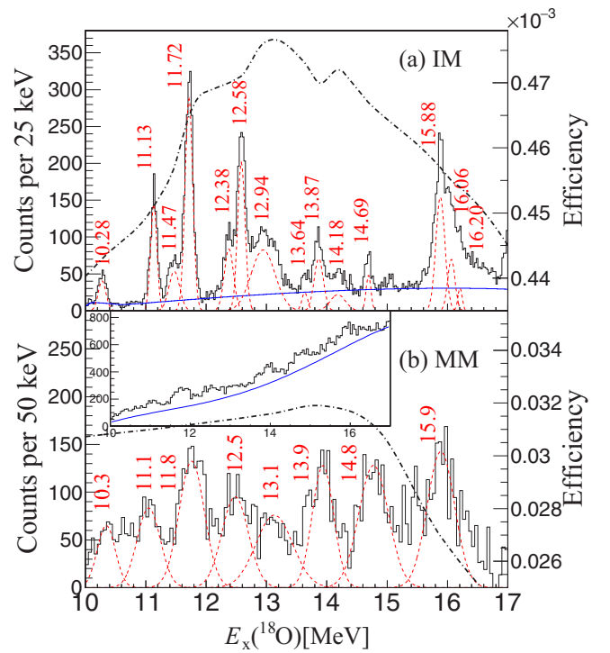
FIG. 6. (a) The invariant-mass spectrum reconstructed from ^{18}\text{O}^* \rightarrow ^{14}\text{C} + \alpha decay [using events with detected 2- \alpha (by L0 + R0) and deduced ^{14}\text{C} ], in comparison to (b) the corresponding missing-mass spectrum using events with detected recoil \alpha -particles. Each spectrum is fitted by a number of Gaussian-function peaks (red dashed lines) plus a smooth background (the blue solid line). For a better view of the peak, the structure built on the large background as exhibited in the inset of panel (b), the inclusive missing-mass spectrum is plotted with the background subtracted. In both cases, the black dot-dashed lines show the simulated experimental detection efficiency.
