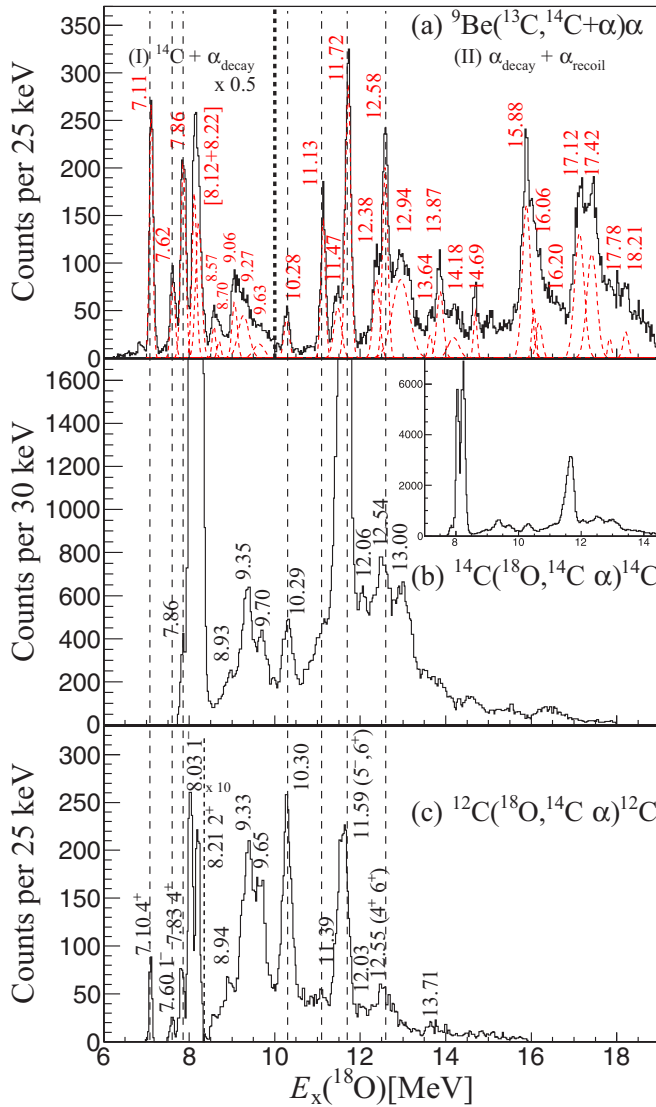
FIG. 5. (a) Excitation-energy spectrum of ^{18}\text{O} obtained from the present experiment. States below 10 MeV are reconstructed from events with detected ^{14}\text{C} + \alpha fragments from the same telescope (L0 or R0), while states between 10 and 19 MeV are from events with detected two- \alpha (and deduced ^{14}\text{C} ) fragments from L0 + R0 telescopes. These resonances are compared with the previous results: (b) from Ref. [28] and (c) from Ref. [26].
