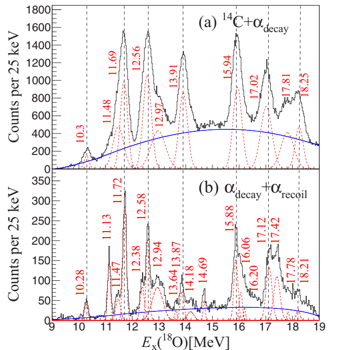
FIG. 4. ^{18}\text{O}^* excitation-energy spectra from (a) events with detected ^{14}\text{C} + \alpha and (b) events with detected \alpha + \alpha . Peaks in each spectrum are fitted by a number of Gaussian functions (red dotted lines) plus a continuous background (the blue smooth line).
