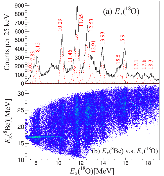
FIG. 7. (a) Excitation-energy spectrum for ^{18}\text{O} , reconstructed from events with one \alpha -particle detected by the L0/R0 telescope while another is detected by the R2/L2 telescope. (b) Dalitz-type two-dimensional excitation-energy spectrum for reconstructed ^8\text{Be} (from 2\text{-}\alpha ) versus ^{18}\text{O} (from \alpha + ^{14}\text{C}_{\text{deduced}} ).
