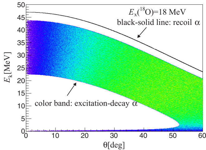
FIG. 2. Relationship between energy and angle (Lab) for the recoil \alpha -particles (the black solid line) and for the decay \alpha -particles originated from excited ^{18}\text{O} (18 MeV) (the color band).
