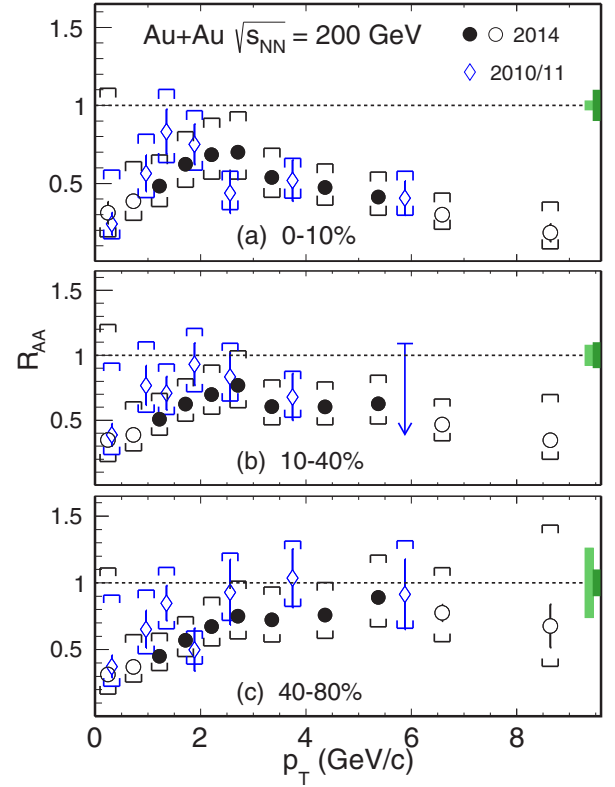
FIG. 31. D^0 R_{AA} in Au + Au collisions at \sqrt{s_{NN}} = 200 GeV for 0–10% (a), 10–40% (b), and 40–80% (c) centrality bins, respectively. The first two and last two data points are presented as empty circles, indicating that the p + p reference is extrapolated into these p_T ranges. The statistical and systematic uncertainties are shown as error bars and brackets on the data points. The light and dark green boxes on the right depict the normalization uncertainties in determining the N_{bin} in Au + Au collisions and the total inelastic cross section in p + p collisions, respectively.
