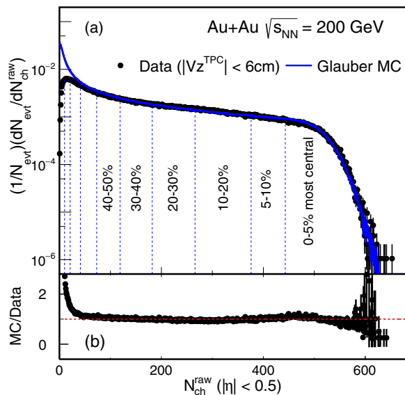
FIG. 1. (a) Uncorrected charged particle multiplicity N_{\text{ch}}^{\text{raw}} distribution measured within |\eta| < 0.5 and |V_z^{\text{TPC}}| < 6 cm. The solid curve depicts the multiplicity distribution from a MC Glauber simulation fit to the experimental data. (b) Ratio between MC simulation and real data.
