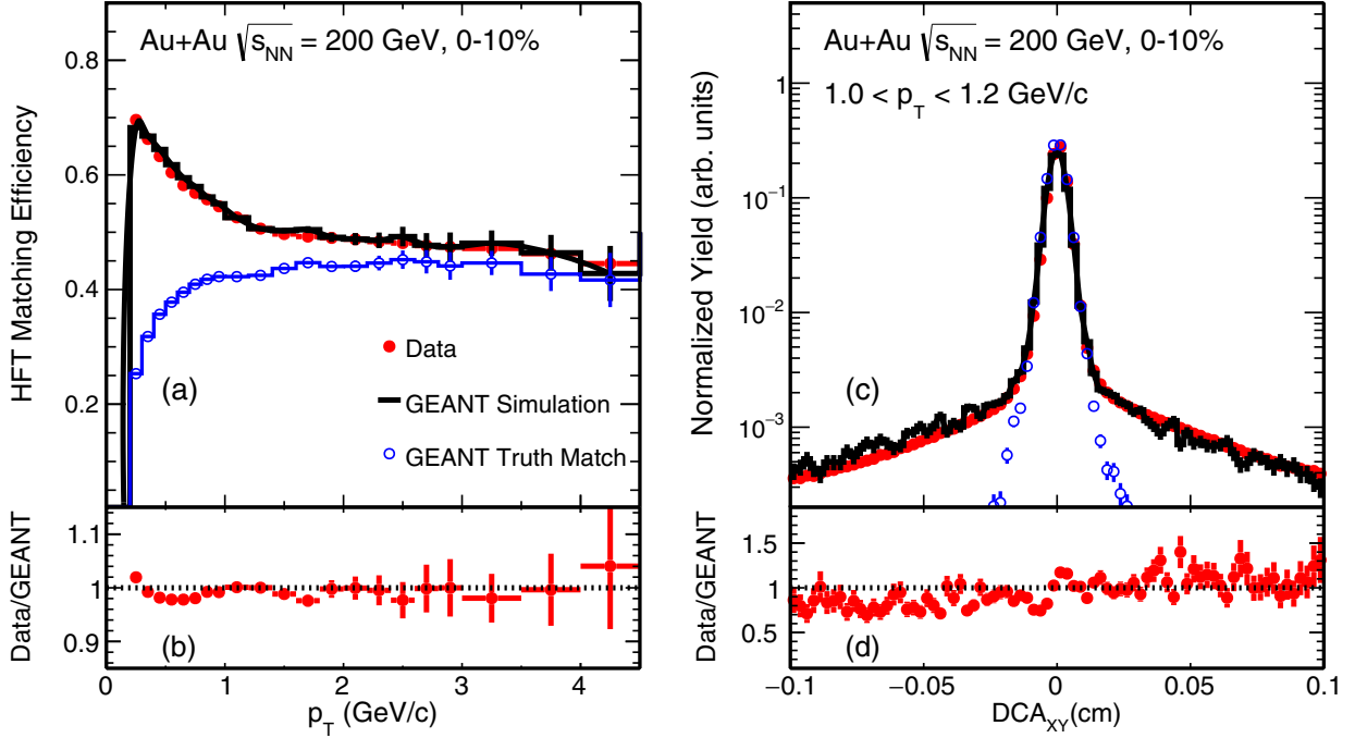
FIG. 10. HFT matching efficiency \varepsilon_{\text{HFT}}^{\text{match}} (a) and \text{DCA}_{XY} (c) distributions of inclusive charged pions from real data and MC simulation in 0–10% Au + Au collisions. The ratios between real data and GEANT simulation are shown in the bottom panels. The blue histogram depicts the true matches for which the reconstructed tracks pick up the correct MC hits in the HFT detector induced by the associated MC tracks in the GEANT simulation.
