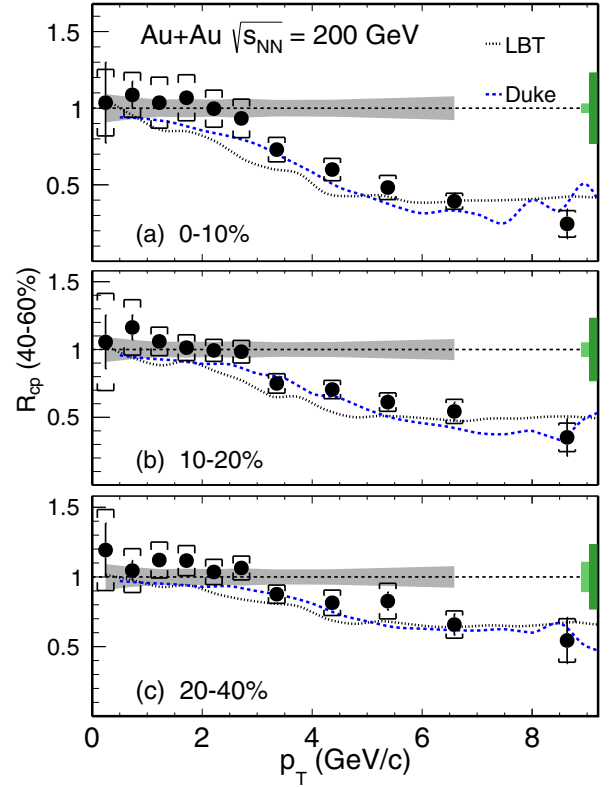
FIG. 36. D^0 R_{CP} with the 40–60% spectrum as the reference for different centrality classes compared to model calculations from LBT (black dotted lines) and the Duke (blue dashed lines) groups [52–54]. Data points shown here are the same as in Fig. 30.
