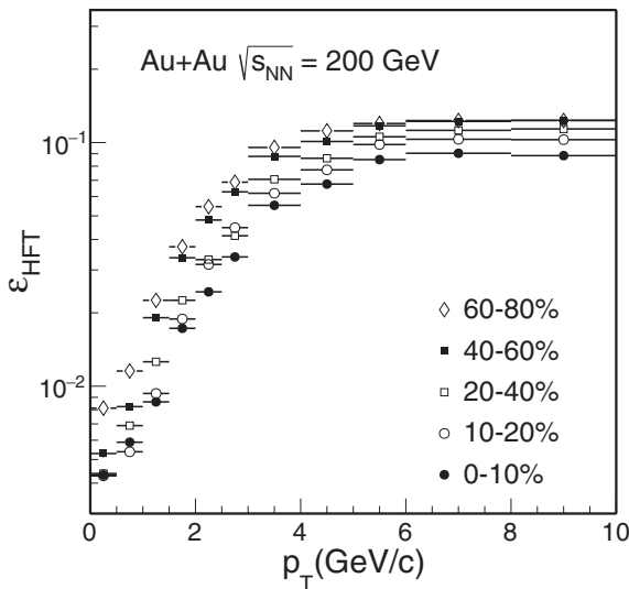
FIG. 14. D^0 HFT tracking and topological cut efficiencies \epsilon_{\text{HFT}} from different centrality classes in Au + Au collisions at \sqrt{s_{\text{NN}}} = 200 \text{ GeV} .
