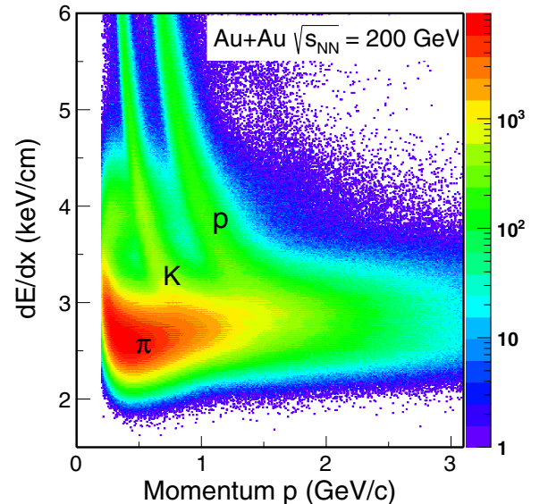
FIG. 3. TPC dE/dx vs particle momentum.
