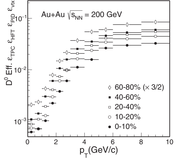
FIG. 21. The total D^0 reconstruction efficiency from different centrality classes.
