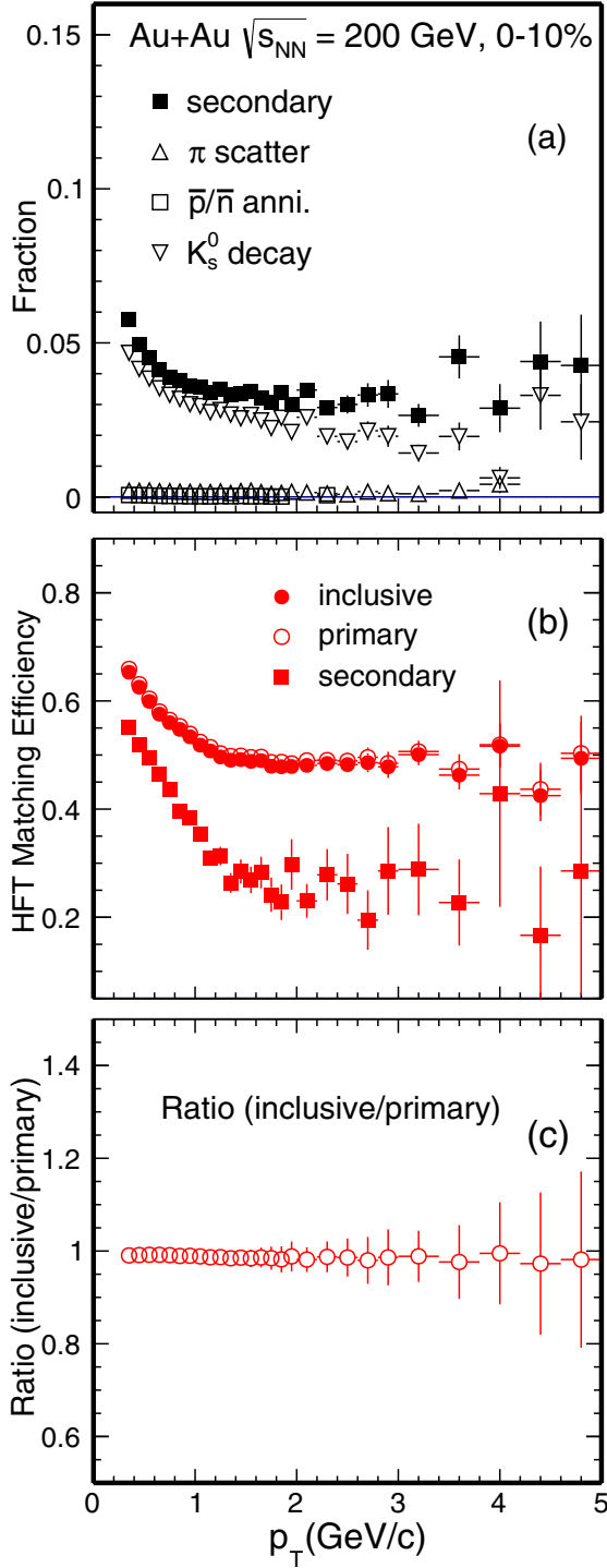
FIG. 15. Secondary pion contribution estimated from HIJING + GEANT simulation with FLUKA hadronic package. Panel (a) shows the fraction of different sources for secondary pion tracks. Panel (b) shows the HFT matching efficiency \varepsilon_{\text{HFT}}^{\text{match}} for inclusive, primary, and secondary pions. Panel (c) shows the ratio of HFT matching efficiencies between inclusive and primary pions.
