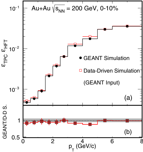
FIG. 12. (a) D^0 reconstruction efficiency comparison between MC GEANT simulation (black) and data-driven fast simulation with reconstructed MC data as the input (red) in central 0–10% Au + Au collisions. (b) The ratio between the two methods. The grey band around unity represents the 5% systematic uncertainties.
