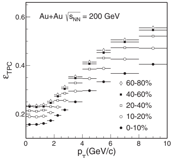
FIG. 9. D^0 TPC acceptance and tracking efficiencies from different centrality classes in Au + Au collisions at \sqrt{s_{\text{NN}}} = 200 GeV.
