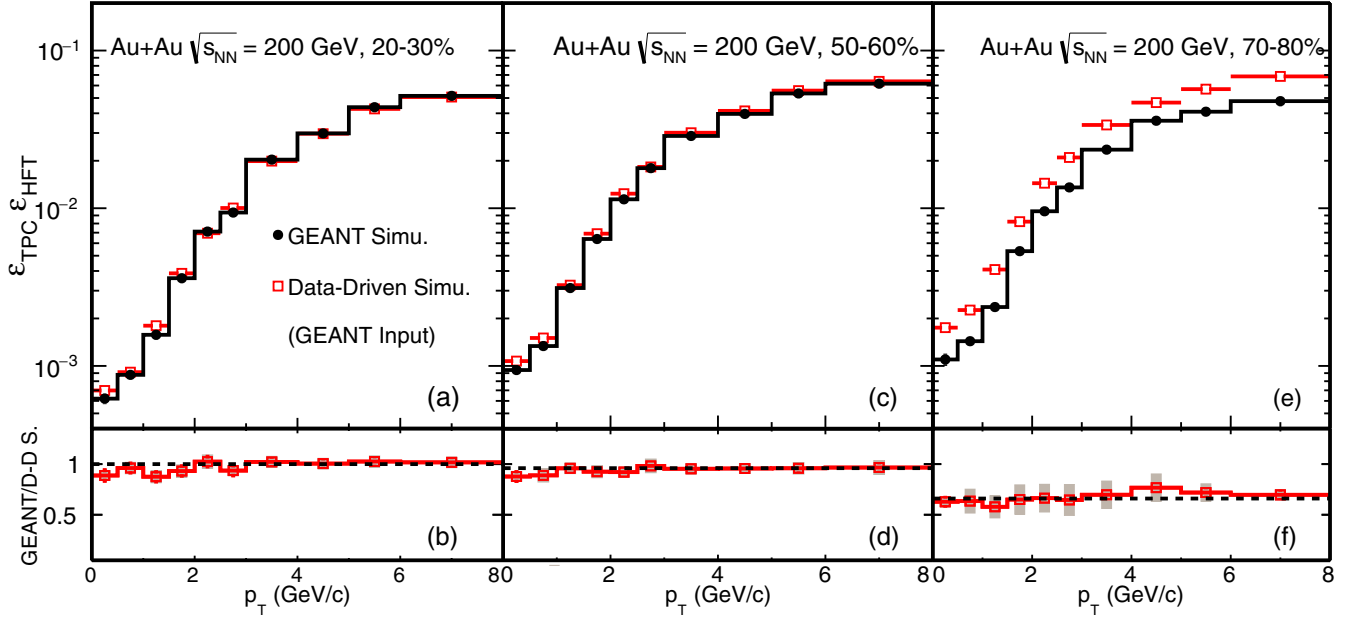
FIG. 17. D^0 reconstruction efficiency comparison between MC GEANT simulation (GEANT, black) and data-driven simulation with the reconstructed MC data as the input (D-D S., red) for 20–30% (a), 50–60% (c), and 70–80% (e) Au + Au collisions. Bottom panels (b), (d), and (f) show the ratios between the two distributions above.
