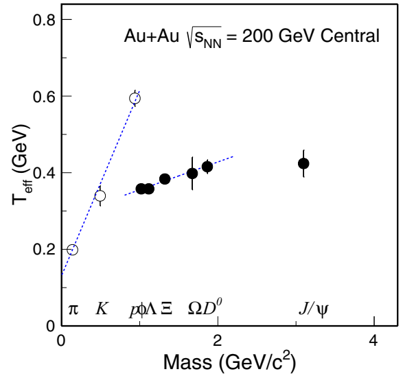
FIG. 26. Slope parameter T_{\text{eff}} for different particles in central Au + Au collisions [29,39–41]. The dashed lines depict linear function fits to \pi , K , p and \phi , \Lambda , \Xi^- , \Omega^- , D^0 respectively.
