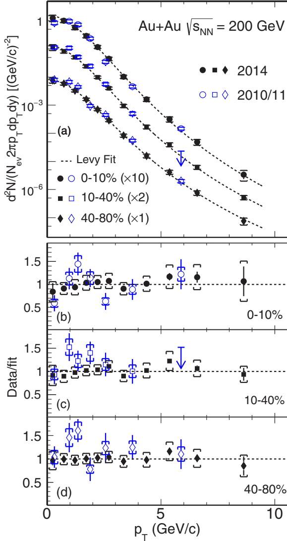
FIG. 23. (a) Measured D^0 spectra from this analysis compared with the previous 2010/11 measurements for different centrality classes. Dashed lines depict Levy function fits to 2014 data. (b)–(d) Ratio of measured spectra to the fitted Levy functions in 0–10%, 10–40%, and 40–80% centrality bins, respectively.
