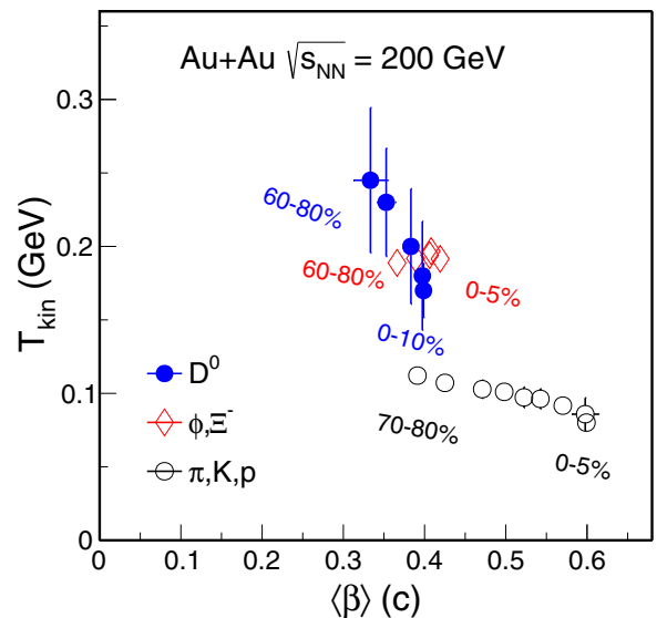
FIG. 28. Results of T_{\text{kin}} vs \langle \beta \rangle from the blast-wave model fits to different groups of particles. The data points for each group of particles present the results from different centrality bins with the most central data point at the largest \langle \beta \rangle .
