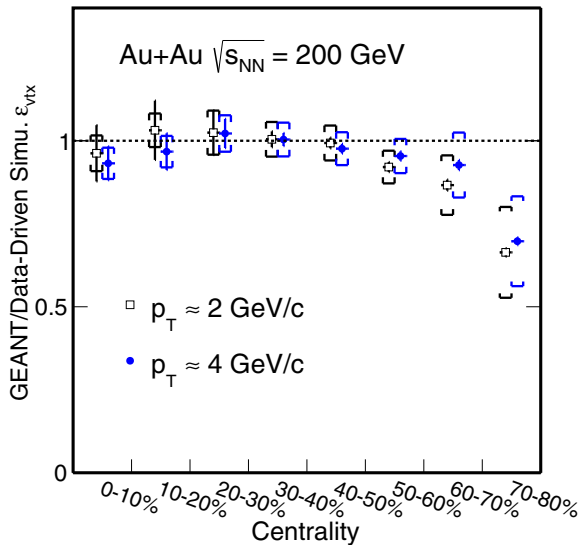
FIG. 18. \varepsilon_{vtx} , D^0 reconstruction efficiency ratios between MC GEANT simulation and data-driven simulation with the reconstructed MC data as the input vs collision centrality for p_T at 2 and 4 GeV/c. The brackets depict the estimated systematic uncertainties.
