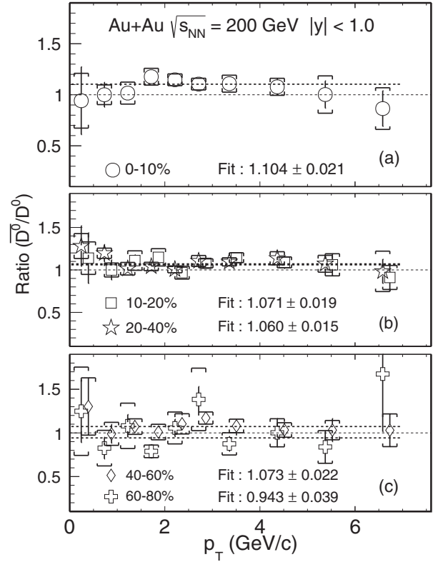
FIG. 34. \bar{D}^0/D^0 invariant yield ratio at mid-rapidity ( |y| < 1 ) vs transverse momentum for different centrality classes. Error bars indicate statistical uncertainties and brackets depict systematic uncertainties. Dashed lines depict constant function fits to the \bar{D}^0/D^0 ratios.
