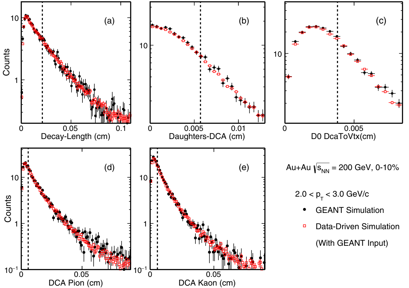
FIG. 11. Comparisons in topological variable distributions between MC GEANT simulation (black) and data-driven fast simulation with reconstructed MC data as the input (red) in 0–10% Au + Au collisions for D^0 mesons at 2 < p_T < 3 GeV/c.
