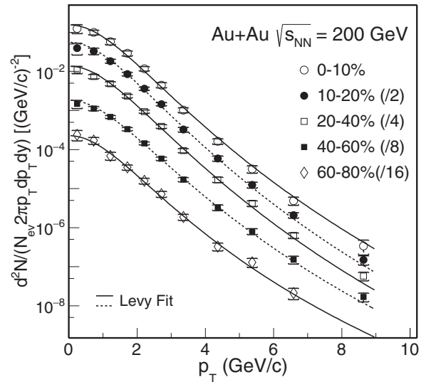
FIG. 22. D^0 invariant yield at mid-rapidity ( |y| < 1 ) vs transverse momentum for different centrality classes. Error bars (not visible for many data points) indicate statistical uncertainties and brackets depict systematic uncertainties. Global systematic uncertainties in B.R. are not plotted. Solid and dashed lines depict Levy function fits.
