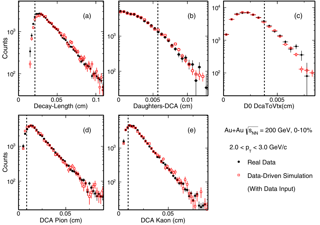
FIG. 13. Comparison of topological variable distributions between D^0 signals in real data (black) and in data-driven simulation with real data distributions as the input (red) in 0–10% Au + Au collisions for D^0 mesons at 2 < p_T < 3 \text{ GeV}/c . The dashed lines indicate the final topological cuts chosen for each individual topological variable.
