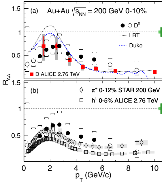
FIG. 32. D^0 R_{AA} in 0–10% Au + Au collisions at \sqrt{s_{NN}} = 200 GeV compared to the ALICE D -meson result in 0–10% Pb + Pb collisions at \sqrt{s_{NN}} = 2.76 TeV (a) and charged hadrons from ALICE and \pi^\pm from STAR (b). Also shown in panel (a) are the model calculations from the LBT and Duke groups [52–54]. Notations for statistical and systematic uncertainties are the same as in previous figures.
