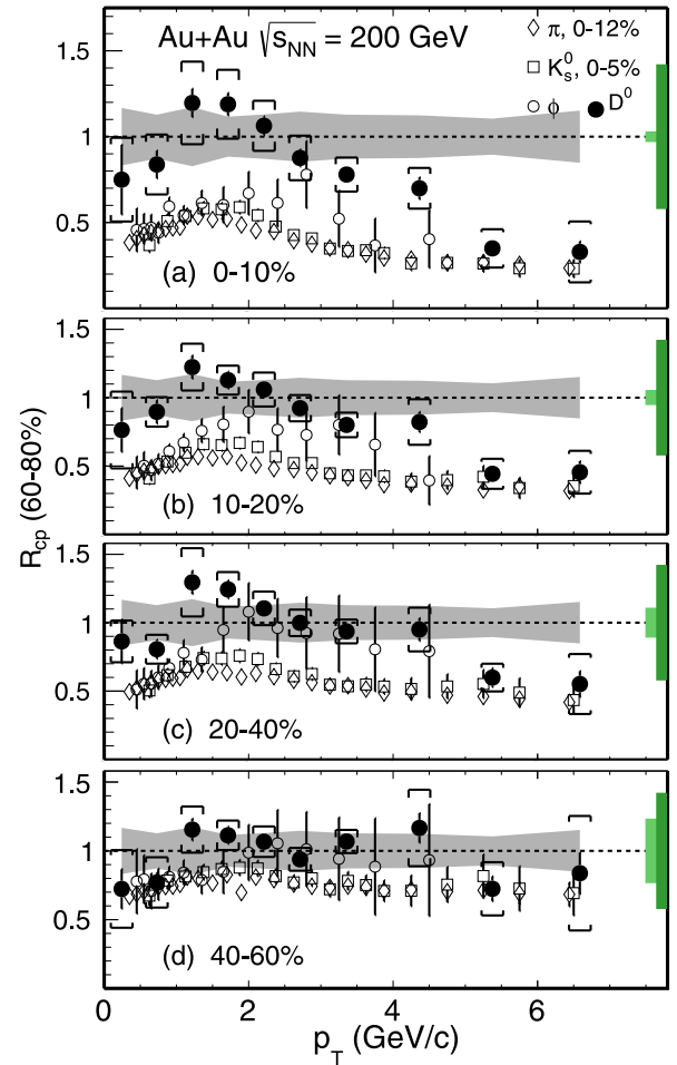
FIG. 29. D^0 R_{\text{CP}} with the 60–80% spectrum as the reference for different centrality classes in Au + Au collisions compared to that of other light and strange mesons ( \pi^\pm , K_s^0 , and \phi ) [48–50]. The statistical and systematic uncertainties are shown as error bars and brackets on the data points. The grey bands around unity depict the systematic uncertainty due to vertex resolution correction, mostly from the 60–80% reference spectrum. The light and dark green boxes on the right depict the normalization uncertainties in determining the N_{\text{bin}} for each centrality (light green) and the 60–80% centrality bin (dark green), respectively.
