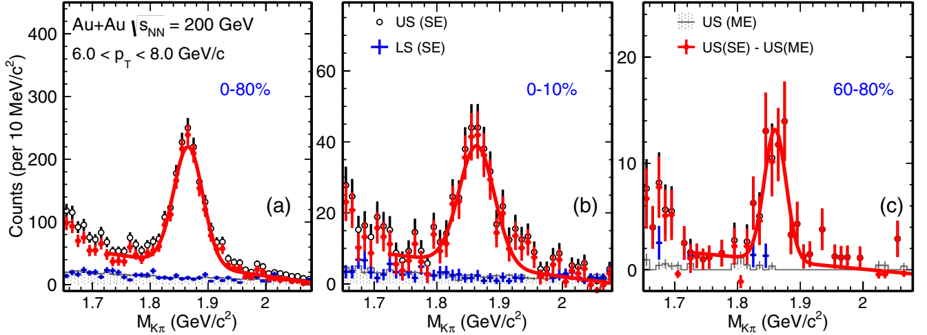
FIG. 8. Invariant mass M_{K\pi} distributions in 6 < p_T < 8 GeV/c from centrality bins 0–80% (a), 0–10% (b), and 60–80% (c), respectively. All histograms and markers use the same notation as in Fig. 6.
