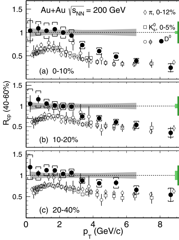
FIG. 30. D^0 R_{CP} with the 40–60% spectrum as the reference for different centrality classes in Au + Au collisions compared to that of other light and strange mesons ( \pi^\pm , K_s^0 , and \phi ) [48–50]. The statistical and systematic uncertainties are shown as error bars and brackets on the data points. The grey bands around unity depict the systematic uncertainty due to vertex resolution correction, mostly from the 40–60% reference spectrum. The light and dark green boxes on the right depict the normalization uncertainties in determining the N_{bin} for each centrality (light green) and the 40–60% centrality bin (dark green), respectively.
