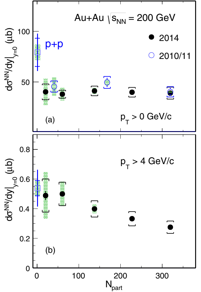
FIG. 24. Integrated D^0 cross section per nucleon-nucleon collision at mid-rapidity for p_T > 0 (a) and p_T > 4 \text{ GeV}/c (b) as a function of centrality N_{part} . The statistical and systematic uncertainties are shown as error bars and brackets on the data points. The green boxes on the data points depict the overall normalization uncertainties in p + p and Au + Au data respectively.
