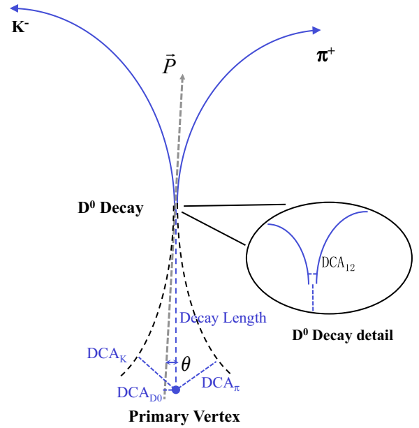
FIG. 5. A cartoon picture for D^0 \rightarrow K^- + \pi^+ decay and definition of topological variables used in the reconstruction.
