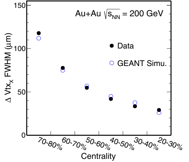
FIG. 16. Full-width at half maximum (FWHM) of vertex position difference in the X dimension between two randomly divided subevents in various centrality bins. Black solid circles present the FWHM values from real data while blue empty circles are from HIJING + GEANT simulation. Statistical uncertainties are smaller than the marker size.
