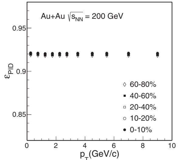
FIG. 19. Particle identification efficiency ( \varepsilon_{PID} ) of D^0 mesons in different centrality classes.
