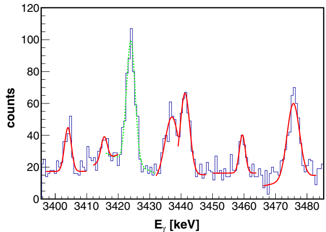
FIG. 8. Partial \gamma -ray energy spectrum illustrating the fit for the 3424.8-keV primary \gamma ray (dashed green curve). Representative fits to neighboring \gamma rays (solid red curves) are presented for comparison.
