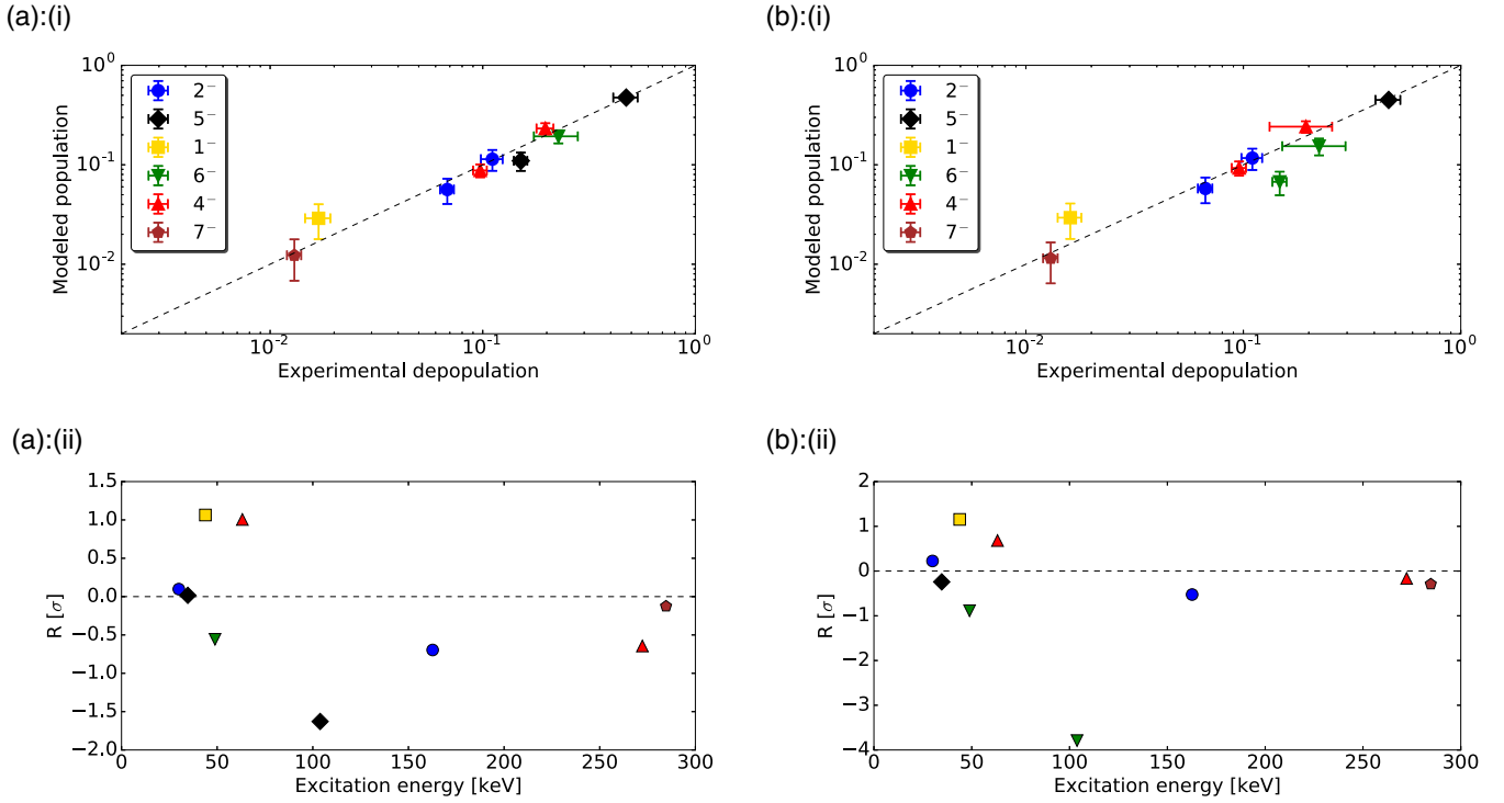
FIG. 7. Upper panels (a):(i) and (b):(i): The simulated population (per neutron capture) of levels below the critical energy of 285 keV vs their experimental depopulation (per neutron capture) assuming using the GLO [56] model for the PSF and the CTF [43,44] model for the LD using the parametrization of Ref. [47]. The J^\pi distribution of the levels is indicated on the plot and a dashed black line of unit slope is drawn for guidance. Lower panels (a):(ii) and (b):(ii): Residuals ( R ) between simulations and experimental data as a function of the excitation energy. The plots correspond to (a) J^\pi = 5^- and (b) J^\pi = 6^- assignments for the 103.8-keV level.
