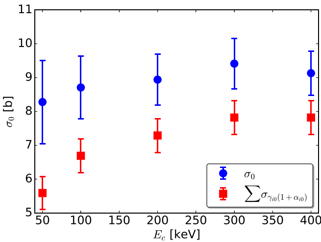
FIG. 10. Variation in the total radiative thermal neutron-capture cross section \sigma_0 and the sum of the experimental cross sections \sum_i \sigma_{\gamma_{i0}}^{\text{expt}}(1 + \alpha_{i0}) feeding the ground state as a function of cutoff energy E_c . This plot was obtained with the BSFG-GLO models using the LD parametrization of Ref. [47] and is representative for PSF-LD combinations adopted in this work.
