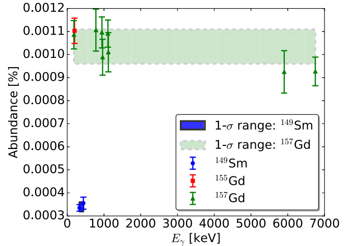
FIG. 3. Measured isotopic abundances of ^{149}\text{Sm} and ^{155,157}\text{Gd} contaminants in the \text{La}_2\text{O}_3 sample. The dark blue (dark gray) and hatched light green (light gray) shaded boundaries correspond to the 1- \sigma uncertainty range on the measured abundances for ^{149}\text{Sm} and ^{157}\text{Gd} , respectively.
