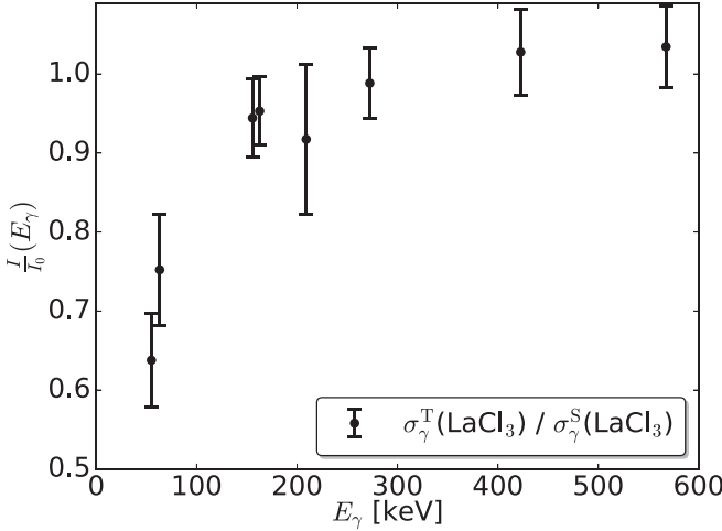
FIG. 4. Ratios of standardized partial \gamma -ray production cross sections for clean prompt ^{139}\text{La}(n, \gamma) transitions measured in the thick \text{LaCl}_3 sample (T) relative to the same transitions in the thin reference \text{LaCl}_3 sample (S). The ratios were measured at the following \gamma -ray energies: 54.9, 63.2, 155.6, 162.6, 209.2, 272.4, 422.7, and 567.4 keV.
