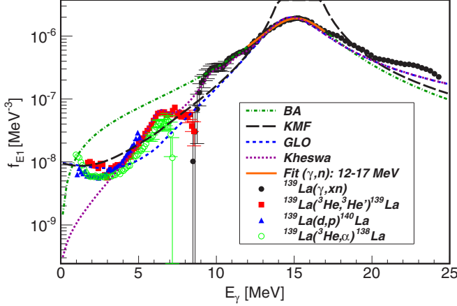
FIG. 6. Experimental data overlaid with BA [51,52] (green dot-dashed line), GLO [56] (blue medium-dashed line), and KMF [55] (black long-dashed line) models describing the E1 PSF. The photonuclear ^{139}\text{La}(\gamma, xn) data (filled black circles) are taken from Ref. [53], the ^{139}\text{La}(\gamma, ^3\text{He}, ^3\text{He}')^{139}\text{La} data (filled red squares) and the ^{139}\text{La}(\gamma, \alpha)^{138}\text{La} data (open green circles) are both taken from Ref. [9], and the ^{139}\text{La}(d, p)^{140}\text{La} data (filled blue triangles) are taken from Ref. [10]. The small-dashed purple curve labeled as Kheswa corresponds to the PSF described in Ref. [9]. The solid orange curve represents a Lorentzian fit to the giant dipole resonance observed over 12–17 MeV used to deduce the adopted parametrizations of the PSF.
