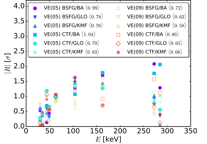
FIG. 11. Absolute residuals |R| , in units of standard deviations \sigma , between simulated population and experimental depopulation to all levels below E_c for the PSF-LD model combinations adopted in this work (Sec. IV F). The LD parametrizations for the combinations denoted “VE(05)” and “VE(09)” are taken from Refs. [46] and [47], respectively. The average residual \langle R \rangle is listed alongside each model combination.
