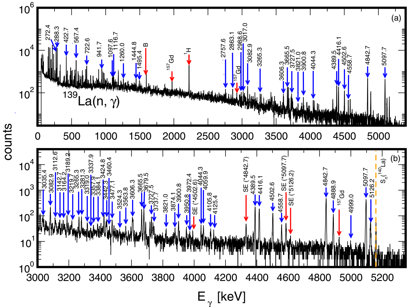
FIG. 1. Prompt \gamma -ray energy spectra observed following the ^{139}\text{La}(n, \gamma) reaction with the \text{La}_2\text{O}_3 sample. The upper panel (a) reveals the complete energy range of interest in the capture- \gamma product ^{140}\text{La} . A strong background line at around 2223 keV from ^1\text{H}(n, \gamma) [22] is clearly visible, as are a few contaminant lines from ^{157}\text{Gd}(n, \gamma) . In the lower panel (b), the same spectrum is expanded around E_\gamma = 3000 – 5350 keV to highlight many of the intense primary \gamma rays observed in this measurement. Prominent background lines (B) and single-escape peaks (SE) are labeled as is the position of the neutron-separation energy ( S_n ) for ^{140}\text{La} .
