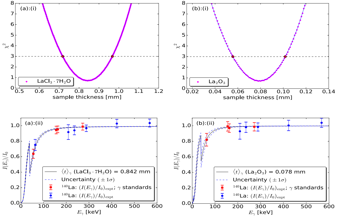
FIG. 5. Upper panels: plot of the global \chi^2 values as a function of the target thickness for (a):(i) \text{LaCl}_3 \cdot 7\text{H}_2\text{O} and (b):(i) \text{La}_2\text{O}_3 . The dashed line drawn at \chi_{\min}^2 + 2.3 defines the 1\sigma range of acceptable t values for two adjustable parameters [36]. Lower panels: Plot of the calculated attenuation factor at the deduced effective sample thicknesses of (a):(ii) \langle t \rangle = 0.842^{(+125)}_{(-124)} mm for \text{LaCl}_3 \cdot 7\text{H}_2\text{O} and (b):(ii) \langle t \rangle = 0.078^{(+24)}_{(-22)} mm for \text{La}_2\text{O}_3 . The experimentally measured attenuation factors [Eq. (3)] for a subset of strong well-resolved \gamma rays are indicated on each plot. The red square data points indicate the \gamma -ray standards used to constrain the fits: 54.9-keV ( \text{LaCl}_3 \cdot 7\text{H}_2\text{O} only); 63.2-keV ( \text{La}_2\text{O}_3 only); 155.6-keV; 162.6-keV; and 272.4-keV transitions. Also shown for comparison are the 63.2- ( \text{LaCl}_3 \cdot 7\text{H}_2\text{O} only), 209.2-, 235.8-, 288.3-, 422.7-, and 567.4-keV transitions (blue circle data points) that were not used to constrain the fitting procedure.
