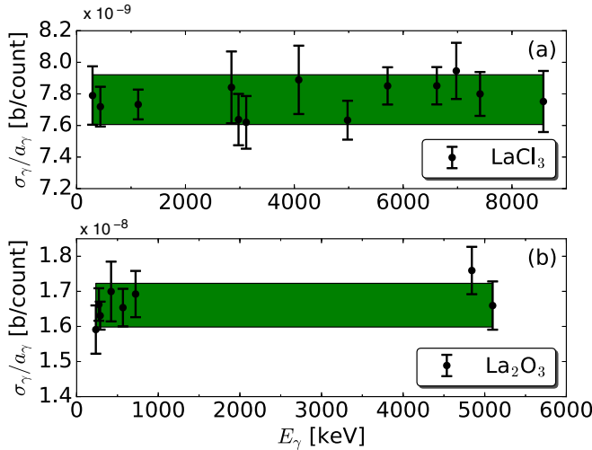
FIG. 2. Normalization \gamma rays used to standardize the (a) \text{LaCl}_3 and (b) \text{La}_2\text{O}_3 spectra. The expectation value of the ratio \sigma_\gamma/a_\gamma is indicated by the shaded 1- \sigma range on each plot. The standardized cross sections used in these plots are listed in Table I and were deduced from the \text{LaCl}_3 sample.
