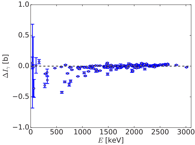
FIG. 9. Plot of the total \gamma -ray intensity balance [ \Delta I_\gamma = \sum I_\gamma(\text{in}) - \sum I_\gamma(\text{out}) ] for all levels observed in ^{140}\text{La} . A dashed black line at \Delta I_\gamma = 0 is drawn for guidance.
