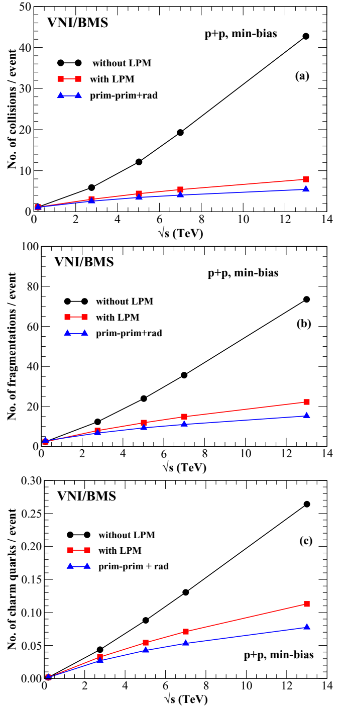
FIG. 1. Number of collisions (a), number of fragmentations (b), and number of charm quarks produced per event (c) for minimum-bias pp interactions as a function of center-of-mass energy. The three calculations involve multiple collisions among partons by neglecting and including the LPM effect and collisions only among primary partons with radiations off the scattered partons.
