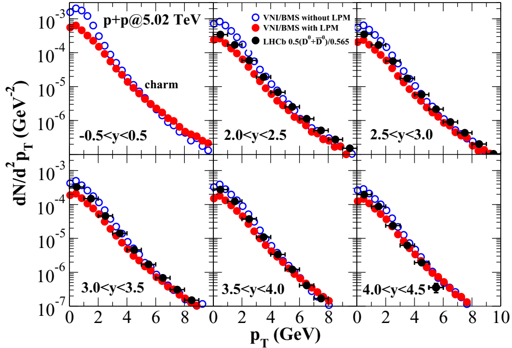
FIG. 5. The transverse momentum spectra of charm quarks in pp collisions at 5.02 TeV due to multiple collisions among partons and fragmentations off final state quarks, with and without inclusion of the LPM effect.
