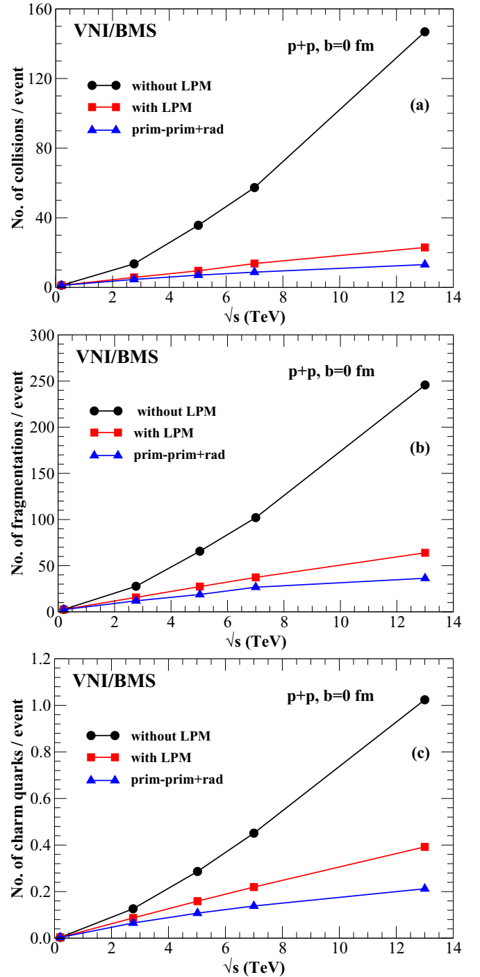
FIG. 2. Number of collisions (a), number of fragmentations (b), and number of charm quarks produced per event (c) for pp interactions as a function of center-of-mass energy at impact parameter equal to zero fm. The three calculations involve multiple collisions among partons by neglecting and including the LPM effect and collisions only among primary partons with radiations off the scattered partons.
