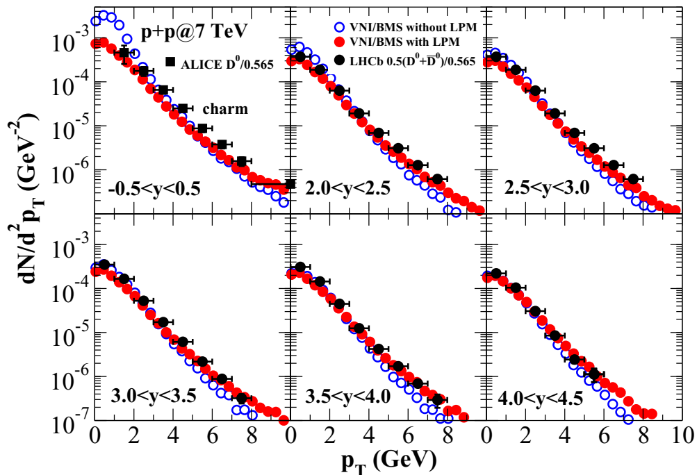
FIG. 6. The transverse momentum spectra of charm quarks in pp collisions at 7.00 TeV due to multiple collisions among partons and fragmentations off final state quarks, with and without inclusion of LPM effect.
