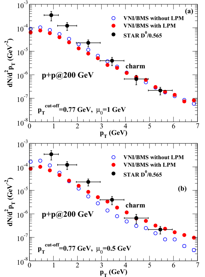
FIG. 4. The transverse momentum spectra of charm quarks in pp collisions at 200 GeV, with p_T^{\text{cut-off}} = 0.77 GeV and \mu_0 = 1 GeV (a) and with p_T^{\text{cut-off}} = 0.77 GeV and \mu_0 = 0.5 GeV (b) due to multiple collisions among partons and fragmentations off final state quarks, with and without inclusion of LPM effect.
