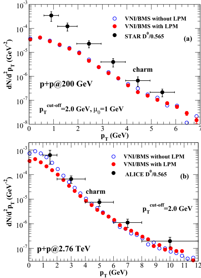
FIG. 3. The transverse momentum spectra of charm quarks in pp collisions at 200 GeV (a) and 2.76 TeV (b) due to multiple collisions among partons and fragmentations off final state quarks, with and without inclusion of LPM effect.
