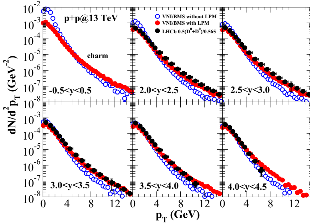
FIG. 7. The transverse momentum spectra of charm quarks in pp collisions at 13.00 TeV due to multiple collisions among partons and fragmentations off final state quarks, with and without inclusion of LPM effect.
