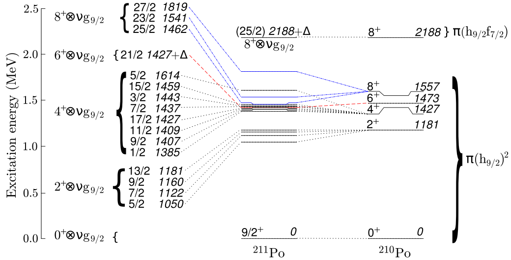
FIG. 8. The \pi(h_{9/2})_{0^+ - 8^+}^2 states and the \pi(h_{9/2}f_{7/2})_{8^+} state in ^{210}\text{Po} are compared to the currently assigned states forming the equivalent \pi(h_{9/2})_{2^+ - 8^+}^2 \otimes \nu g_{9/2} multiplets and the \pi(h_{9/2}f_{7/2})_{8^+} \otimes \nu g_{9/2} state in ^{211}\text{Po} . Note that the states next to the brackets are considered to have positive parity. The ^{210}\text{Po} data is taken from Ref. [21].
