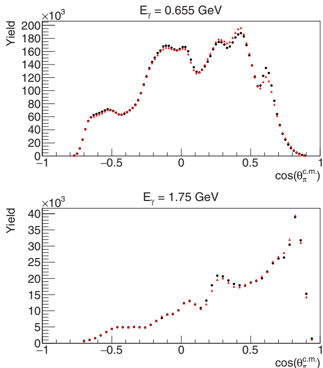
FIG. 8. A comparison of the reconstructed \gamma d \rightarrow \pi^- p(p) yields between the experimental data (black) and the simulation (red) as a function of the pion c.m. angle \cos \theta_{\pi}^{c.m.} in two selected beam energy bins for the 2.655-GeV data. The simulated yields have been scaled such that their integral matches that of the experimental data.
