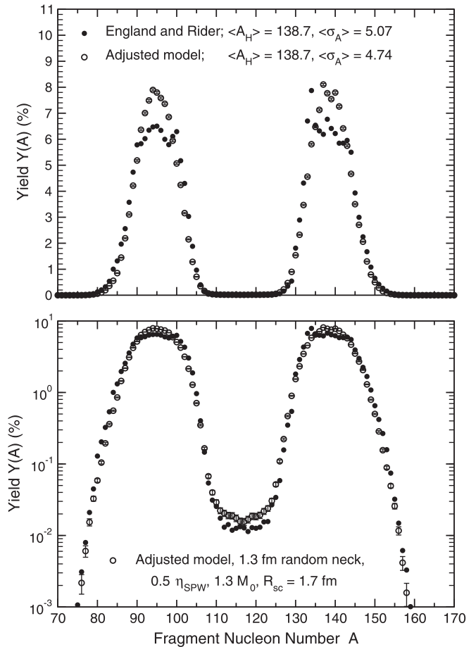
FIG. 12. Calculated postevaporation fragment yields as a function of fragment mass number A from an adjusted model with reduced dissipation, increased inertia, increased scission neck radius, and a random neck rupture, for the thermal-neutron-induced fission of ^{235}\text{U} , compared to the evaluation of England and Rider [115]. The upper part of the figure has a linear yield scale, while the lower part has a logarithmic yield scale.
