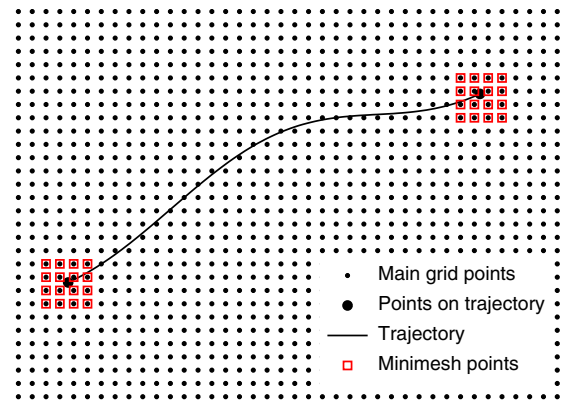
FIG. 2. A schematic representation of a dynamical trajectory in the space of mesh points, with minimeshes surrounding the initial and final points on the trajectory. Along the trajectory, every time a point is reached in the outer layer of hypercells in the minimesh, a new minimesh is defined, centered about the current trajectory point.
