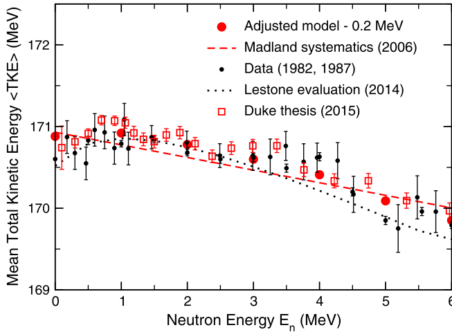
FIG. 19. Calculated average pre-evaporation total fragment kinetic energy as a function of incident neutron energy for ^{235}\text{U}(n, f) , using the same model as for Figs. 12–17 (solid red circles). The model calculations have 0.2 MeV subtracted to facilitate comparison of the predicted neutron energy dependence with the several data sets. The solid black points are the data used by Madland to derive the linear evaluation shown as a red dashed line [114,117,118]. The dotted curve shows the 2014 evaluation of Lestone [119], while the recent measurements of Duke [120] are shown by open red squares. The calculated point at 6 MeV is for first-chance fission only, while the data include about 6% second-chance fission.
