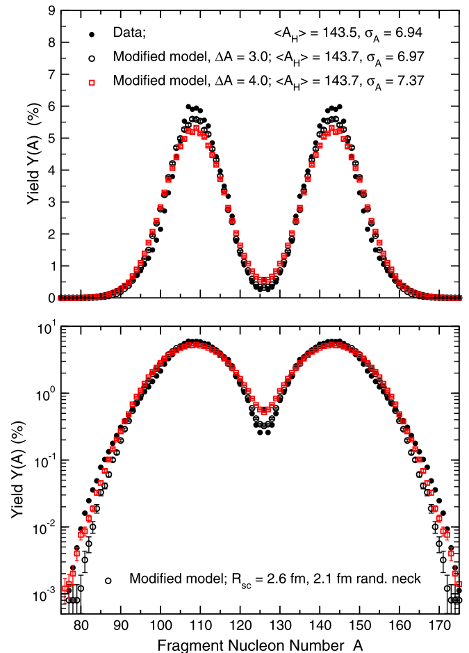
FIG. 41. Calculated pre-evaporation fragment yields as a function of fragment mass number A from the modified model, for spontaneous fission of ^{252}\text{Cf} , compared to experimental data [113]. The dissipation and inertial parameters are the same as in the adjusted model, but a scission neck radius of 2.6 fm and a neck rupture parameter of 2.1 fm are used. The results with two different mass resolutions are shown; \Delta A = 3.0\text{ u} (black circles) and 4.0\text{ u} (red squares). The upper part of the figure shows the yields with a linear scale, while the lower part shows them with a logarithmic scale.
