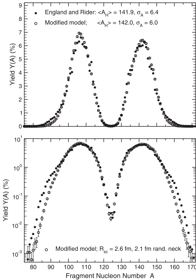
FIG. 40. Calculated postevaporation fragment yields as a function of fragment mass number A from the modified model, for spontaneous fission of ^{252}\text{Cf} , compared to an evaluation [115]. The dissipation and inertial parameters are the same as used in the adjusted model, but a scission neck radius of 2.6 fm and a neck rupture parameter of 2.1 fm are used. The upper part of the figure shows the yields with a linear scale, while the lower part shows them with a logarithmic scale.
