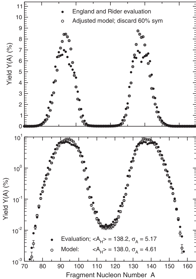
FIG. 23. Calculated postevaporation fragment yields as a function of fragment mass number A from the adjusted model for thermal-neutron-induced fission of ^{233}\text{U} , with 60% of symmetric trajectories removed, compared to evaluated prompt yields [115]. The upper part of the figure shows the yields with a linear scale, while the lower part shows them with a logarithmic scale.
