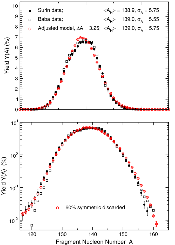
FIG. 24. Calculated pre-evaporation fragment yields as a function of fragment mass number A from the adjusted model with 60% of the symmetric trajectories removed, and a mass resolution \Delta A = 3.25 for thermal-neutron-induced fission of ^{233}\text{U} , compared to two data sets [122,123]. The upper part of the figure shows the yields with a linear scale, while the lower part shows them with a logarithmic scale.
