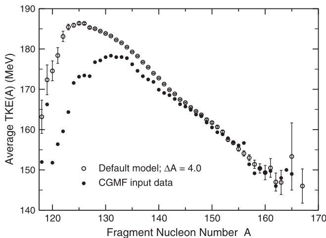
FIG. 8. Calculated pre-evaporation average total fragment kinetic energies as a function of fragment mass number from the default model with a mass resolution \Delta A = 4.0 u for thermal-neutron-induced fission of ^{235}\text{U} , compared to evaluated experimental data [113].
