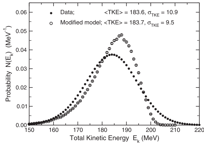
FIG. 42. Calculated pre-evaporation total fragment kinetic energy distribution from the modified model for spontaneous fission of ^{252}\text{Cf} , compared to experimental data [113].
