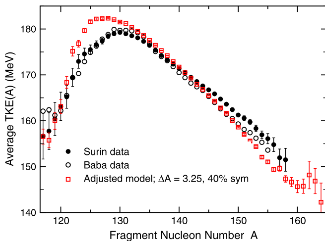
FIG. 26. Calculated pre-evaporation average total fragment kinetic energies as a function of fragment mass number from the adjusted model with 60% of the symmetric trajectories discarded, and a mass resolution \Delta A = 3.25 u for thermal-neutron-induced fission of ^{233}\text{U} , compared to two data sets [122, 123].
