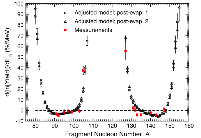
FIG. 20. Logarithmic derivative with respect to neutron energy of the postevaporation fragment yields for ^{235}\text{U}(n, f) . The plotted quantity is \frac{100}{3}[Y(E_3)/Y(E_{\text{th}}) - 1] , where Y(E_3) is the calculated postevaporation fragment yield for 3 MeV neutron-induced fission, while Y(E_{\text{th}}) is the calculated yield for thermal-neutron-induced fission of ^{235}\text{U} . The points labeled post-evap 1 (open circles) and post-evap 2 (open triangles) utilize different assumptions about the distribution of excitation energy in the heavy and light fragments for 3 MeV neutron energy. See the text for details. The data points (solid squares) are from linear fits to measured prompt yields as a function of the energy of monoenergetic neutron beams interacting with ^{235}\text{U} targets from Ref. [121].
