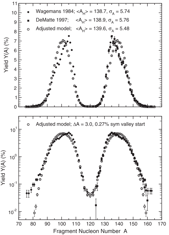
FIG. 36. Calculated pre-evaporation fragment yields as a function of fragment mass number A from the adjusted model with 0.27% of the trajectories starting in the symmetric valley, while the remainder start in the asymmetric valley, for spontaneous fission of ^{240}\text{Pu} , compared to experimental data [125,127]. The mass resolution applied to the model is \Delta A = 3.0 u. The upper part of the figure shows the yields with a linear scale, while the lower part shows them with a logarithmic scale.
