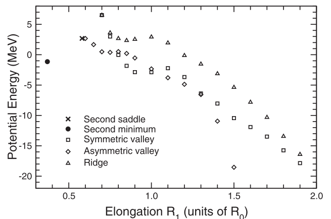
FIG. 28. The calculated energies of the second minimum, the second (outermost) saddle point, the mass-symmetric and mass-asymmetric valleys, and the ridge between them as functions of the coordinate R_1 for ^{240}\text{Pu} .
