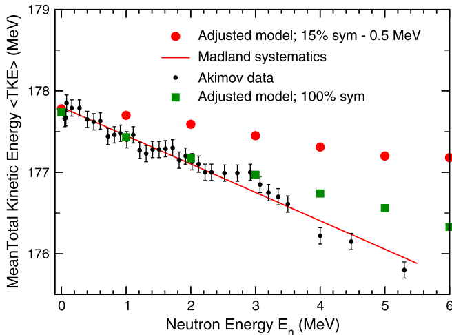
FIG. 34. Calculated average pre-evaporation total fragment kinetic energy as a function of incident neutron energy for ^{239}\text{Pu}(n, f) , using the same model as for Figs. 30–33 (solid red circles). The model calculations have 0.5 MeV subtracted to facilitate comparison of the predicted neutron energy dependence with the data set. The solid black points are the data used by Madland to derive the linear evaluation shown as a red solid line [117,126]. The same model with all symmetric trajectories included, used to calculate the results shown in Fig. 29, predicts the energy dependence shown by the green solid squares. The calculated points at 6 MeV are for first-chance fission only.
