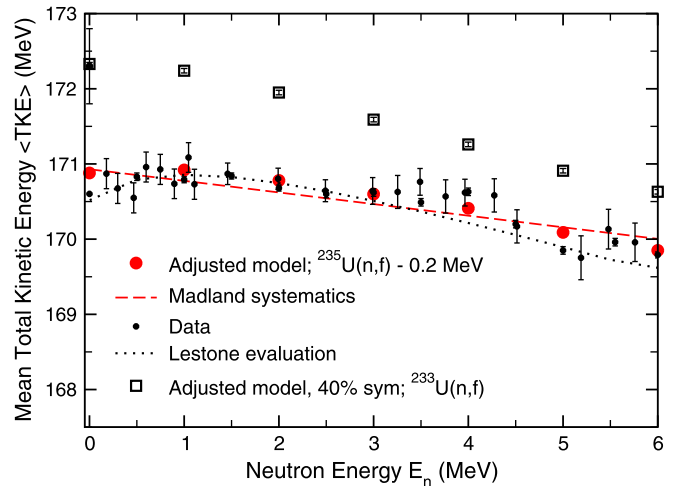
FIG. 27. Similar to Fig. 19. The solid data points, the Madland systematics [117], the Lestone evaluation [119], and the solid circles (model) are the same as in that figure, and apply to ^{235}\text{U}(n, f) , while the open squares are calculated using the same adjusted model, with 60% of the symmetric trajectories discarded, for ^{233}\text{U}(n, f) . The data point for ^{233}\text{U}(n, f) at thermal energy is from Ref. [124]. The calculated points at 6 MeV are for first-chance fission only, while the data include about 6% second-chance fission.
