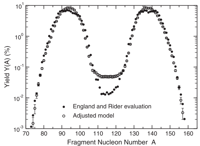
FIG. 22. Calculated postevaporation fragment yields as a function of fragment mass number A from the adjusted model for thermal-neutron-induced fission of ^{233}\text{U} , compared to evaluated prompt yields [115].
