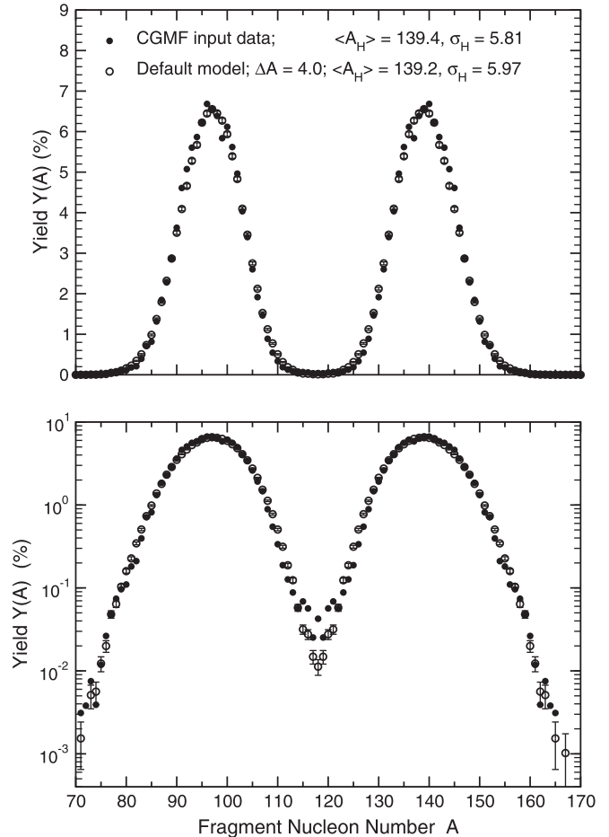
FIG. 6. Calculated pre-evaporation fragment yields as a function of fragment mass number A from the default model with a mass resolution \Delta A = 4.0 u for thermal-neutron-induced fission of ^{235}\text{U} , compared to evaluated experimental data [113]. The upper part has a linear yield scale, while the lower part shows the same points with a logarithmic yield scale.
