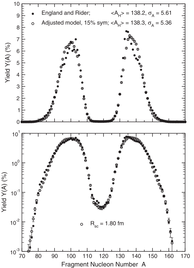
FIG. 30. Calculated postevaporation fragment yields as a function of fragment mass number A from the adjusted model for thermal-neutron-induced fission of ^{239}\text{Pu} , compared to the evaluation of England and Rider [115]. The model uses the same parameters as for ^{235}\text{U}(n, f) except for a scission neck radius of 1.8 fm instead of 1.7 fm. 85% of symmetric trajectories have been discarded to more closely approximate the symmetric yield. The upper part of the figure shows the yields with a linear scale, while the lower part shows them with a logarithmic scale.
