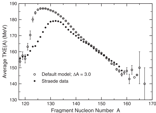
FIG. 10. Calculated pre-evaporation average total fragment kinetic energies as a function of fragment mass number A from the default model with a mass resolution \Delta A = 3.0 for thermal-neutron-induced fission of ^{235}\text{U} , compared to the data of Straede [114].
