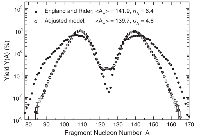
FIG. 39. Calculated postevaporation fragment yields as a function of fragment mass number A from the adjusted model, for spontaneous fission of ^{252}\text{Cf} , compared to an evaluation [115]. All trajectories start in the neighborhood of the exit point in the asymmetric valley, and the scission neck radius is 2.0 fm, compared to 1.8 fm used for Figs. 36–38.
