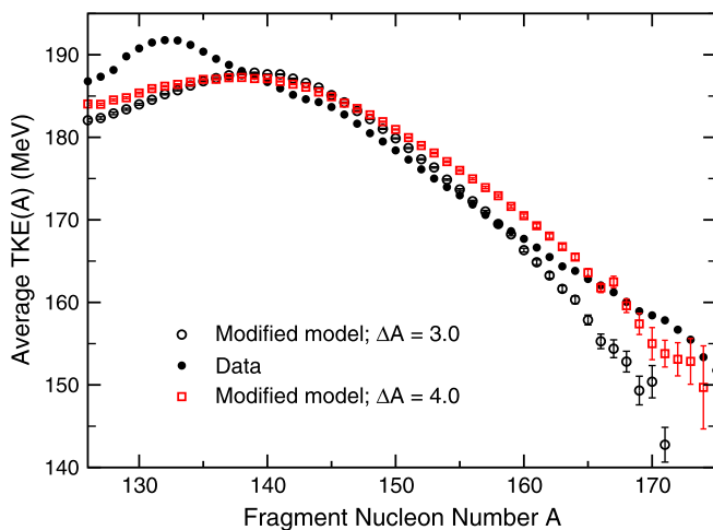
FIG. 43. Calculated pre-evaporation average total fragment kinetic energies as a function of fragment mass number from the modified model with a mass resolution \Delta A = 3.0 u (black circles) and 4.0 u (red squares), for spontaneous fission of ^{252}\text{Cf} , compared to experimental data [113].
