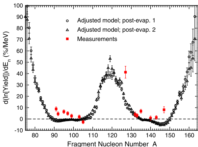
FIG. 35. Same as Fig. 20, for ^{239}\text{Pu}(n, f) .
