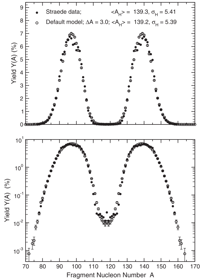
FIG. 9. Calculated pre-evaporation fragment yields as a function of fragment mass number A from the default model with a mass resolution \Delta A = 3.0 for thermal-neutron-induced fission of ^{235}\text{U} , compared to the data of Straede [114]. The upper part has a linear yield scale, while the lower part shows the same points with a logarithmic yield scale.
