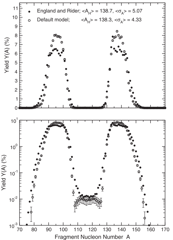
FIG. 11. Calculated postevaporation fragment yields as a function of fragment mass number A from the default model for thermal-neutron-induced fission of ^{235}\text{U} , compared to the evaluation of England and Rider [115]. The upper part of the figure has a linear yield scale, while the lower part has a logarithmic yield scale.
