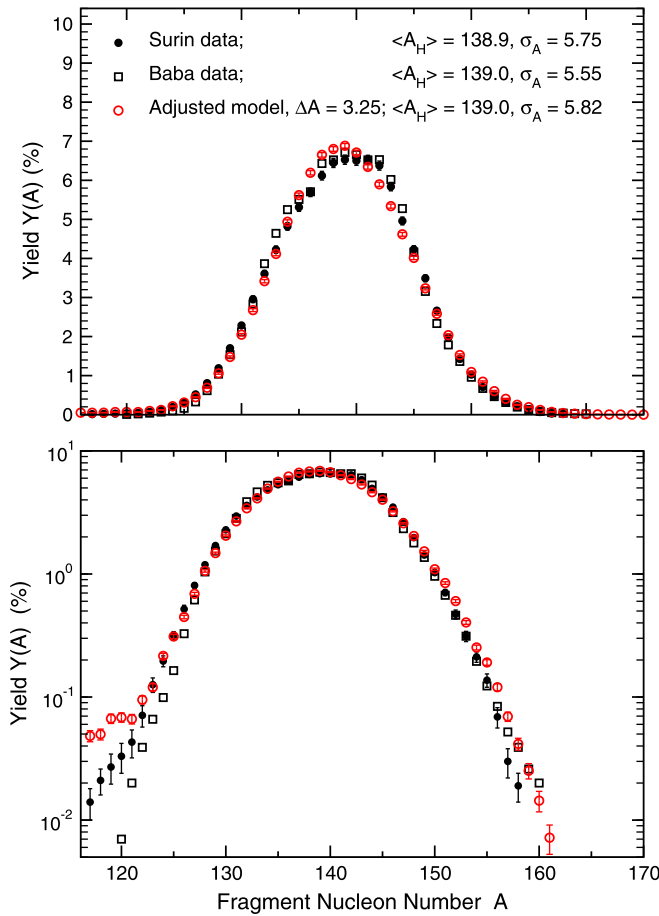
FIG. 21. Calculated pre-evaporation fragment yields as a function of fragment mass number A from the adjusted model with a mass resolution \Delta A = 3.25 for thermal-neutron-induced fission of ^{233}\text{U} (red circles), compared to two data sets [122,123]. The upper part of the figure shows the yields with a linear scale, while the lower part shows them with a logarithmic scale.
