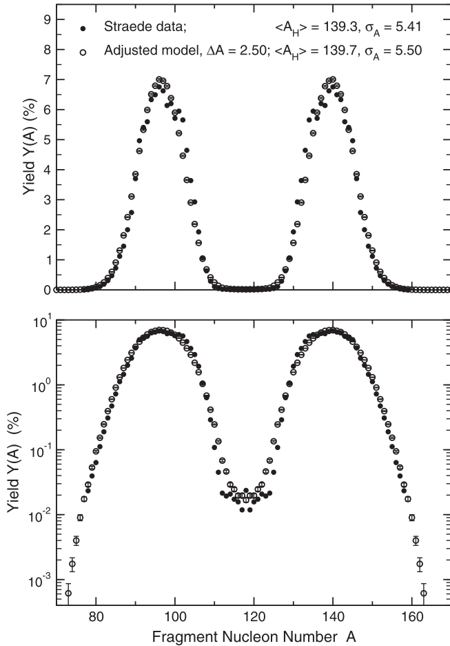
FIG. 16. Calculated pre-evaporation fragment yields as a function of fragment mass number A from the adjusted model with a mass resolution \Delta A = 2.50 u for thermal-neutron-induced fission of ^{235}\text{U} , compared to the data of Straede [114]. The calculated trajectories are identical to those used to calculate the results in Fig. 13 except for the use of a different mass-resolution filter. The upper part of the figure shows the yields with a linear scale, while the lower part shows them with a logarithmic scale.
