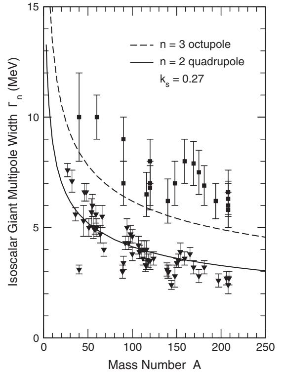
FIG. 4. Isoscalar giant quadrupole and octupole widths used in 1985 to fix the strength k_s of the surface dissipation. The width data are from Refs. [82,83].
