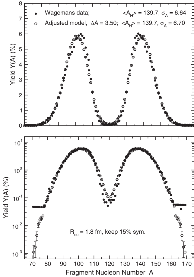
FIG. 31. Calculated pre-evaporation fragment yields as a function of fragment mass number A from the adjusted model with 85% of the symmetric yield discarded, for thermal-neutron-induced fission of ^{239}\text{Pu} , compared to experimental data [125]. The scission neck radius of 1.8 fm is used instead of 1.7 fm for the case of ^{235}\text{U}(n, f) shown previously, while the mass resolution \Delta A = 3.50 u. The upper part of the figure shows the yields with a linear scale, while the lower part shows them with a logarithmic scale.
