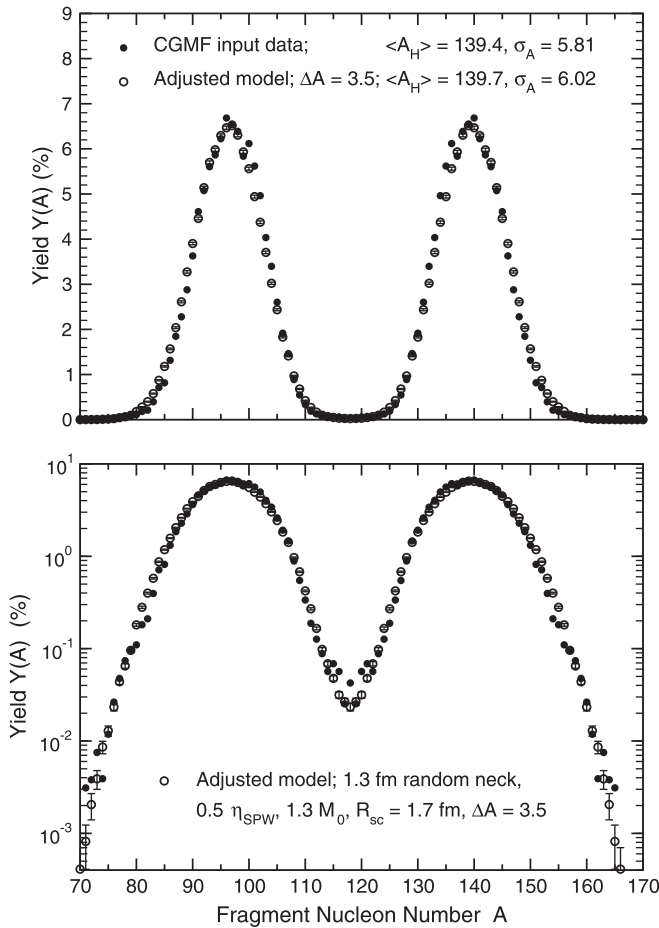
FIG. 13. Calculated pre-evaporation fragment yields as a function of fragment mass number A from an adjusted model with reduced dissipation, increased inertia, increased scission neck radius, and a random neck rupture, for the thermal-neutron-induced fission of ^{235}\text{U} , compared to evaluated experimental data [113].
