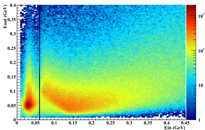
FIG. 3. The energy deposited in the inner ( E_{in} ) and outer ( E_{out} ) layers of the EC for all electron candidates. The line corresponds to 60 MeV, which separates the minimum ionizing pions (to the left) and electrons (to the right).
