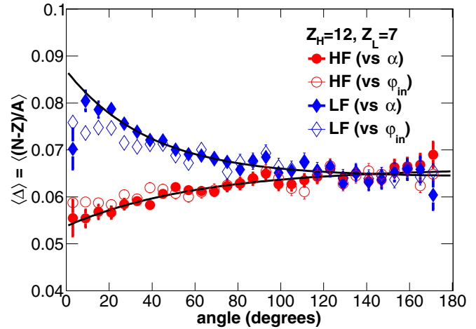
FIG. 8. Average composition \langle \Delta \rangle as a function of the decay alignment \alpha (in full markers) and the in-plane angle \varphi_{\text{in}} (in open markers) for the Z_H = 12 , Z_L = 7 pair in the ^{70}\text{Zn} + ^{70}\text{Zn} system.
