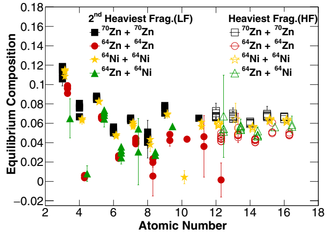
FIG. 12. Equilibrium composition as a function of the atomic number. All four systems studied are represented: ^{70}\text{Zn} + ^{70}\text{Zn} in black squares, ^{64}\text{Zn} + ^{64}\text{Zn} in red circles, ^{64}\text{Ni} + ^{64}\text{Ni} in yellow stars, and ^{64}\text{Zn} + ^{64}\text{Ni} in green triangles. The open markers correspond to the atomic numbers of the HF and the full markers represent the atomic numbers of the LF. The different sets of data are slightly horizontally offset for clarity.
