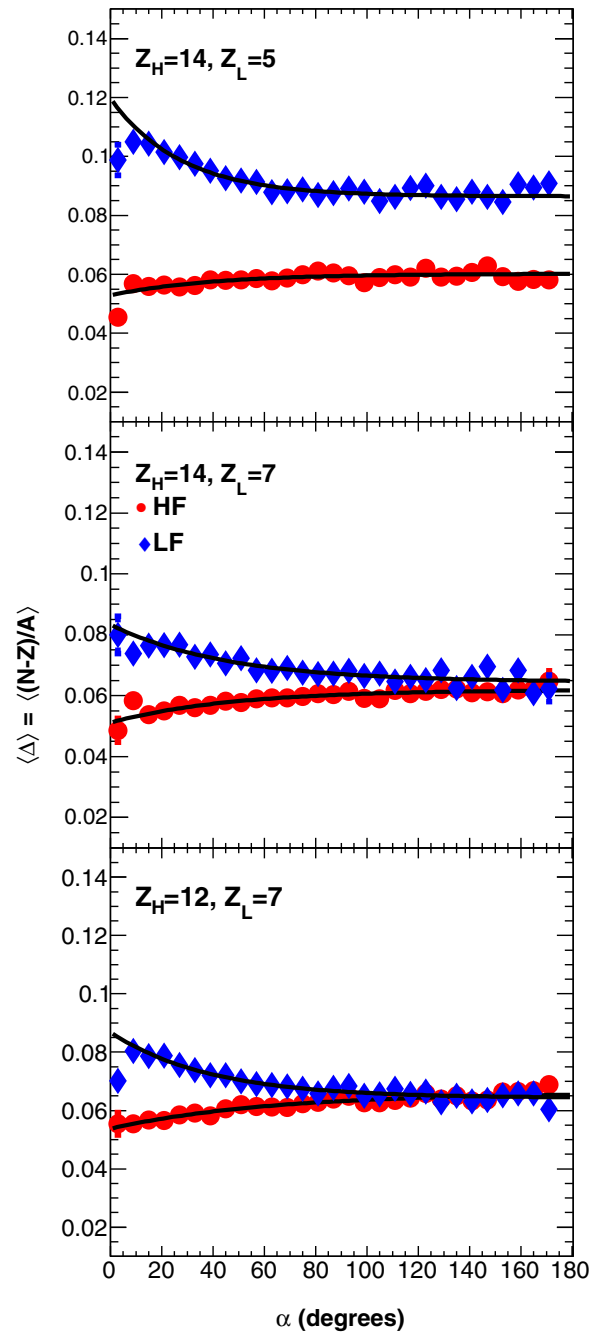
FIG. 6. Average composition \langle\Delta\rangle as a function of the decay alignment \alpha for the ^{70}\text{Zn} + ^{70}\text{Zn} system. Three representative combinations of HF (red circles) and LF (blue rhombi) are shown: Z_H = 14, Z_L = 5 (upper panel), Z_H = 14, Z_L = 7 (middle panel), and Z_H = 12, Z_L = 7 (lower panel). The black lines correspond to the exponential fits of the data.
