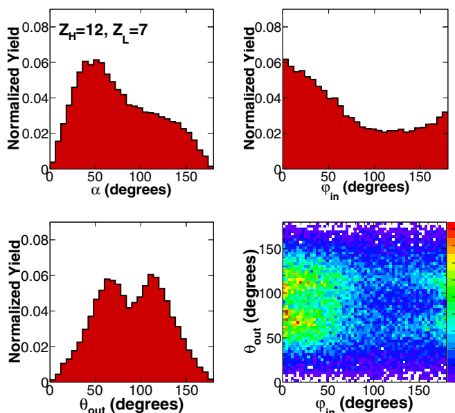
FIG. 3. Normalized yield as a function of the angular in-plane distribution \varphi_{\text{in}} (top right panel), out-of-plane distribution \theta_{\text{out}} (bottom left panel), and \alpha (top left panel). The bottom right panel shows the angular distribution as a function of the in-plane and out-of-plane angles simultaneously, with a linear color scale. All angular distributions shown correspond to the Z_H = 12 , Z_L = 7 combination of HF and LF of the ^{70}\text{Zn} + ^{70}\text{Zn} system.
