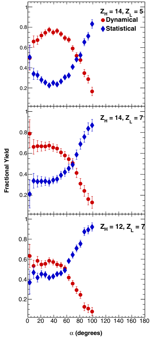
FIG. 5. Fractional yield as a function of \alpha for the ^{70}\text{Zn} + ^{70}\text{Zn} system. Three representative combinations of HF and LF are shown: Z_H = 14 , Z_L = 5 (upper panel), Z_H = 14 , Z_L = 7 (middle panel), and Z_H = 12 , Z_L = 7 (lower panel). The circular red markers correspond to the dynamical contribution while the blue rhombic markers represent the statistical contribution.
