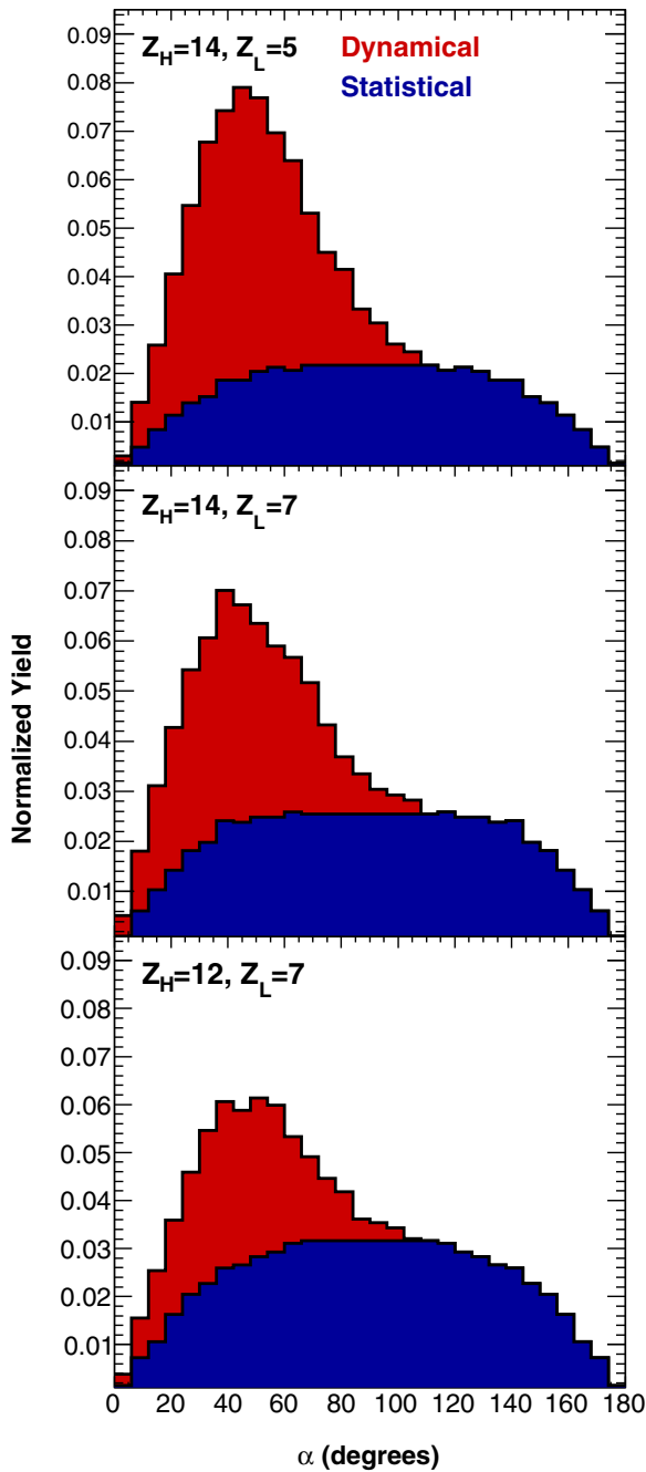
FIG. 4. Normalized angular distribution \alpha for the ^{70}\text{Zn} + ^{70}\text{Zn} system. Three representative combinations of HF and LF are shown: Z_H = 14 , Z_L = 5 (upper panel), Z_H = 14 , Z_L = 7 (middle panel), and Z_H = 12 , Z_L = 7 (lower panel). The blue area represents the statistical contribution and the remaining area (red) represents the dynamical contribution.
