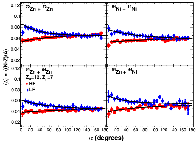
FIG. 11. Average composition \langle \Delta \rangle as a function of the decay alignment \alpha for the Z_H = 12, Z_L = 7 pair in all systems studied (i.e., ^{70}\text{Zn} + ^{70}\text{Zn} , ^{64}\text{Zn} + ^{64}\text{Zn} , ^{64}\text{Ni} + ^{64}\text{Ni} , and ^{64}\text{Zn} + ^{64}\text{Ni} ). The HF is represented in red circles and the LF in blue rhombi. The black lines correspond to the exponential fits of the data.
