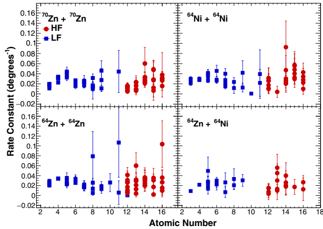
FIG. 13. Rate constants (in units of inverse degrees) as a function of the atomic number. All four systems are represented: ^{70}\text{Zn} + ^{70}\text{Zn} (top left panel), ^{64}\text{Ni} + ^{64}\text{Ni} (top right panel), ^{64}\text{Zn} + ^{64}\text{Zn} (lower left panel), and ^{64}\text{Zn} + ^{64}\text{Ni} (lower right panel). The red circles represent the atomic numbers of the HF while the blue squares represent the atomic numbers of the LF.
