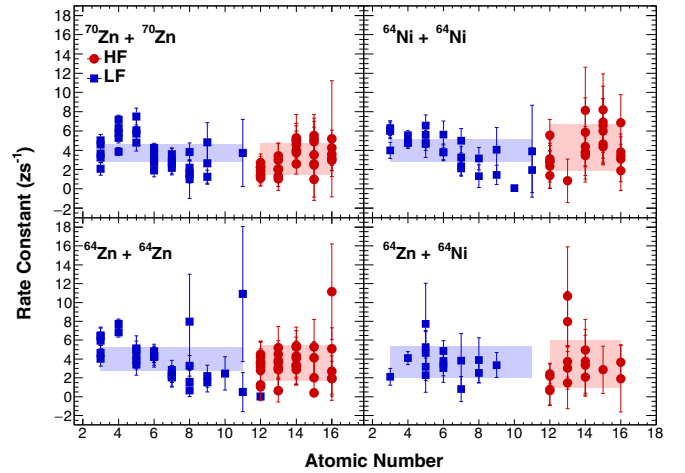
FIG. 14. Rate constants (in units of inverse zs) as a function of the atomic number. All four systems are represented: ^{70}\text{Zn} + ^{70}\text{Zn} (top left panel), ^{64}\text{Ni} + ^{64}\text{Ni} (top right panel), ^{64}\text{Zn} + ^{64}\text{Zn} (lower left panel), and ^{64}\text{Zn} + ^{64}\text{Ni} (lower right panel). The red circles represent the atomic numbers of the HF while the blue squares represent the atomic numbers LF. The shaded areas correspond to the average rate constant per zs values for the HF and LF.
