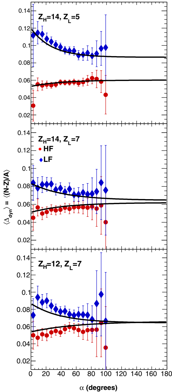
FIG. 7. Average dynamical composition, \langle \Delta_{\text{dyn}} \rangle , as a function of the decay alignment \alpha for the ^{70}\text{Zn} + ^{70}\text{Zn} system. Three representative combinations of HF (red circles) and LF (blue rhombi) are shown: Z_H = 14 , Z_L = 5 (upper panel), Z_H = 14 , Z_L = 7 (middle panel), and Z_H = 12 , Z_L = 7 (lower panel). The black lines correspond to the exponential fit of the average composition as a function of the decay alignment.
