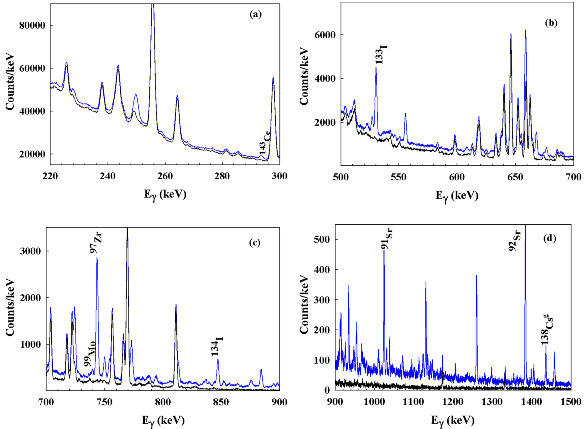
FIG. 2. Gamma-ray energy spectra of interest for ^{239}\text{Pu} prior to (lower) and after irradiation (upper) with 11 MeV photons. The transitions corresponding to the fission products identified in the present work are labeled. Both spectra are normalized to the same live-time.
