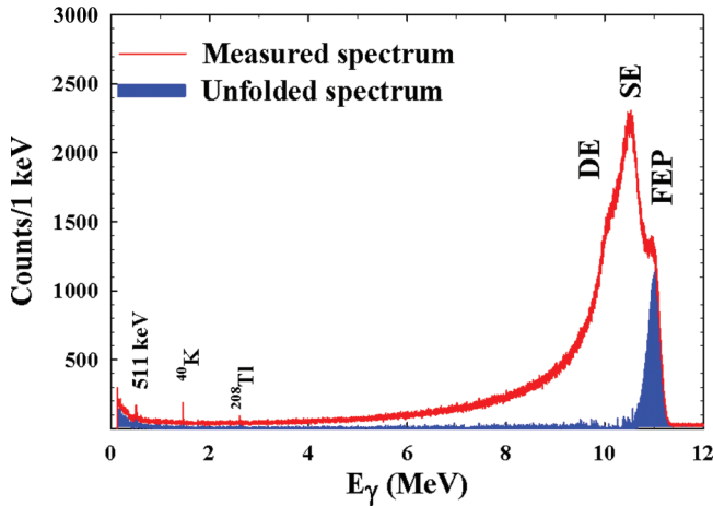
FIG. 1. Photon spectrum (in red) measured with a 123% HPGe detector positioned at 0^\circ relative to the incident photon beam of 11.0 MeV. The full-energy peak (FEP), single escape (SE), and double escape (DE) are labeled. In the low-energy part of the spectrum, room background lines are clearly seen. An unfolded spectrum (in blue) of the FEP is indicated by the shaded area.
