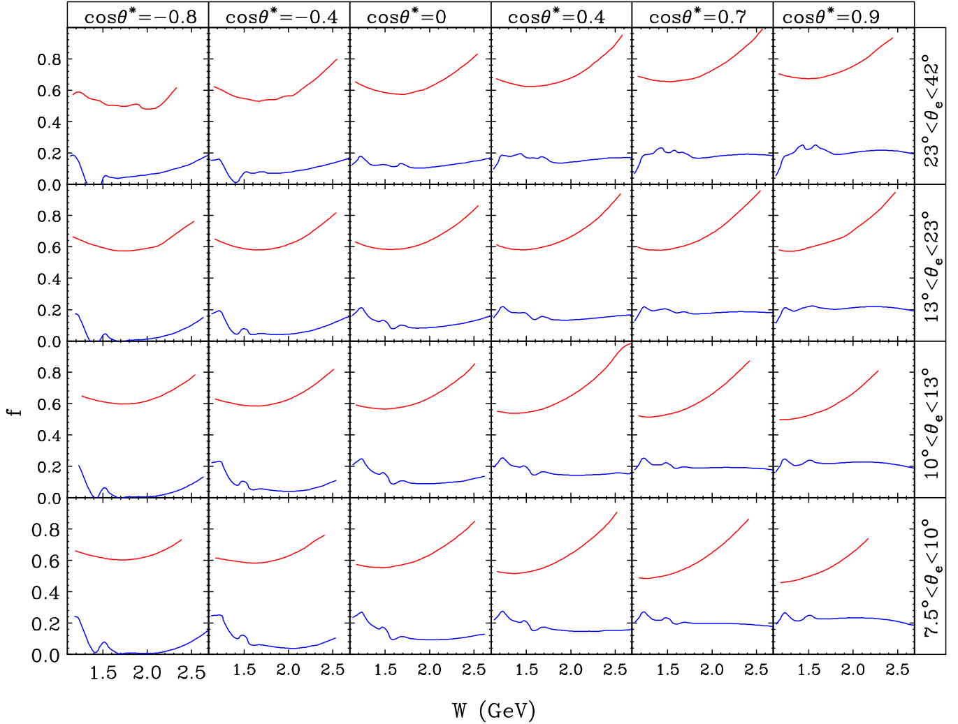
FIG. 8. Same as Fig. 7, except for the two \pi^- topologies: ed \rightarrow e\pi^- p(p) (upper red curves) and ed \rightarrow e\pi^- (pp) (lower blue curves).
