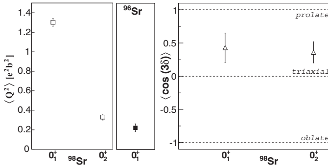
FIG. 8. Quadrupole deformation parameters obtained with the sum-rule method for the 0_{1,2}^+ states in ^{98}\text{Sr} and 0_1^+ in ^{96}\text{Sr} .
