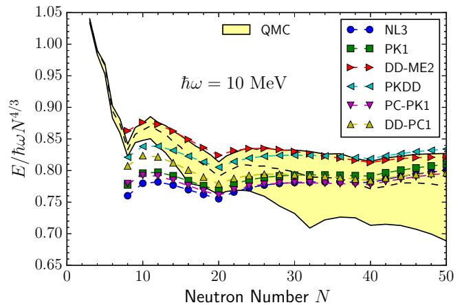
FIG. 1. Total energies (scaled by \hbar\omega N^{4/3} ) of N -neutron systems in a HO trap ( \hbar\omega = 10 \text{ MeV} ) predicted with various relativistic density functionals (solid symbols). The shaded area indicates the ab initio QMC results from Refs. [14,15] for the NN interaction AV8' (center dashed line) as well as the AV8' plus 3N interactions of UIX (upper solid line) and IL7 (lower solid line).
