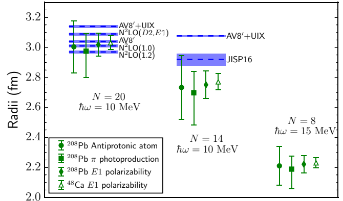
FIG. 3. The rms radii for three neutron drops determined from their linear correlations with the neutron skin thicknesses of ^{208}\text{Pb} and ^{48}\text{Ca} . For comparison, the ab initio results obtained using phenomenological forces and local chiral forces of Ref. [63] are also shown.
