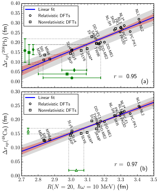
FIG. 2. (a) Neutron skin thickness \Delta r_{np} of ^{208}\text{Pb} against the rms radius R of 20 neutrons trapped in a HO potential with \hbar\omega = 10 MeV for various nuclear density functionals. The inner (outer) colored regions depict the 95% confidence (prediction) intervals of the linear regression, and Pearson's correlation coefficient r is also displayed ( r is a value between +1 and -1 inclusive, where +1 is total positive correlation, 0 is no correlation, and -1 is total negative correlation; see, e.g., Ref. [56]). The data of \Delta r_{np} in different measurements with antiprotonic atoms [31] (circle), pion photoproduction [28] (square), and electric dipole polarizability [57] (diamond) are also given together with their projections on the radius of the neutron drop. (b) Same plot, but for the neutron skin thickness \Delta r_{np} of ^{48}\text{Ca} . The estimate of \Delta r_{np} is from a prediction of electric dipole polarizability [58].
