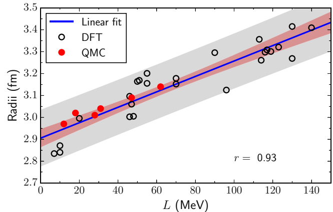
FIG. 4. Values of the slope L of the symmetry energy against rms radii of 20 neutrons in a HO with \hbar\omega = 10 \text{ MeV} , obtained with density functional theories (open circles) and ab initio methods (solid circles).
