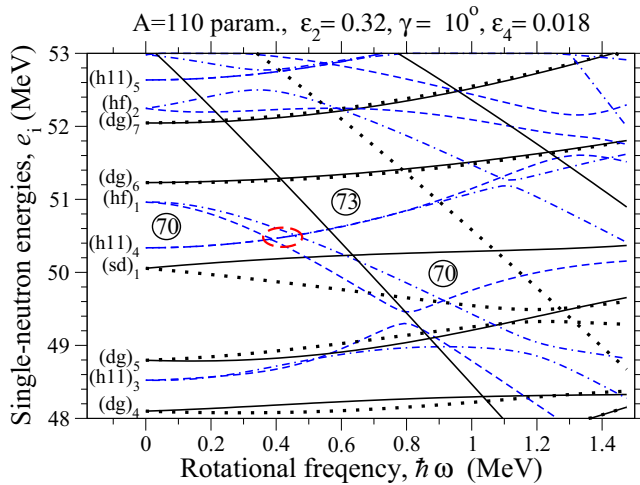
FIG. 12. Calculated neutron orbitals as a function of rotational frequency, \hbar\omega , at a deformation typical for the high-spin configurations of ^{124}\text{Xe} , \epsilon_2 = 0.32 , \gamma = 10^\circ , \epsilon_4 = 0.018 . The orbitals are labeled at \hbar\omega = 0 by their dominant j -shell amplitude and the ordering within the respective groups. The h_{11/2} orbitals are labeled as (h11) while pseudospin partners [31] d_{5/2}g_{7/2} , s_{1/2}d_{3/2} , and h_{9/2}f_{7/2} are labeled as (dg) , (sd) , and (hf) , respectively. Dashed (or dot-dashed) lines are used for negative-parity orbitals while lines with dots are used for signature \alpha = -1/2 . The crossing between the (h11)_4 and (hf)_1 orbitals is highlighted with a dashed ellipse.
