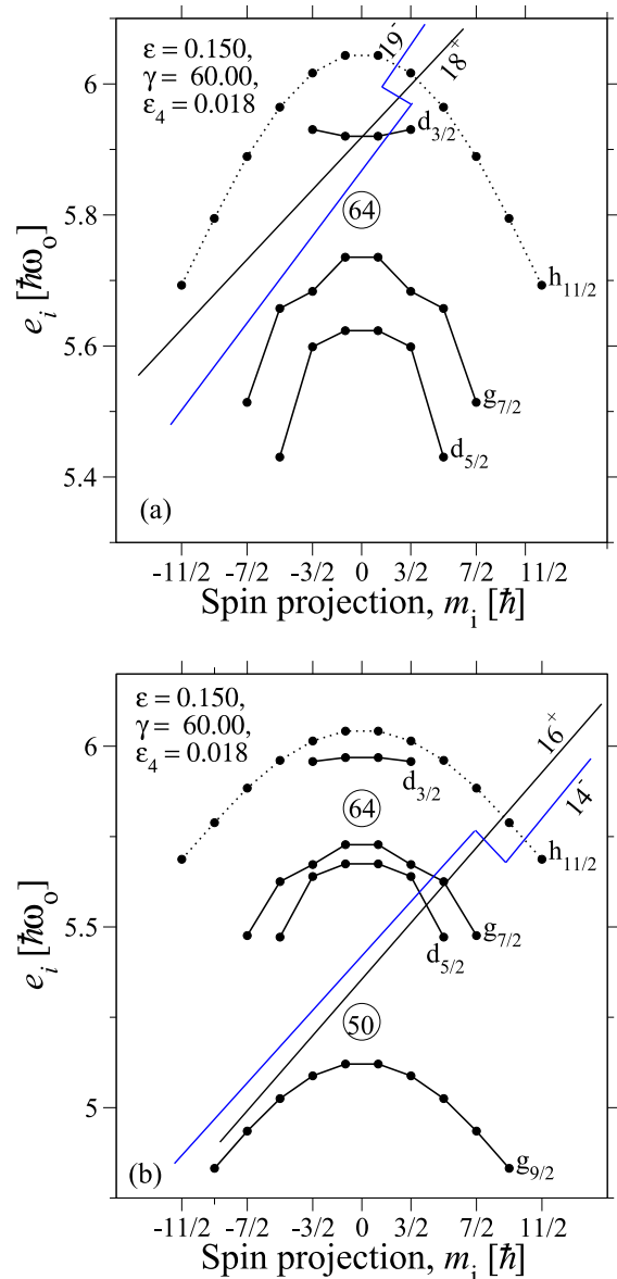
FIG. 8. Calculated single-particle energies, e_i , as a function of the spin-projection quantum number, m_i , at \varepsilon_2 \approx 0.15 , \gamma = 60^\circ : (a) for neutrons and (b) for protons. Some low-lying aligned configurations are defined by “straight-line Fermi surfaces,” where the orbitals below the lines are occupied and the total spin is obtained as the sum of the projections m_i below the lines.
