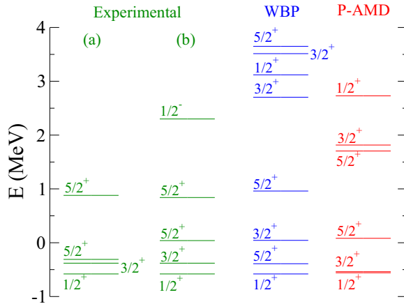
FIG. 1. Experimental (far left column) [29,33] and calculated spectrum of ^{19}\text{C} in a shell-model calculation with OXBASH using the WBP interaction [40,41] (middle right column), and within a semimicroscopic core-plus-valence-particle calculation (P-AMD, far right column) which takes into account core excitations as described in [34]. We include a second experimental spectrum (middle left column) due to the discrepancy raised by the latest knock-out experiments [30–32].
