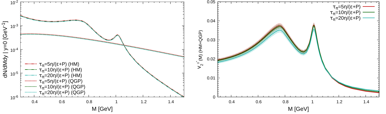
FIG. 8. Dilepton yield (left panel) and elliptic flow (right panel) as a function of invariant mass, for different values of shear relaxation time.
