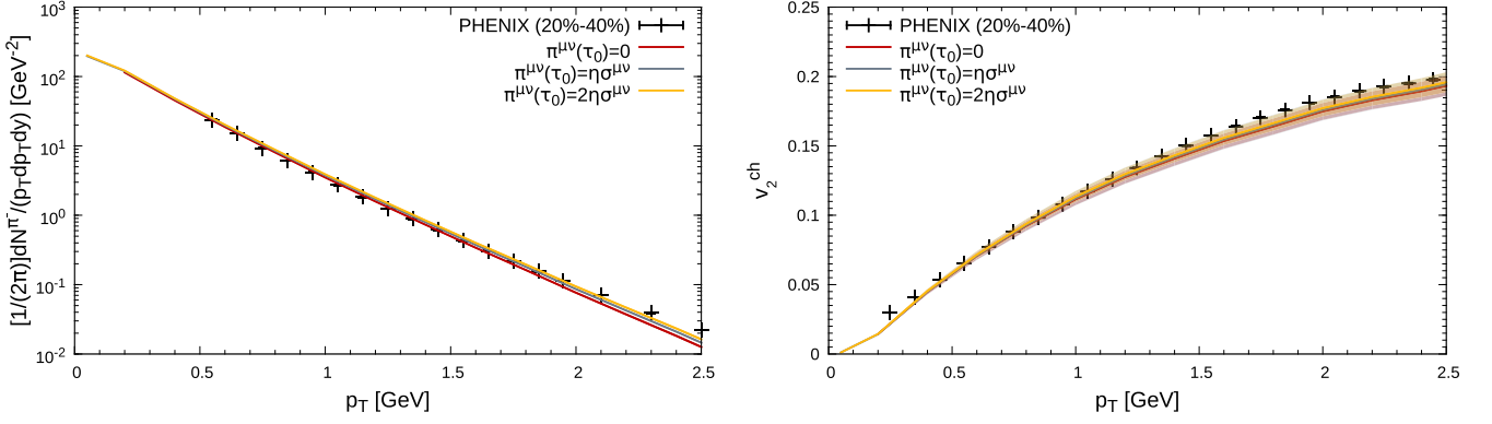
FIG. 10. Pion transverse momentum spectra (left panel) and charged hadron differential elliptic flow (right panel) as a function of transverse momentum, for different values of the initial shear-stress tensor.
