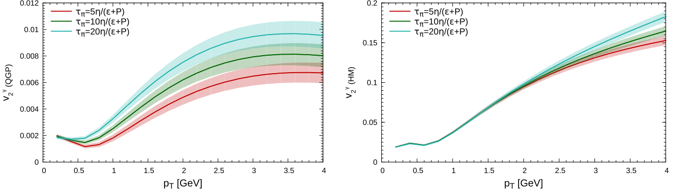
FIG. 4. Differential elliptic flow of thermal photons emitted by the QGP (left panel) and emitted by the hadronic medium (HM) (right panel) as a function of transverse momentum, for different values of shear relaxation time.
