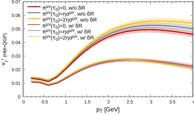
FIG. 12. Thermal photon elliptic flow with and without viscous corrections ( \delta R ) to the emission rates.
