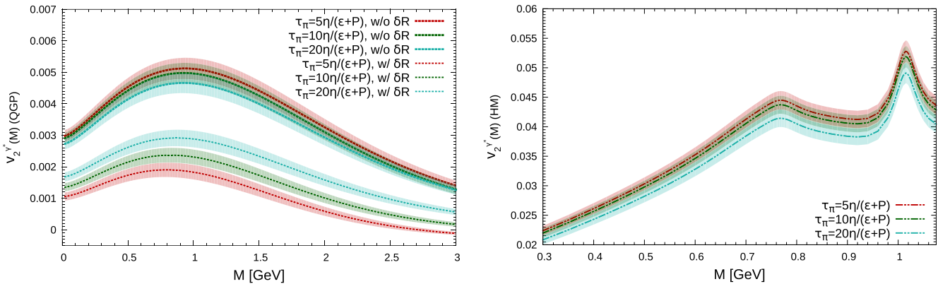
FIG. 7. Differential elliptic flow of dileptons emitted by the QGP (left panel) and emitted by the hadronic medium (right panel) as a function of the dilepton invariant mass, for different values of shear relaxation time. The effect of the viscous correction to the QGP rate is presented in the left panel, whereas that of the HM rate is small and hence only results using the rate including the viscous correction is presented in the right panel.
