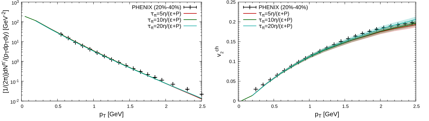
FIG. 2. Pion transverse momentum spectra (left panel) and charged hadron differential elliptic flow (right panel) as a function of transverse momentum, for different values of shear relaxation time. Here, and in all subsequent figures of this paper, the colored bands represent the statistical uncertainty associated with 200 hydrodynamical events.
