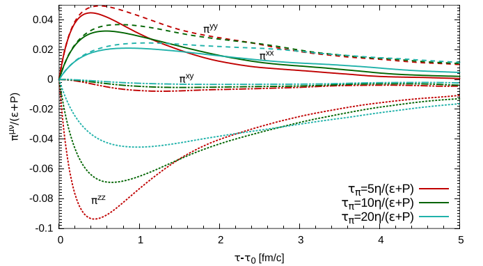
FIG. 1. Event averaged shear-stress tensor for b_\pi = 5, 10, 20 in the local rest frame of the fluid cell located at x = y = 2.67 fm, z = 0 fm. Results with b_\pi = 5 are in red, b_\pi = 10 in dark green and b_\pi = 20 in light green. Different types of lines are used for various components of \pi^{\mu\nu} . The full line is reserved for \pi^{xx} , dashed line for \pi^{yy} , dotted line for \pi^{zz} and dash-dotted line is used for \pi^{xy} .
