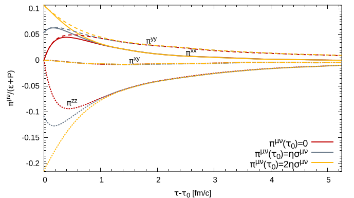
FIG. 9. Shear-stress tensor for c = 0, 1/2, 1 in the local rest frame of the fluid cell located at x = y = 2.67 fm, z = 0 fm, averaged over all events. Results with c = 0 are displayed in red, c = 1/2 in gray, and c = 1 in yellow.
