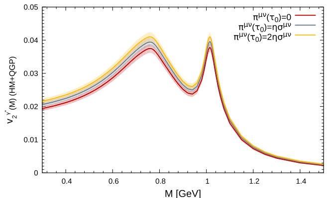
FIG. 13. Dilepton yield (left panel) and elliptic flow (right panel) as a function of invariant mass, for different values of initial \pi^{\mu\nu} .
