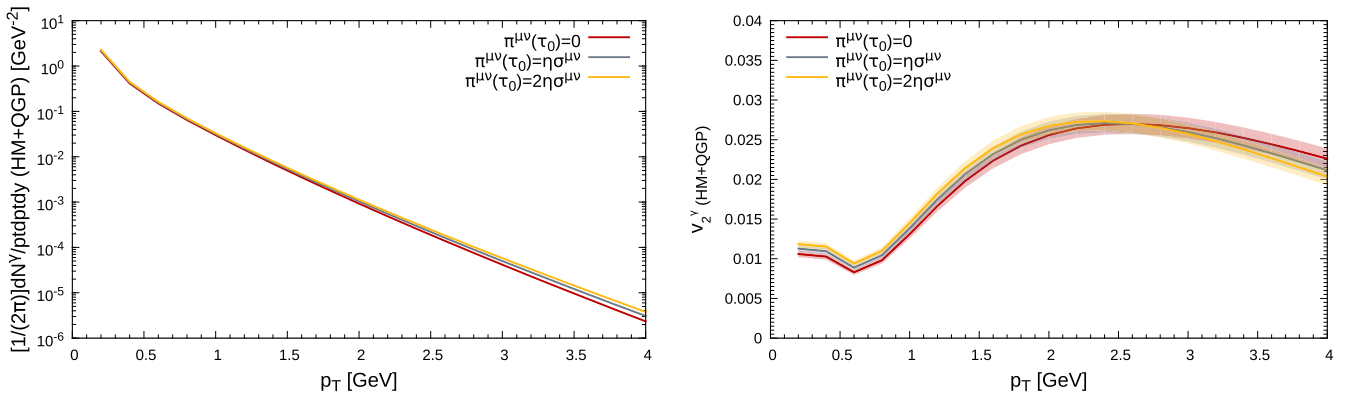
FIG. 11. Transverse momentum spectra (left panel) and differential elliptic flow (right panel) of thermal photons as a function of transverse momentum, for different values of initial \pi^{\mu\nu} .
