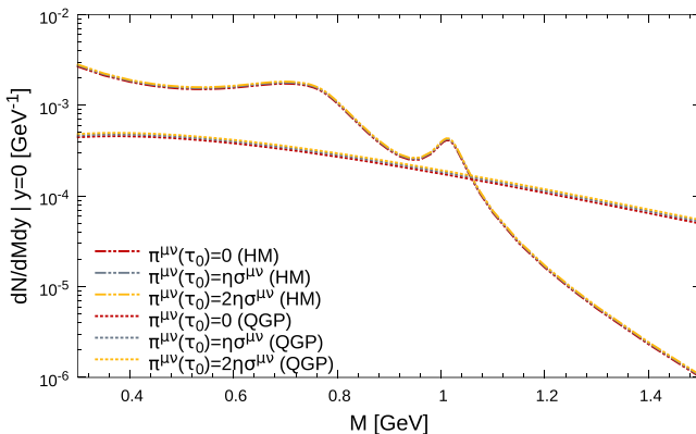
FIG. 13. Dilepton yield (left panel) and elliptic flow (right panel) as a function of invariant mass, for different values of initial \pi^{\mu\nu} .
