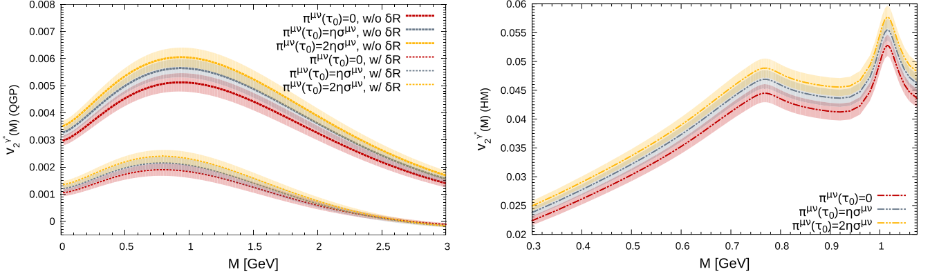
FIG. 14. Differential elliptic flow of dileptons emitted by the QGP (left panel) and emitted by the hadronic medium (HM) (see right panel) as a function of the dilepton invariant mass, for different values of initial shear stress tensor. Only the QGP dileptons are calculated with and without viscous correction \delta R to the rate, while the HM dileptons are calculated with the viscous correction.
