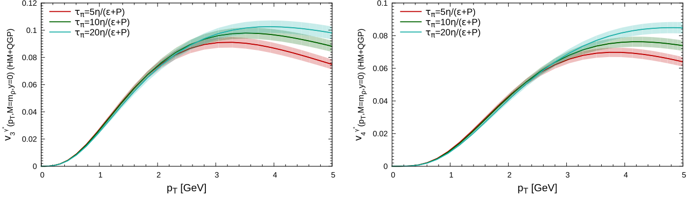
FIG. 6. Influence of \tau_\pi on higher flow harmonics of thermal dileptons at M = m_\rho : v_3(p_T) is in the left panel, and v_4(p_T) is in the right panel.
