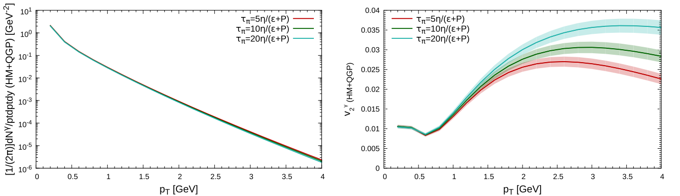
FIG. 3. Transverse momentum spectra (left panel) and differential elliptic flow (right panel) of thermal photons as a function of transverse momentum, for different values of shear relaxation time.
