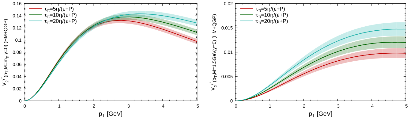
FIG. 5. Differential elliptic flow of thermal dileptons for M = m_\rho (left panel) and M = 1.5 GeV (right panel) as a function of transverse momentum, for different values of shear relaxation time.
