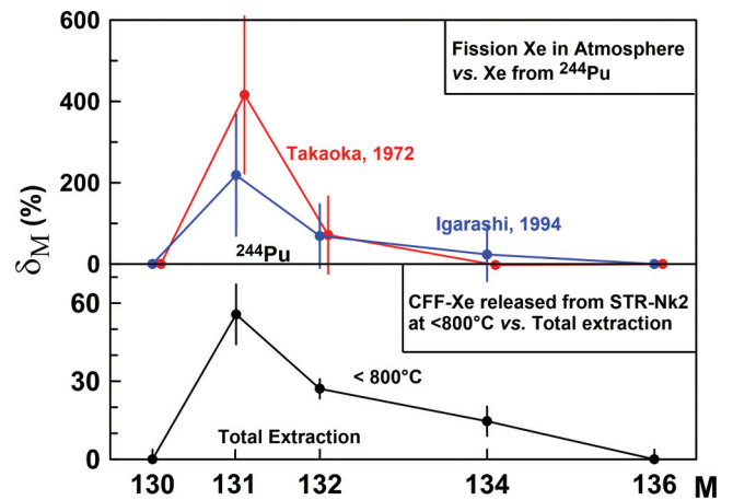
FIG. 9. Xe isotopic excesses in terrestrial atmosphere derived by Takaoka [38], Igarashi [43] \delta_M = 100\%[(^M\text{Xe}/^{136}\text{Xe})/(^M\text{Xe}/^{136}\text{Xe})_{\text{ref.}} - 1] (top) and CFF-Xe released at low temperature from acid-treated sample STR-Nk2 (bottom, this work). Terrestrial fission Xe is plotted relative to fission Xe from ^{244}\text{Pu} , and CFF-Xe from STR-Nk2 is shown relative to the total Xe composition in this sample. The similarity of the isotopic patterns suggests that terrestrial fission Xe is also formed by the CFF process.
