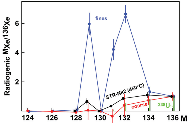
FIG. 6. Composition of fission Xe in Archean anorthosite from Fiskenaesset Complex in West Greenland. Xe in the coarse-grained fraction [32] is indistinguishable from fission Xe from ^{238}\text{U} (green bars). Xe from the fine-grained fraction of the same anorthosite block [7] has an anomalous pattern similar to the low-temperature Xe extraction of the acid-treated sample STR-Nk2 (this work). Errors are 1\sigma .
