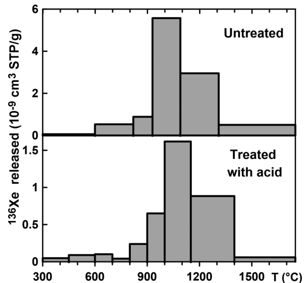
FIG. 1. Release of radiogenic ^{136}\text{Xe} from the original STR-Nk1 sample (top) and from the sample STR-Nk2 treated with \text{HNO}_3 for 3 h (bottom). About 2/3 of fission ^{136}\text{Xe} has been lost as a result of the treatment and the low-temperature Xe release peak became apparent in the leached STR-Nk2.
