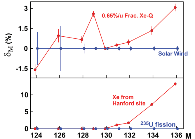
FIG. 11. Xe-Q can be modeled as fractionated by 6.5‰/u solar Xe [48] with \sim 3\% addition of ^{136}\text{Xe} , \sim 1.5\% of ^{134}\text{Xe} and <0.5\% of ^{132}\text{Xe} and ^{131}\text{Xe} (top). The isotopic structure of the required for this model addition matches the pattern of Xe found in the gas bubbles released from the Hanford site [35] (bottom). This model does not require any presolar Xe components.
