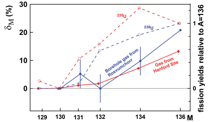
FIG. 7. Isotope excess \delta_M = 100\%[(^M\text{Xe}/^{136}\text{Xe})_{\text{sample}}/ (^M\text{Xe}/^{136}\text{Xe})_{\text{atm.}} - 1] in Xe released from boreholes in Rosvumchorr tunnel, Kola Peninsula [34], and in gas bubbles in groundwater from soil containing highly radioactive transuranic waste at DOE’s Hanford site [35] (solid lines). Fission yields of Xe isotopes from ^{235}\text{U} and ^{238}\text{U} (normalized to ^{136}\text{Xe} ) are shown for comparison (dashed lines). In both cases the ^{136}\text{Xe} excess is twice as large as the ^{134}\text{Xe} excess.
