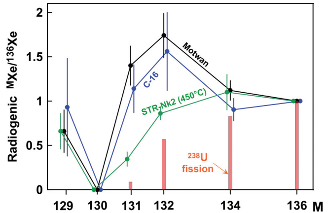
FIG. 5. Composition of fission Xe in CO 2 well gases from C-16, New Mexico [27], Motwan, Gujarat/India [31], and the lowest temperature extraction from the acid-treated sample STR-Nk2 (this work). Bars show fission yields from spontaneous fission of ^{238}\text{U} . All compositions are normalized to ^{136}\text{Xe} . Errors are 1\sigma .
