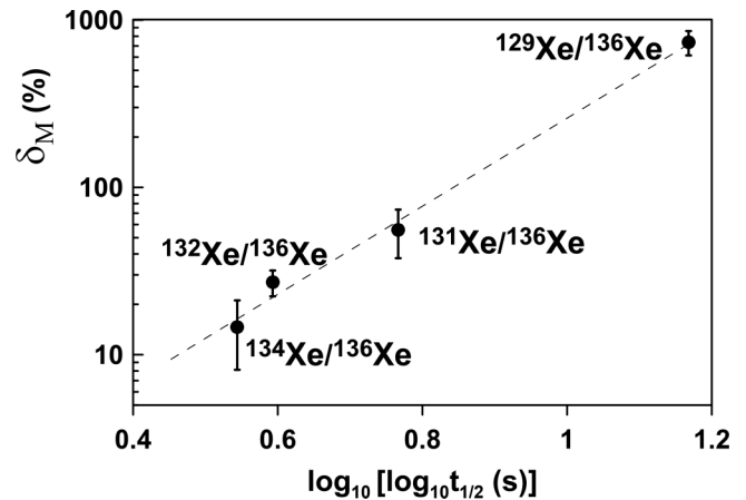
FIG. 4. Weighted average of Xe relative to ^{136}\text{Xe} isotopic excesses \delta_M = 100\% \times [(^M\text{Xe}/^{136}\text{Xe})_{\text{low T}} / (^M\text{Xe}/^{136}\text{Xe})_{\text{total}} - 1] at low ( < 800^\circ\text{C} ) extraction temperatures vs. half-lives of corresponding iodine isotopes, Xe precursors in fission chains. The correlation spans over 13 orders of magnitude in half-lives. Errors are 1\sigma .
