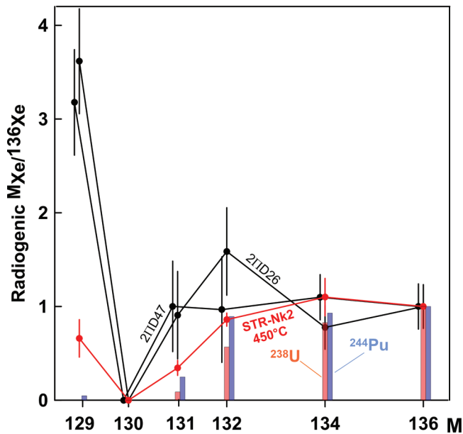
FIG. 8. Radiogenic Xe in precisely measured midocean ridge basalt glasses 2PID47 and 2PID26 [36] are not consistent with fission spectrum of ^{244}\text{Pu} (blue bars). This inconsistency is likely due to a CFF process which modified a ^{244}\text{Pu} fission yield. Similar modification is observed in low-temperature Xe extraction from acid-treated sample STR-Nk2 (this work) which is due to CFF modified yields of ^{238}\text{U} (red bars). Errors are 1\sigma .
