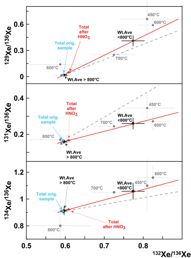
FIG. 2. Isotopic composition of Xe released from acid treated sample STR-Nk2 during stepwise pyrolysis. All temperature fractions tend to form linear arrays (solid lines) which differ from mass-fractionation lines (dashed). Stars show the compositions of Xe from spontaneous fission of ^{238}\text{U} and neutron-induced fission of ^{235}\text{U} . Composition of Xe lost due to the acid treatment is calculated from the difference between the original and treated samples.
