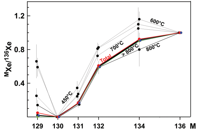
FIG. 3. Composition of fission Xe released from the acid-treated sample STR-Nk2 at different extraction temperatures. These compositions are normalized to ^{136}\text{Xe} . Errors are 1\sigma .
