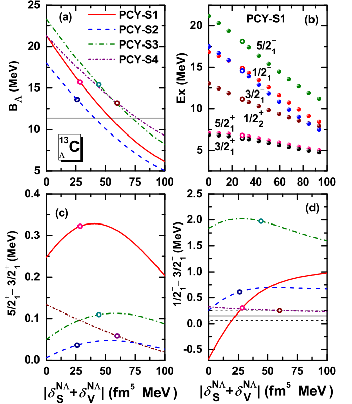
FIG. 4. (a) The \Lambda binding energy in ^{13}\text{C} as a function of |\delta_S^{N\Lambda} + \delta_V^{N\Lambda}| , while keeping the same values of \alpha_S^{N\Lambda} , \alpha_V^{N\Lambda} , \alpha_T^{N\Lambda} , and \delta_S^{N\Lambda}/\delta_V^{N\Lambda} as the original values for the PCY-S1, PCY-S2, PCY-S3, and PCY-S4 parameter sets. B_\Lambda with the original value of \delta_S^{N\Lambda} and \delta_V^{N\Lambda} is denoted by the open circles for each parameter set. The experimental value is denoted by the thin solid line. (b) The energy levels of the low-lying states as a function of |\delta_S^{N\Lambda} + \delta_V^{N\Lambda}| for the PCY-S1 parameter set. (c) and (d) The energy splitting between the 5/2_1^+ and 3/2_1^+ states and that between the 1/2_1^- and 3/2_1^- states, respectively, as a function of |\delta_S^{N\Lambda} + \delta_V^{N\Lambda}| .
