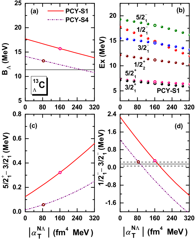
FIG. 5. Same as Fig. 4, but as a function of the tensor coupling strength |\alpha_T^{N\Lambda}| ( =-\alpha_T^{N\Lambda} ) for the PCY-S1 and PCY-S4 forces.
