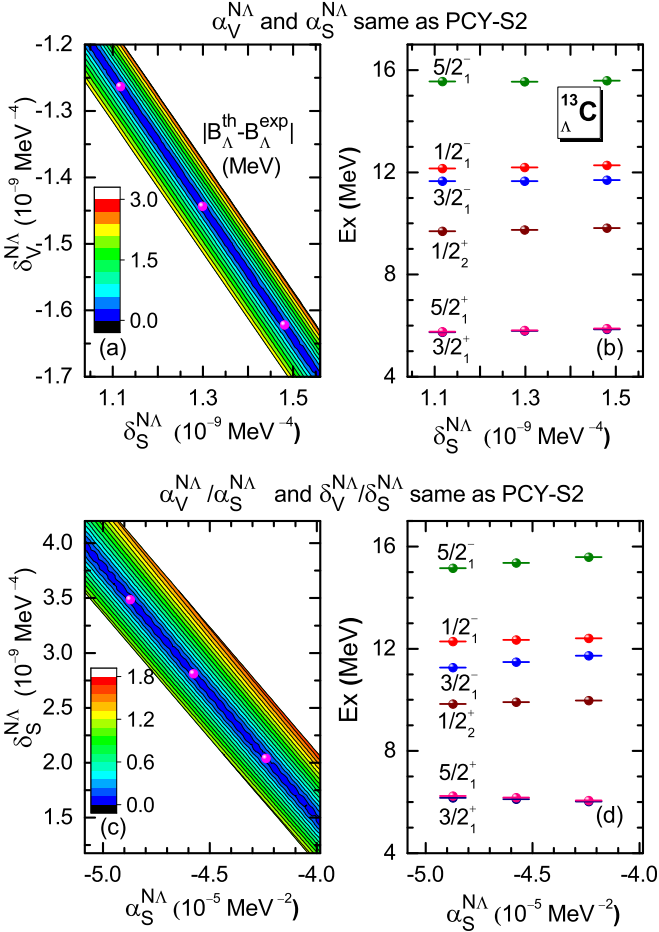
FIG. 3. (a) and (c) Contour plots for the absolute value of the difference between the theoretical and the experimental hyperon binding energies of the ^{13}\text{C} hypernucleus as a function of the coupling strength parameters (\delta_S^{N\Lambda}, \delta_V^{N\Lambda}) and (\alpha_S^{N\Lambda}, \alpha_V^{N\Lambda}) , respectively. In the former, \alpha_V^{N\Lambda} and \alpha_S^{N\Lambda} are fixed to the same values as in PCY-S2, while, in the latter, the value of \alpha_V^{N\Lambda} and \delta_V^{N\Lambda} is determined for each (\alpha_S^{N\Lambda}, \delta_S^{N\Lambda}) so as to keep the ratios \alpha_V^{N\Lambda}/\alpha_S^{N\Lambda} and \delta_V^{N\Lambda}/\delta_S^{N\Lambda} the same as those for PCY-S2. (b) and (d) Low-lying states in ^{13}\text{C} calculated with the strength parameters denoted by the dots in panels (a) and (c), respectively.
