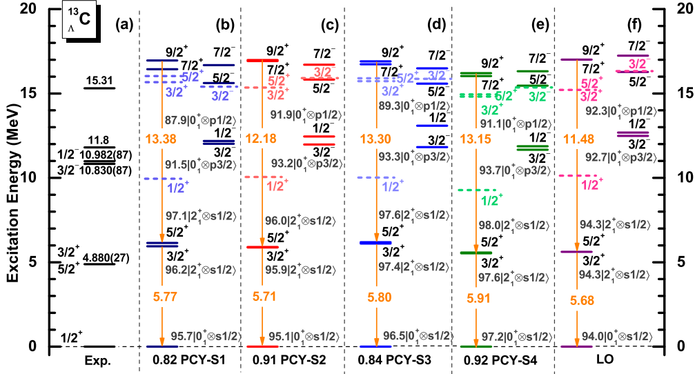
FIG. 2. The same as in Fig. 1, but with the scaled N\Lambda interaction, in which the scaling factor is determined for each parameter set to reproduce the empirical \Lambda binding energy of ^{13}_{\Lambda}\text{C} .
