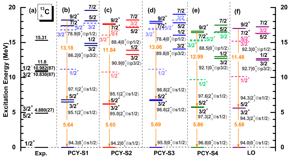
FIG. 1. The low-energy excitation spectra of {}^{13}_\Lambda\text{C} obtained with the microscopic particle-rotor model with (b) PCY-S1, (c) PCY-S2, (d) PCY-S3, and (e) PCY-S4. Part (f) shows the spectrum taken from Ref. [30], which was obtained by including only the leading-order (LO) N\Lambda interaction. The solid and the dashed lines represent the first and the second states for each spin-parity ( J^\pi ). The experimental data shown in (a) are taken from Refs. [1,38,39]. The numbers with the arrows indicate the B(E2) values for the 3/2^+_1 \rightarrow 1/2^+_1 and the 9/2^+_1 \rightarrow 5/2^+_1 transitions, given in units of e^2\text{fm}^4 . The dominant component of several hypernuclear states, together with its weight (in percent), is also given.
