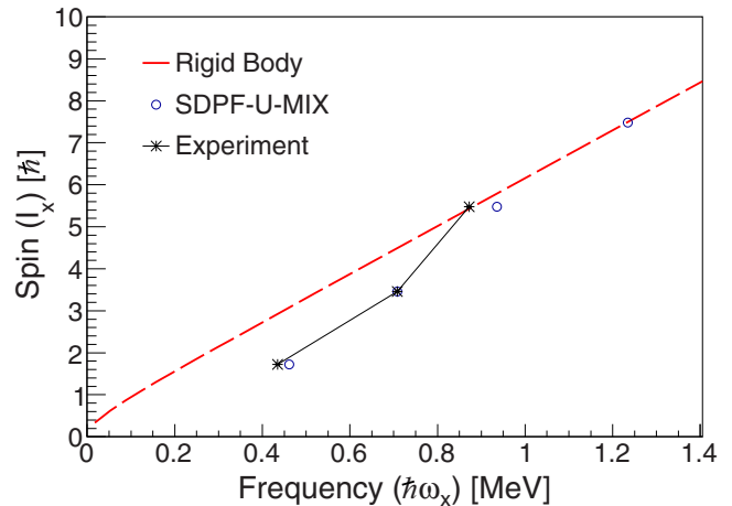
FIG. 2. Spin ( I_x ) versus angular frequency ( \hbar\omega_x ) for the ground-state band. Experimental points are plotted as asterisks (connected by the solid black line) while the results of large-scale shell-model calculations using the SDPF-U-MIX effective interaction are shown in blue open circles. The red dashed line shows the rigid-rotor limit for this nucleus assuming an axially symmetric prolate shape with a deformation \epsilon_2 = 0.4 .
