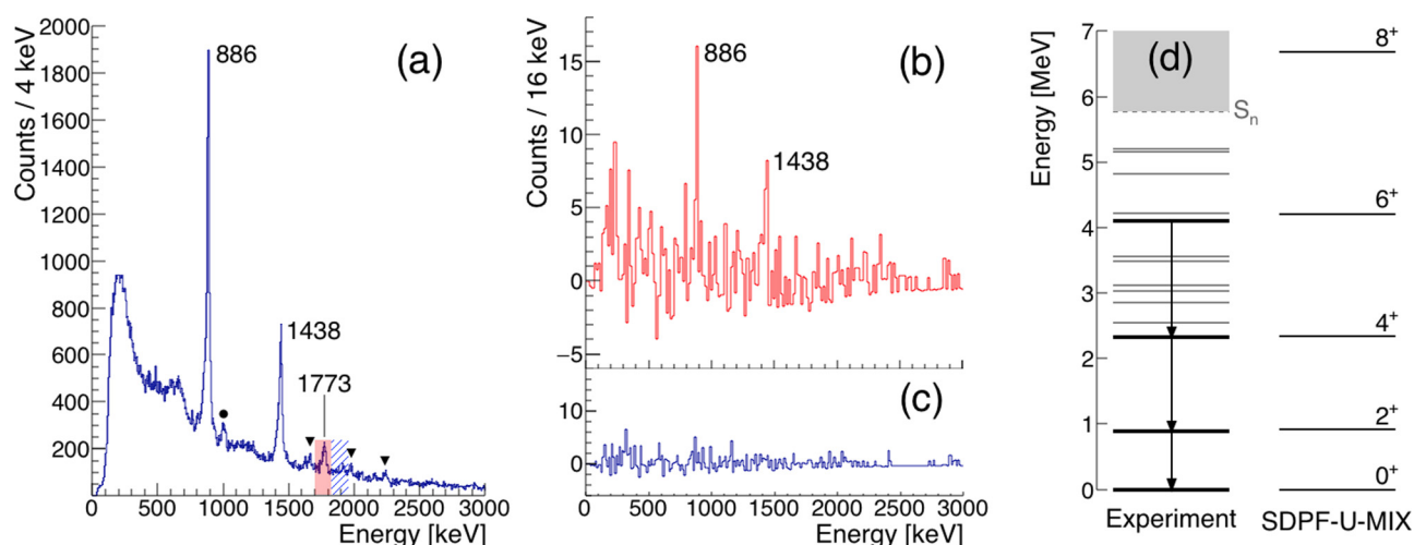
FIG. 1. (a) Prompt \gamma -ray spectrum detected with GRETINA in coincidence with ^{32}\text{Mg} heavy recoils following secondary fragmentation of a ^{46}\text{Ar} beam at the target position of the S800; other previously observed transitions are marked by inverted triangles (see text). (b) Spectrum of \gamma rays in coincidence with the 1773 keV transition (red shaded region) obtained from a background-subtracted \gamma - \gamma correlation matrix [see Eq. (3) in Ref. [13]]. (c) Similar to panel (b) but now in coincidence with an energy region (“background”) immediately above the proposed 1773 keV \gamma ray (blue hashed region). The 886 and 1438 keV transitions are visible in the 1773 keV gated spectrum (panel b), but not in the “background” gated spectrum [panel (c)]. (d) Experimental excitation energies for the known levels in ^{32}\text{Mg} [8,14,15], including the ground-state rotational band states observed in the present work (bolded lines) and shell-model excitation energies for the lowest-lying (yrast) rotational states.
