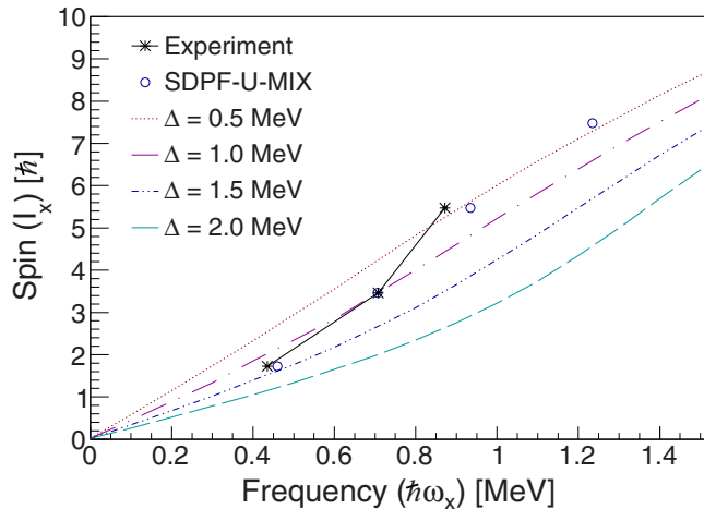
FIG. 3. Spin ( I_x ) vs angular frequency ( \hbar\omega_x ) for the ground-state band; experimental points are plotted as asterisks and connected by the solid black line, while the open blue circles are the results of shell-model calculations. The colored curves correspond to the results of CSM calculations performed with different values for the pairing gap, \Delta_{n,p} ranging from 2.0 to 0.5 MeV.
